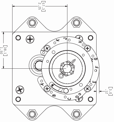
BRACKET CUT-OUT DIMENSIONS SCALE 1:2
