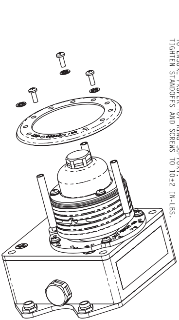
Figure A-11. GSM 85A Servo Gearbox For 1/16" Cable (Sheet 2 of 2)
