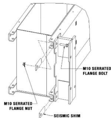
I-BEAM HARDWARE INSTALLATION Figure 7
