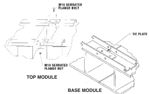
TIE PLATE ASSEMBLIES - HORIZONTAL STACKS Figure 18
