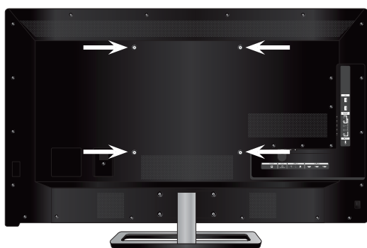
WALL-MOUNT SCREW LOCATIONS
