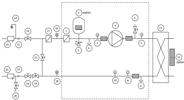
Typical hydraulic circuit diagram
