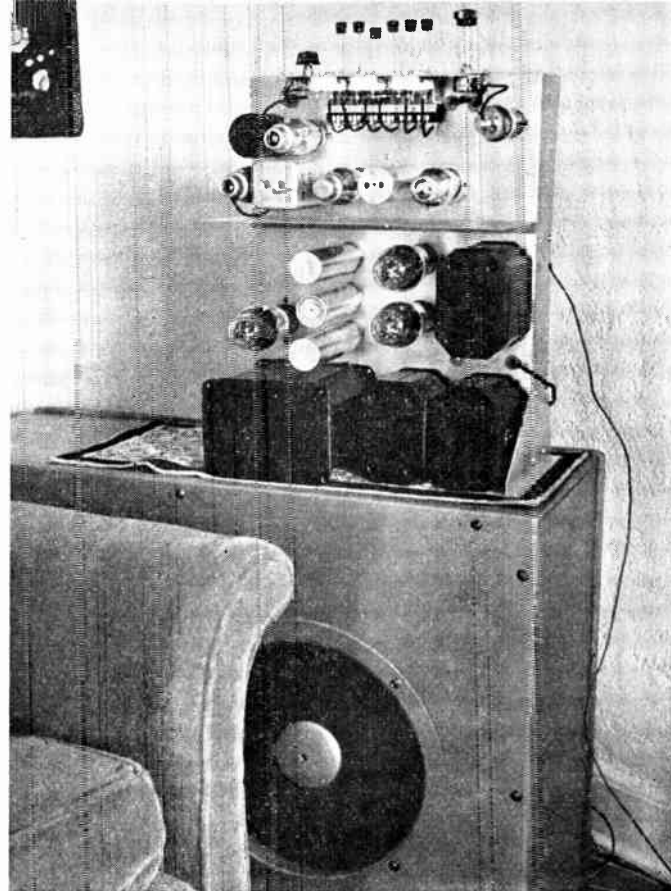
The AWR Automatic receiver resting atop the Jensen Peri-dynamic reproducer which is part of the equipment. Note that chassis assumes a vertical position, with push-button switch at top.
