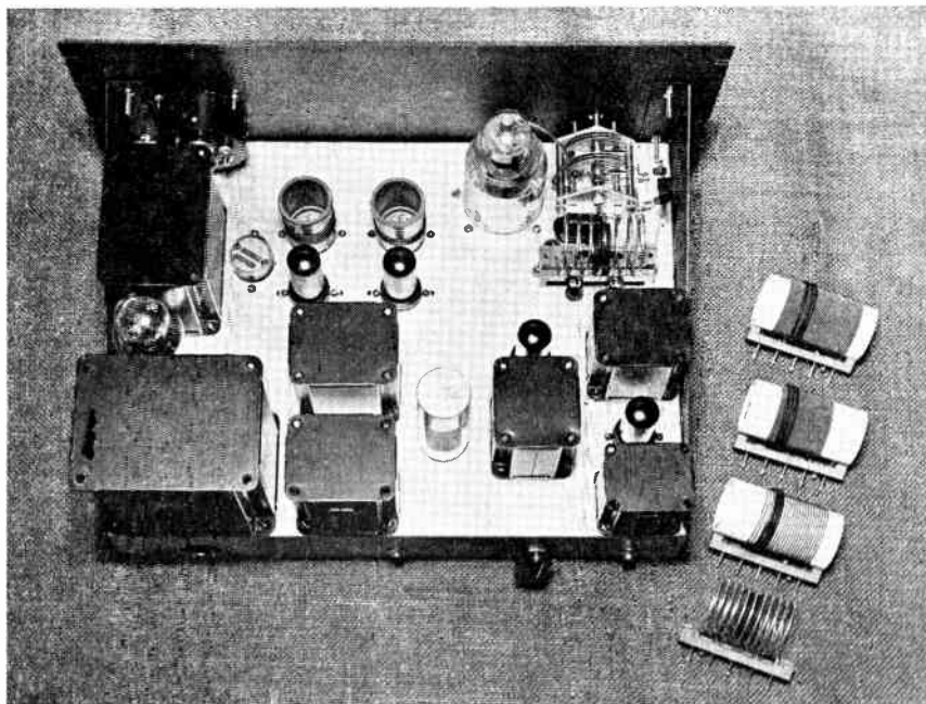
Top view of the transmitter chassis, showing location of components. Compare this with the chassis layout drawing on page 16. The 20, 40, 80 and 160-meter coils for the final tank circuit are also shown.
