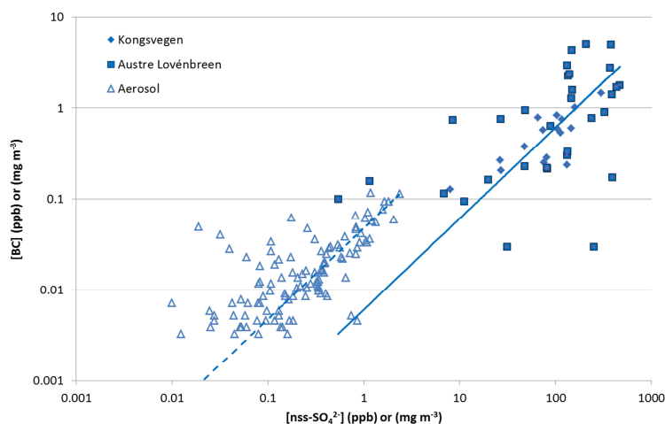
Fig. 7: BC vs. nss-sulfate concentrations in snow pit KV (filled diamonds) and AL (filled squares), and in aerosols (open triangles). The lines calculated by linear regression are forced through the origin and separated for the aerosol and the snow samples. BC in the snow pits corresponds to rBC, while the BC in aerosols corresponds to eBC.
