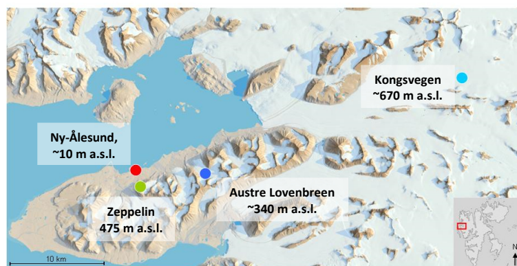
Fig. 1: 3D map of the Kongsfjord area with Ny-Ålesund (red), Zeppelin Station (green) and the locations of the snow pits on the Kongsvegen (light blue) and the Austre Lovénbreen glaciers (dark blue) indicated (©Norwegian Polar Institute).
