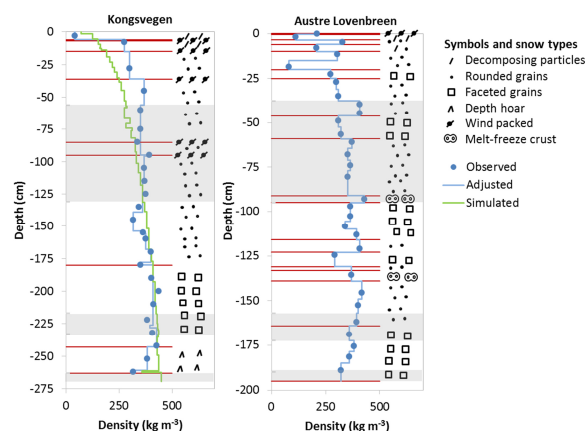
Fig. 2: Snow stratigraphy observed in the snow pits KV (left) and AL (right). Note the different depth scales. Snow types are indicated on the right side using the classification recommended by Fierz et al. (2009) with layers separated by horizontal red lines. Blue circles indicate observed snow densities, vertical blue lines correspond to snow densities adjusted to observed and sampled layers. The green line shows snow densities simulated with the Crocus model for snow pit KV. The alternating shaded and non-shaded areas correspond from the top to the months March to October.
