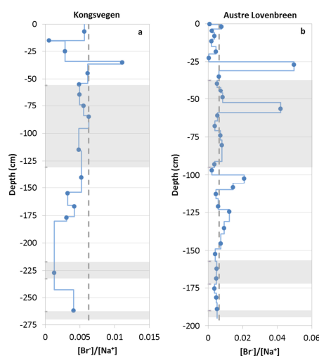
Fig. 8: Bromide-to-sodium ratio in the snow pits KV (left) and AL (right). Blue circles indicate observed ratios; blue lines correspond to ratios adjusted to the observed stratigraphy. The alternating non-shaded areas correspond to the months November, December, January, February, and March (from the bottom). The vertical dashed grey lines indicate the standard sea water ratio.
