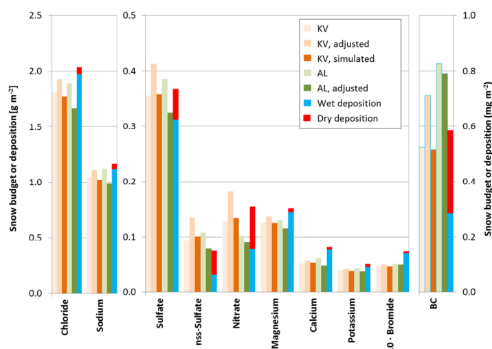
Fig. 4: Snow budgets of sea salt components, nss-sulfate, nitrate and bromide (left and middle) and BC (right) for the snow pits KV (Kongsvegen, brown) and AL (Austre Lovénbreen, green) for October 2011 to March 2012 according to different calculation methods: simple budgets from average concentrations and total SWE (light colors), adjusted budgets using co-located concentration and density profiles (middle colors), and simulated budgets for KV using interpolated concentration and simulated density profiles (dark colors). Also shown is the total deposition as the sum of observed wet deposition at Ny-Ålesund (blue) and estimated dry particle deposition (red). For bromide the wet deposition was estimated from the standard sea water ratio and all numbers are multiplied by ten. For BC the snow budgets correspond to rBC, while the wet deposition was estimated for the KV snow pit. The BC deposition corresponds to eBC. See text for further details.
