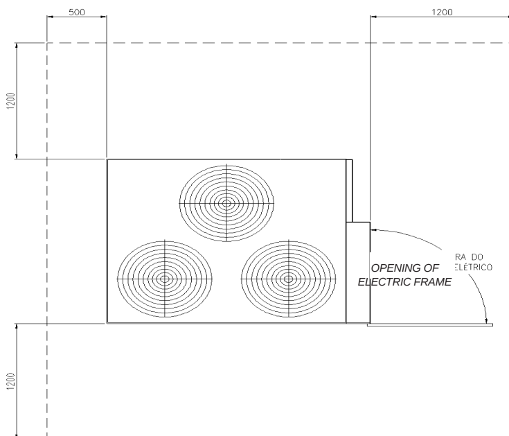
Fig. 14 - Maintenance and air circulation clearances
