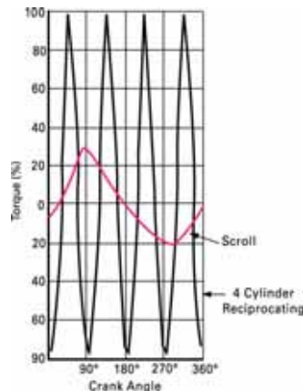
Fig. 38 - Comparison Scroll x Reciprocal
