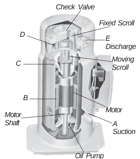
Fig. 40 - Compressor Scroll
