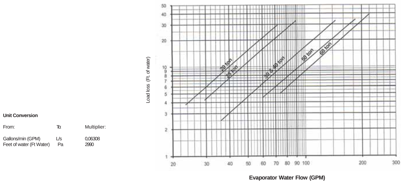
Fig. 03 - Evaporator Pressure Drop - 70 to 90 Tons Units
