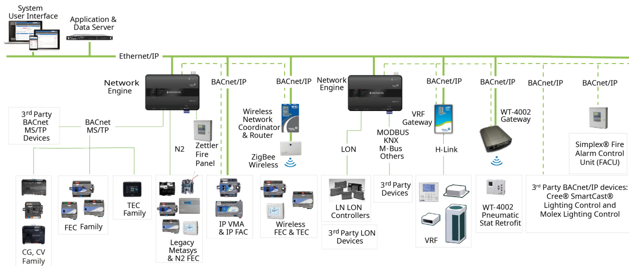
Figure 2: Metasys system architecture
