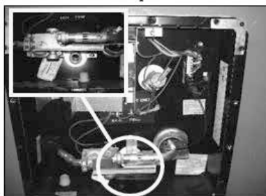
Fig 1: Water Heater Drain Plug
