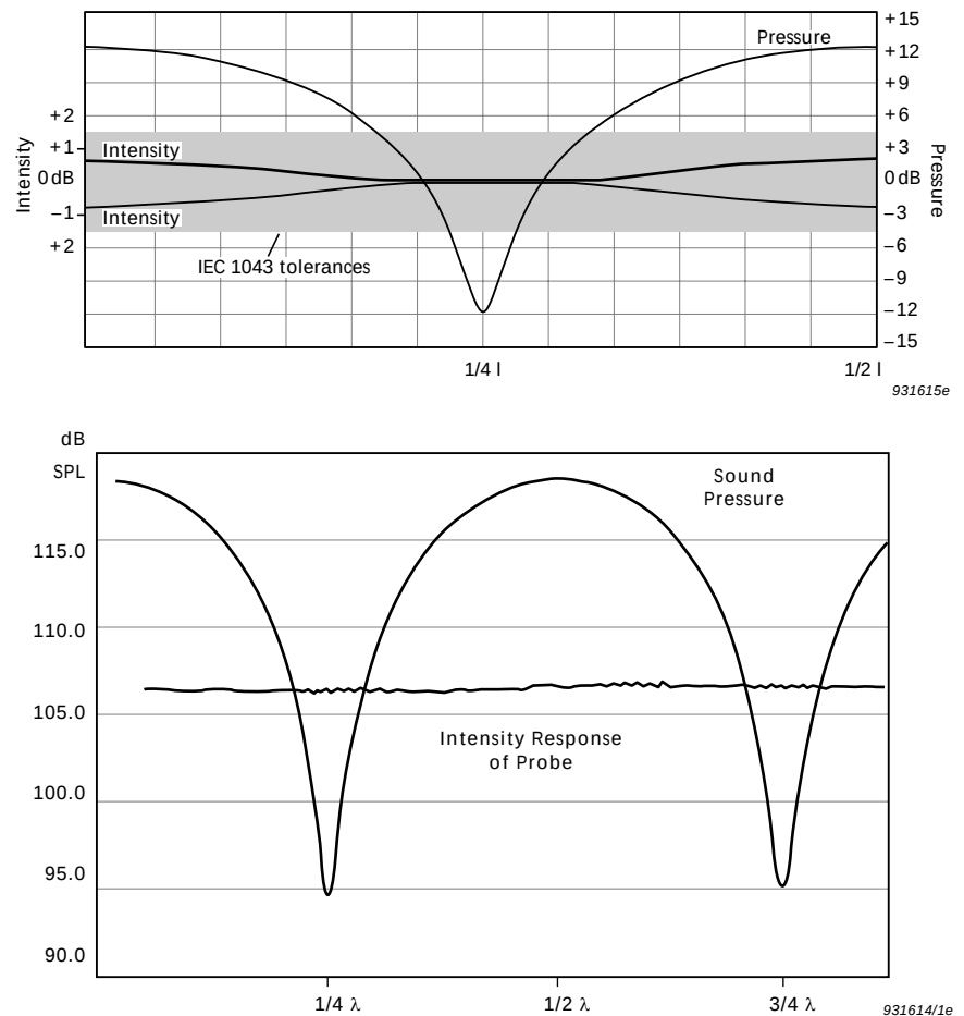
Fig.6 The upper graph illustrates the calculated intensity response limits relative to a standing wave, for a probe consisting of Sound Intensity Microphone Pair Type 4197 and Dual Preamplifier Type 2683. The calculation is valid for the maximum phase deviation specified for the microphone pair and preamplifier configuration and for field conditions according to IEC 1043 (50 mm spacer at 125 Hz and a standing wave ratio of 24 dB). In practice the intensity response of the probe is significantly better as shown in the lower graph
