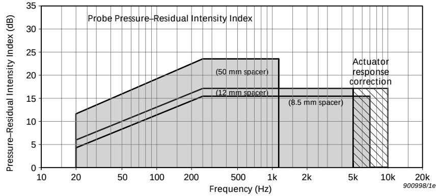
Fig.5 Specified frequency and Pressure-Residual Intensity Index ranges for the probe (Pressure-Residual Intensity Index = Pressure Level – Intensity Level (measured in a closed coupler)). Frequency axis is in 1/3 -octave centre frequencies
