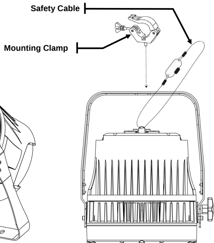
Overhead Mounting
