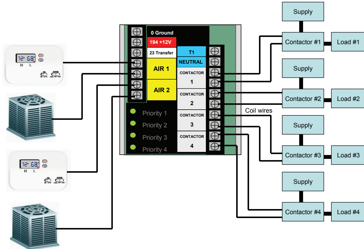
Load Shed Module Connections
