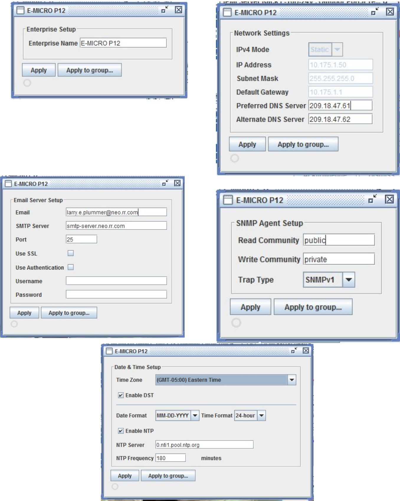
Figure 37- E-MICRO-T(RHP) and -1W Configuration Options
