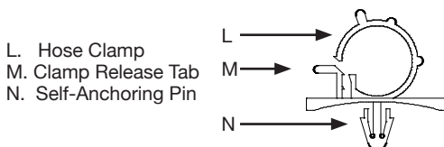
(Fig. 3) Leader Hose Bracket (N/A 32534)
