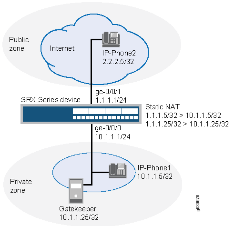
Figure 22: NAT with the H.323 ALG—Outgoing Calls
