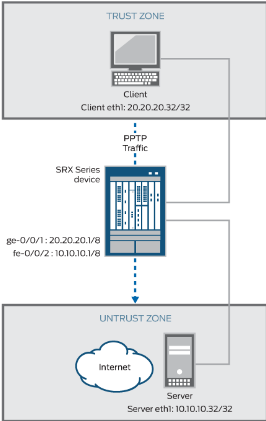
Figure 4: PPTP ALG Topology
