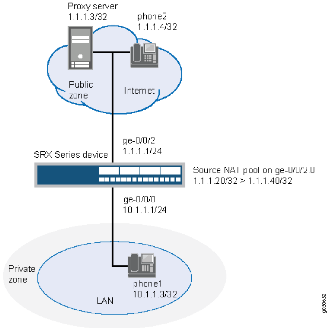
Figure 32: Source NAT Pool for Incoming SIP Calls
