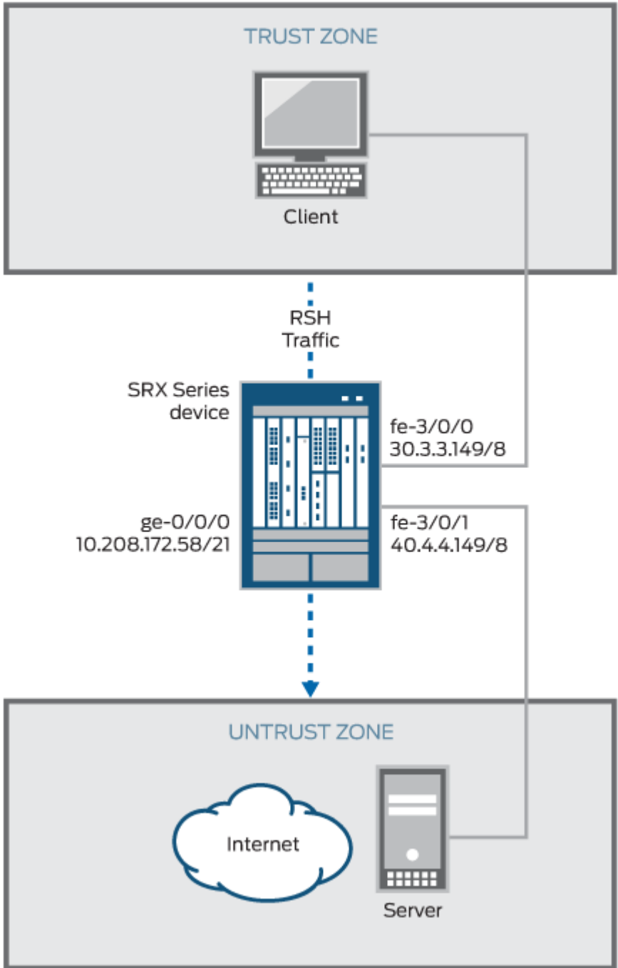
Figure 5: RSH ALG Topology
