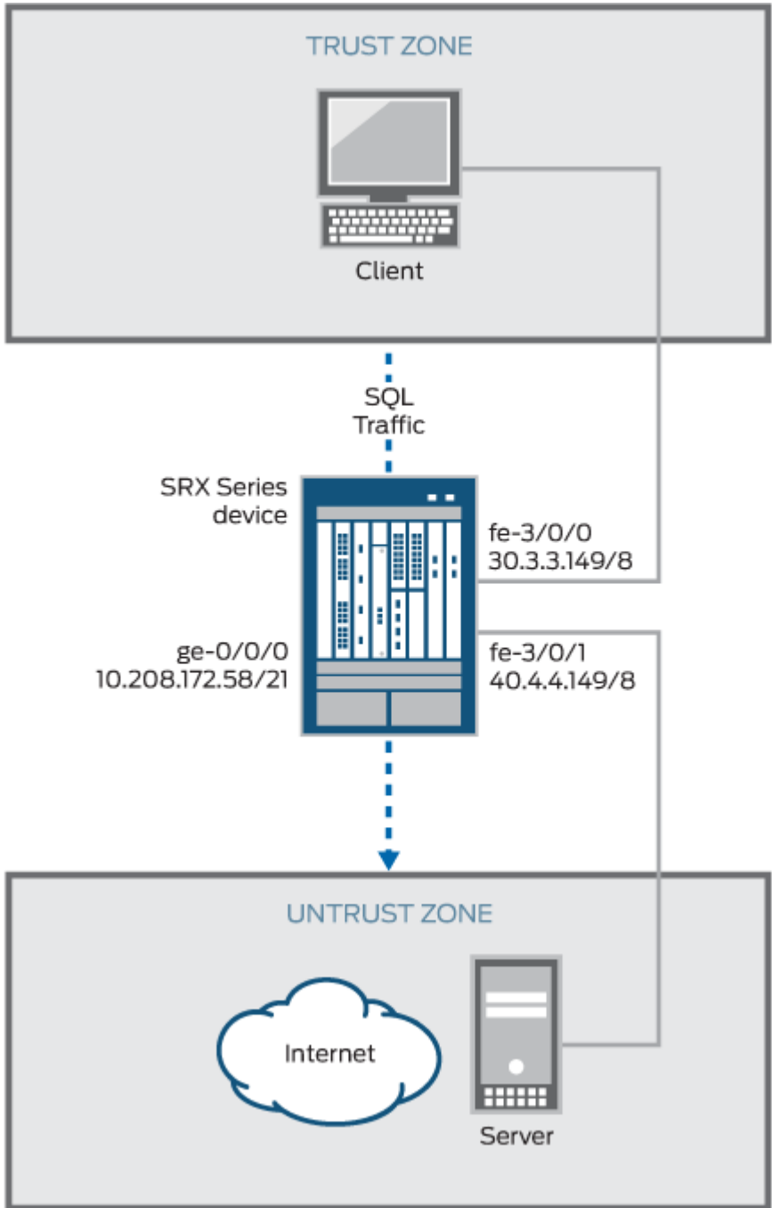
Figure 9: SQLNET ALG Topology
