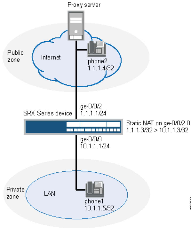
Figure 33: Static NAT for Incoming Calls
