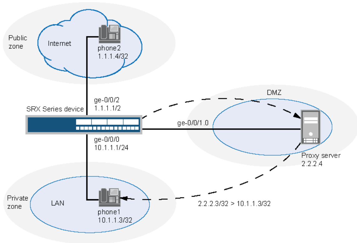
Figure 35: Three-Zone SIP Configuration with Proxy in the DMZ
