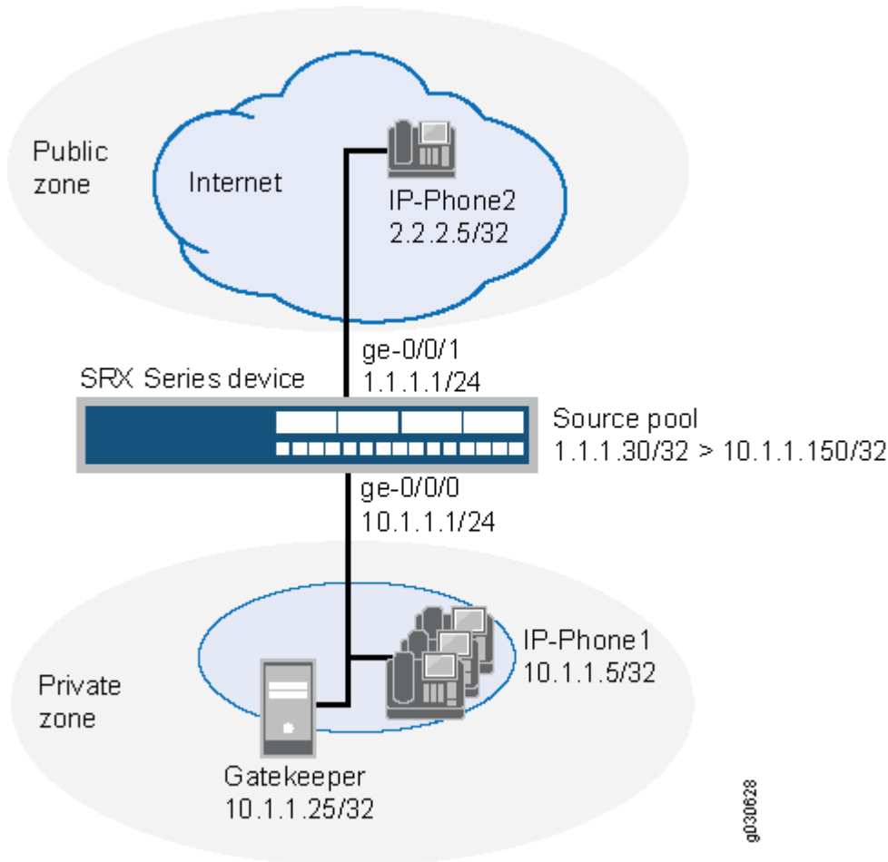
Figure 21: NAT with the H.323 ALG—Incoming Calls
