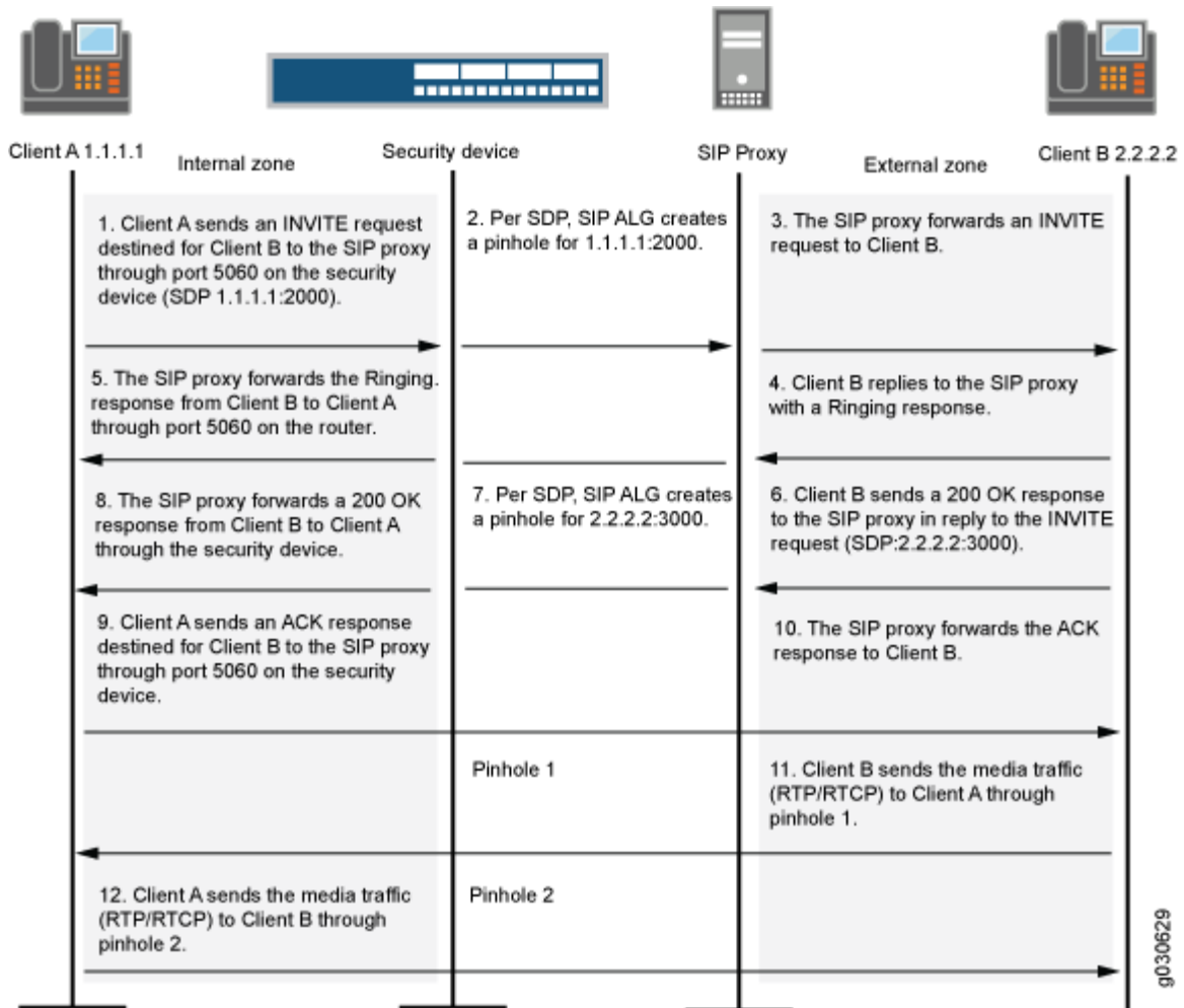
Figure 27: SIP ALG Call Setup
