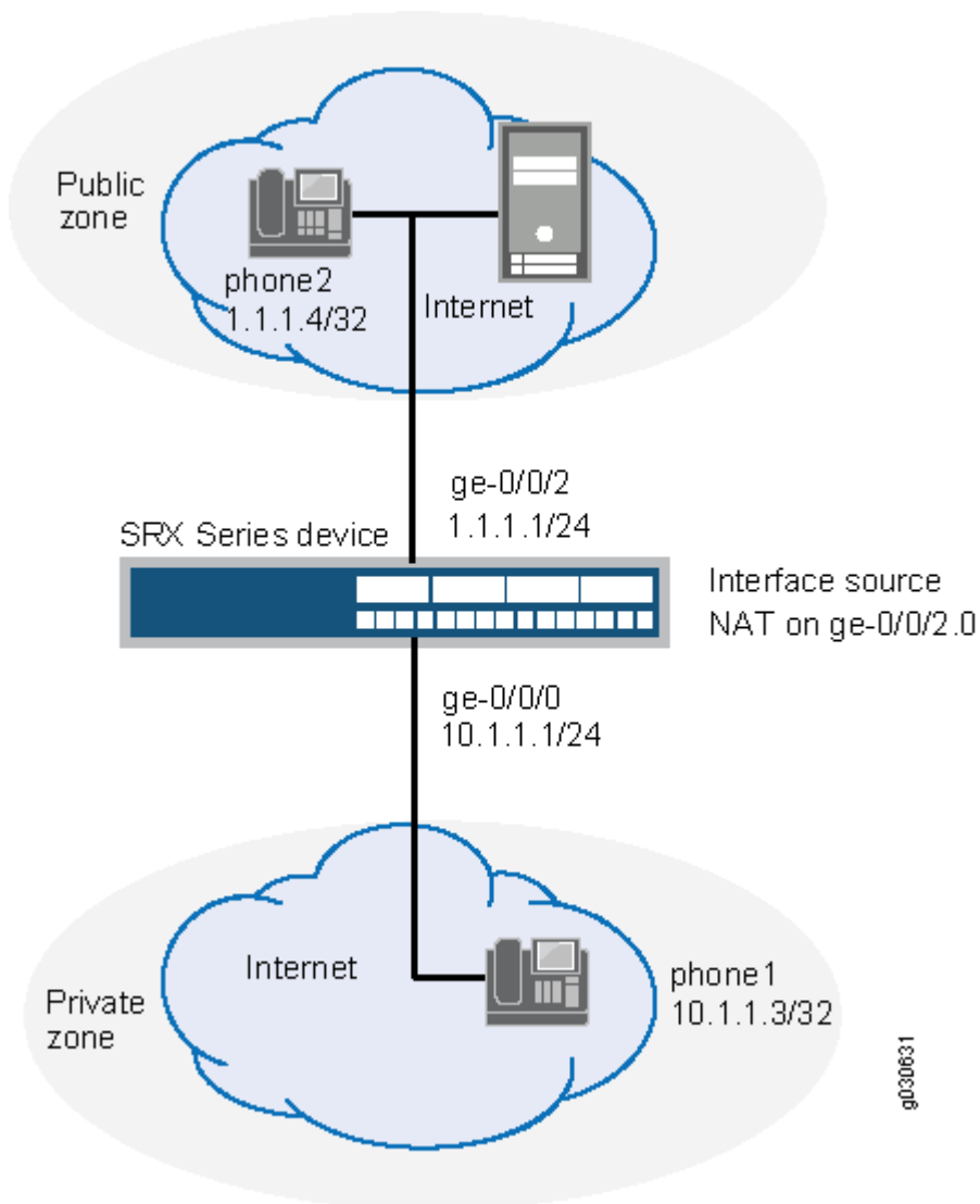
Figure 31: Source NAT for Incoming SIP Calls
