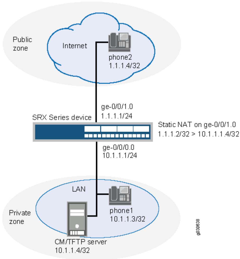
Figure 26: Call Manager or TFTP Server in the Private Zone
