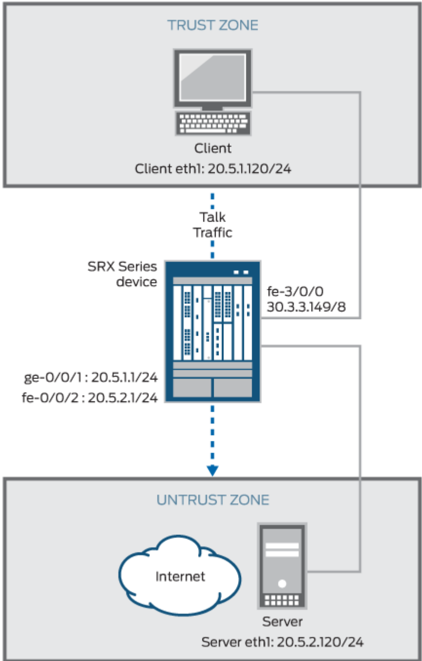
Figure 10: TALK ALG Topology
