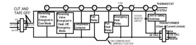
Figure 4. Typical wiring diagram for two transformer heat pump systems with NO safety circuits
