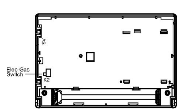
Figure 1. Electric/Gas Switch (Fan Option)
