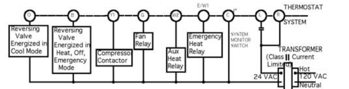
Figure 3. Typical wiring diagram for single transformer heat pump systems
