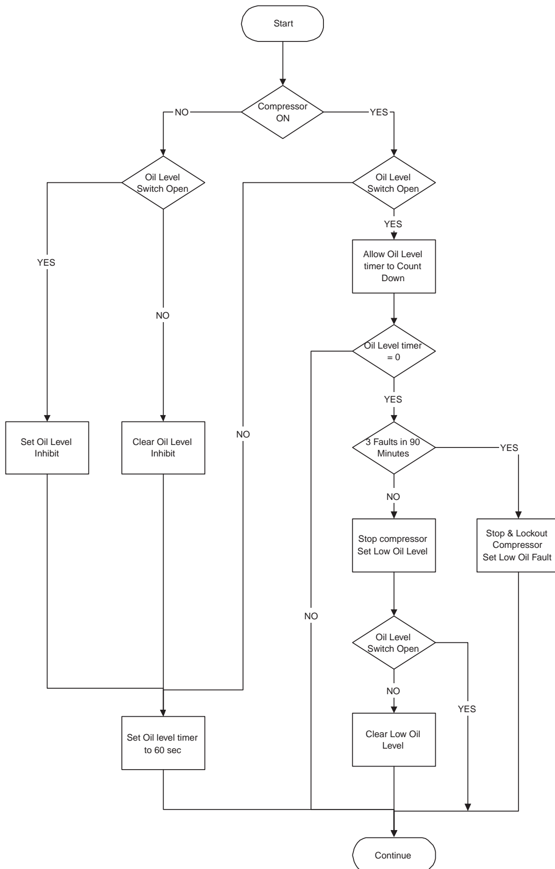
Figure 8 - Oil Level Safety Flow Chart
