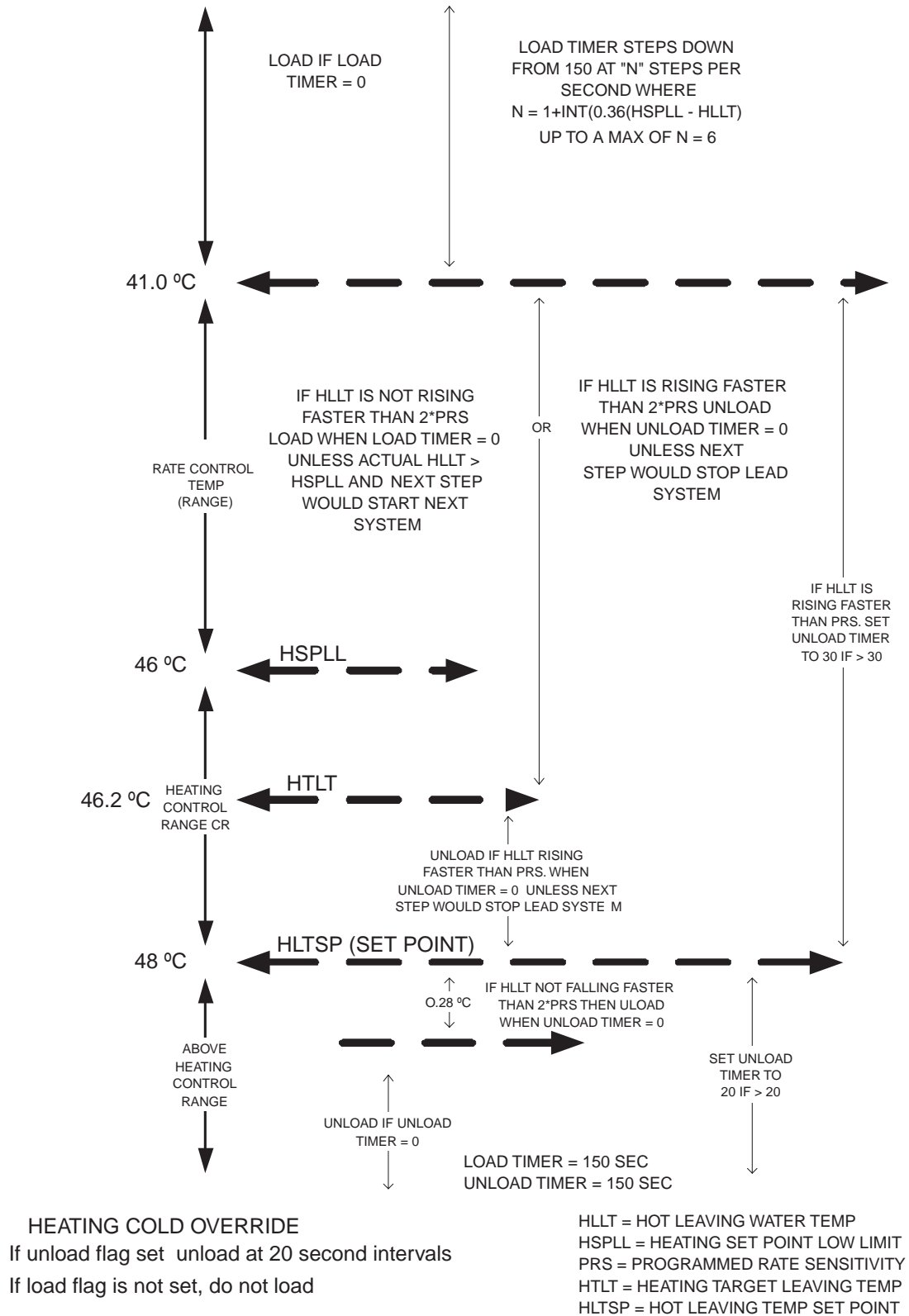
Figure 12 - Heatpump Mode Leaving Water Control
