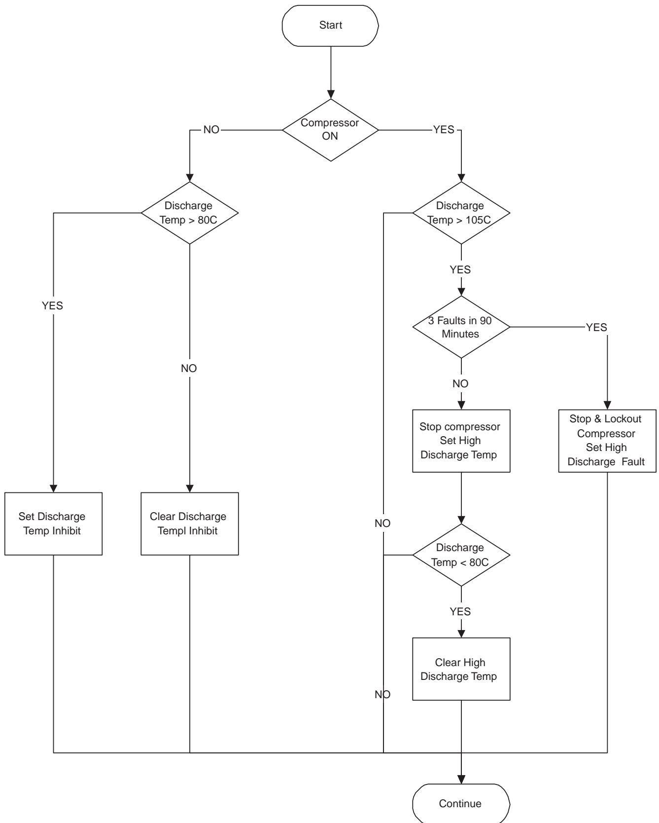
Figure 9 - High Discharge Temperature Safety Flow Chart
