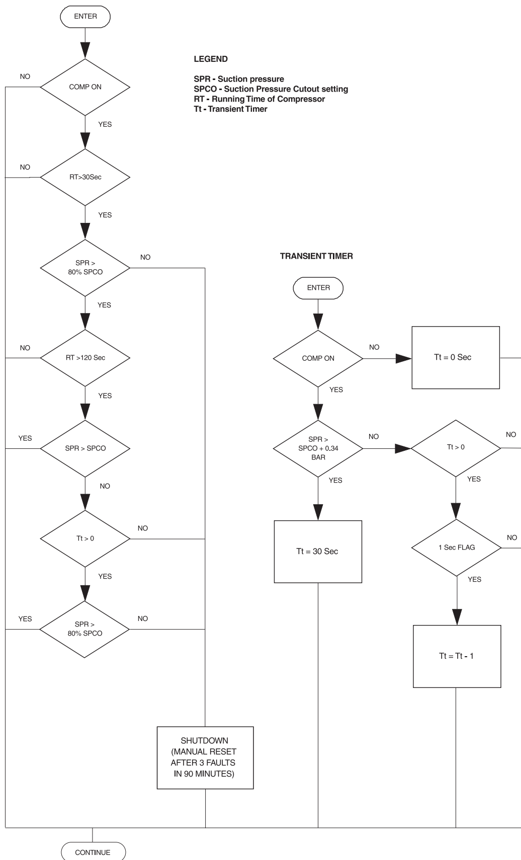
Figure 2 - Suction Pressure Safety Flow Chart
