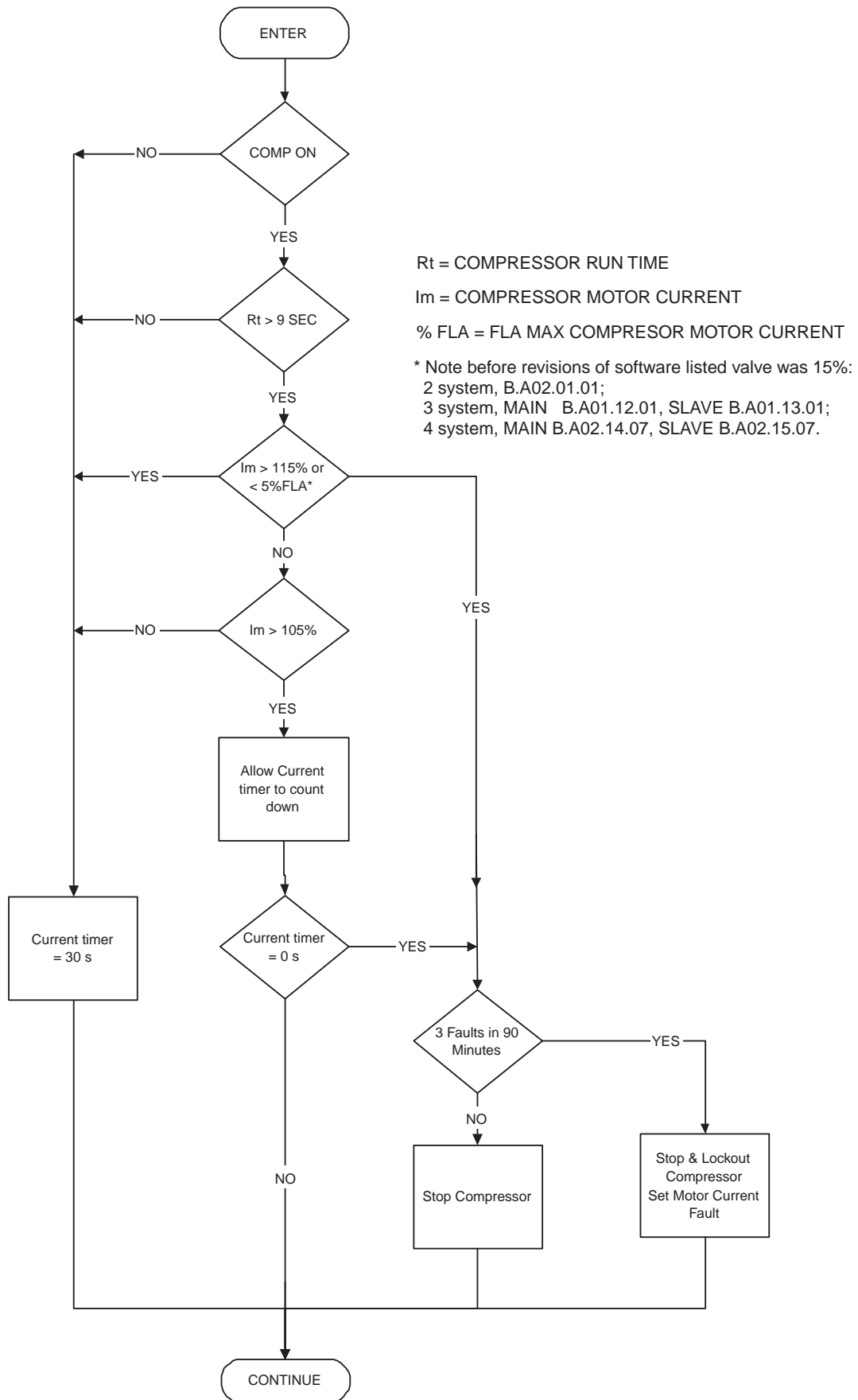
Figure 3 - Electronic Overload Flow Chart
