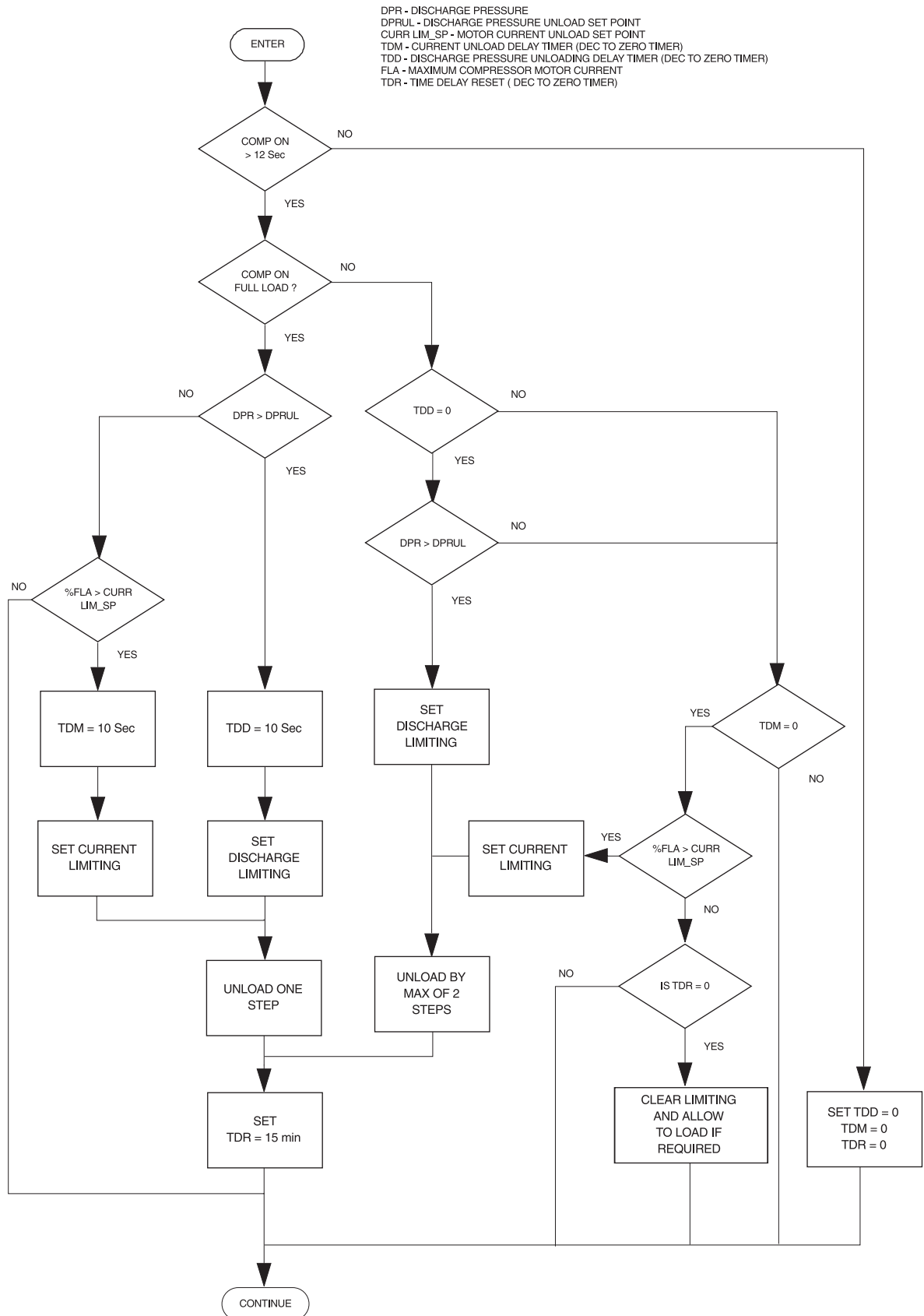
Figure 5 - Discharge/Current Unloading Flow Chart
