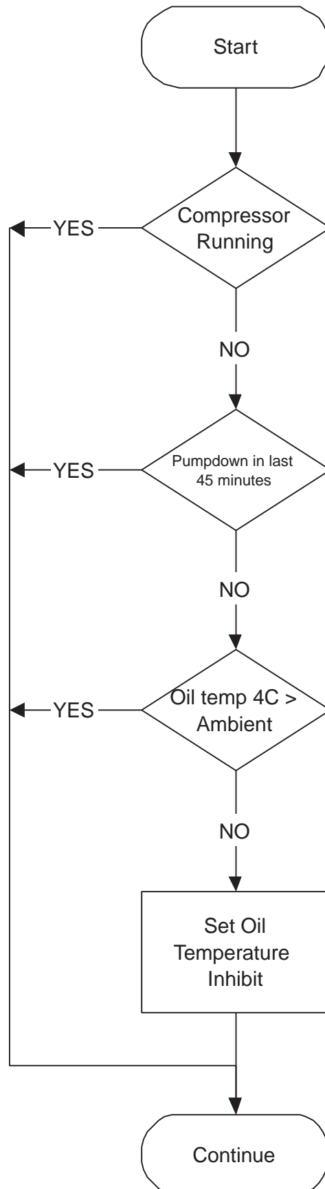
Figure 7 - Oil Temperature Inhibit Flow Chart
