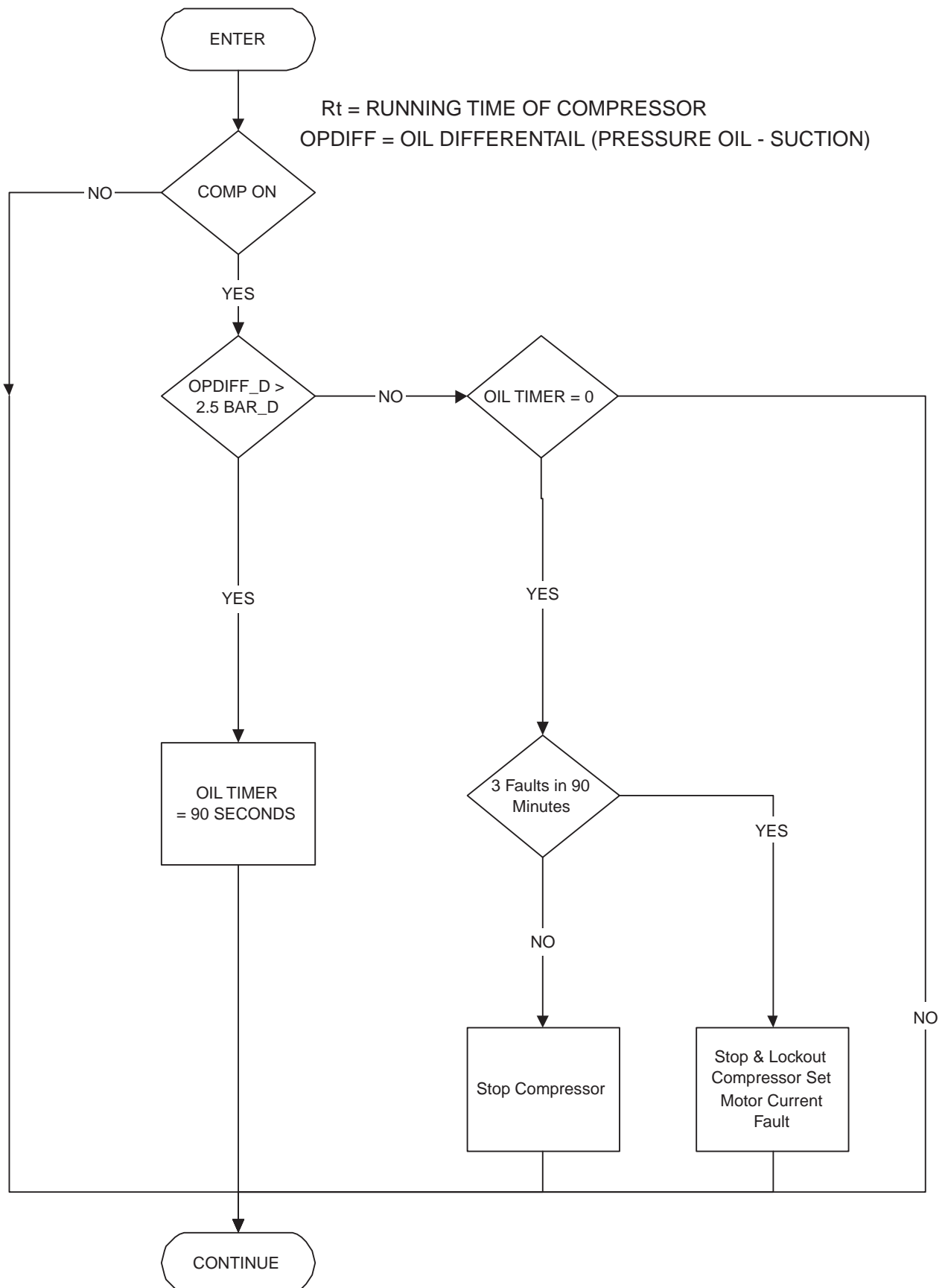
Figure 4 - Oil Pressure Safety Flow Chart
