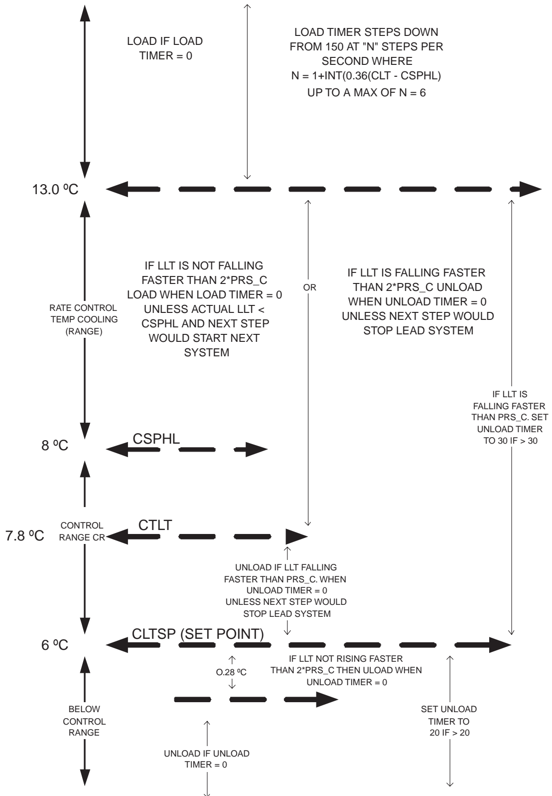
Figure 1 - Leaving Water Control
