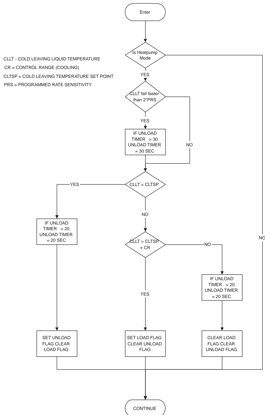
Figure 13 - Heating Cold Override Routine
