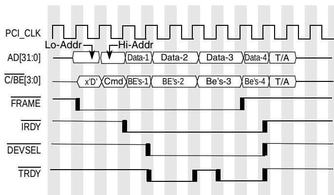
Figure 7-11. DAC Burst Write Example
