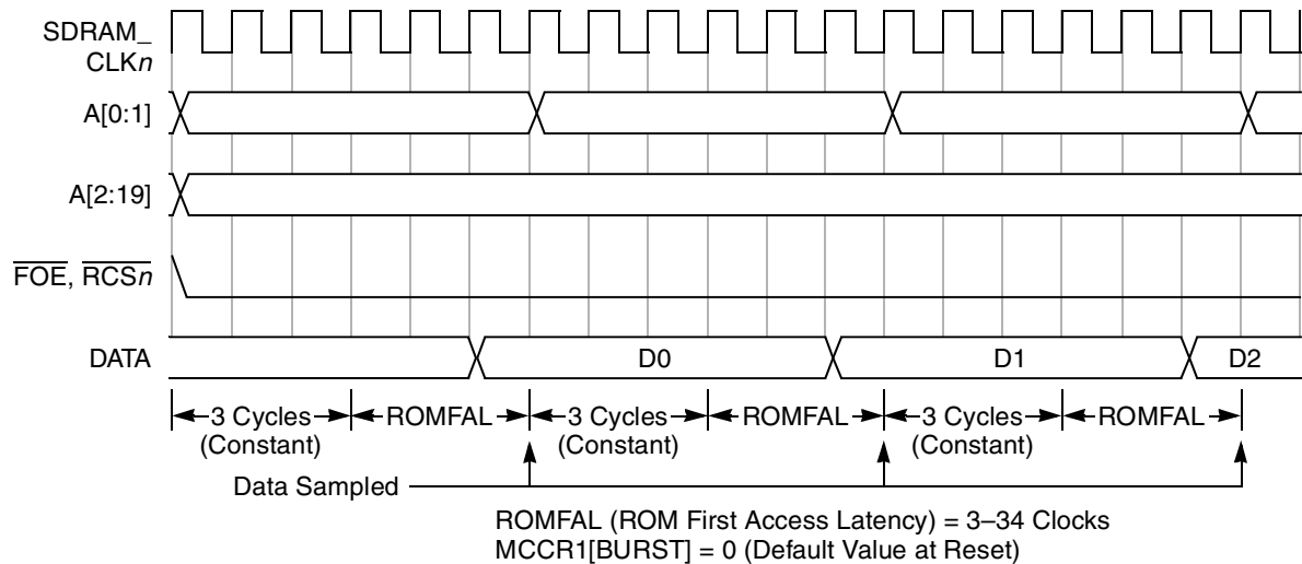
Figure 6-38. Read Access Timing for Non-Burst ROM/Flash Devices—64-/32-Bit (Wide) Data Path
