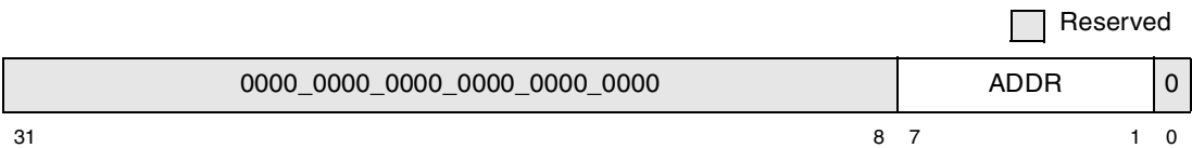
Figure 10-3. I 2 C Address Register (I2CADR)
