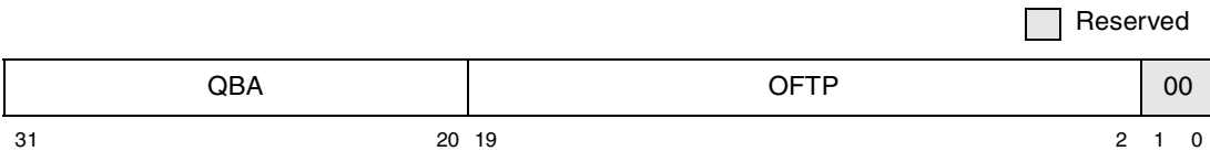
Figure 9-16. Outbound Free_FIFO Tail Pointer Register (OFTPR)
