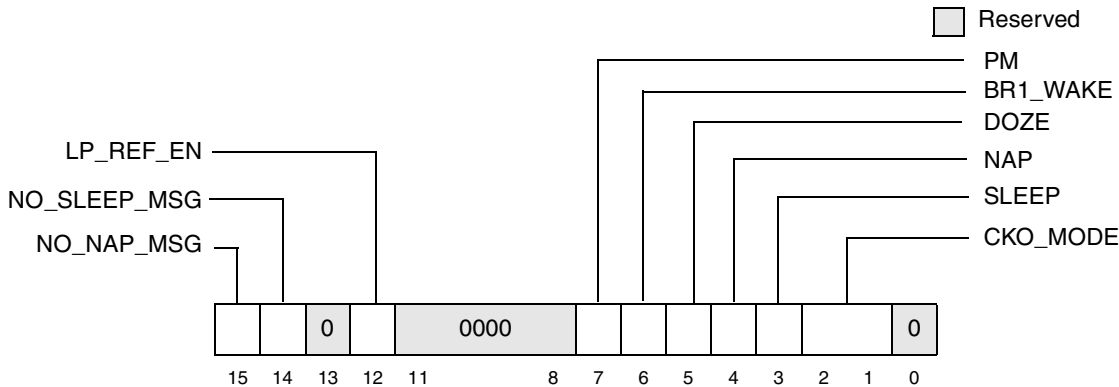
Figure 4-5. Power Management Configuration Register 1 (PMCR1)—0x70
