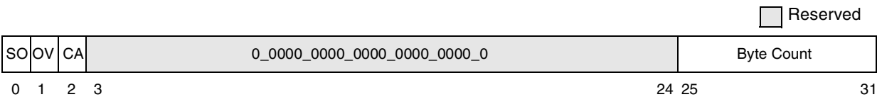
Figure D-6. XER Register
