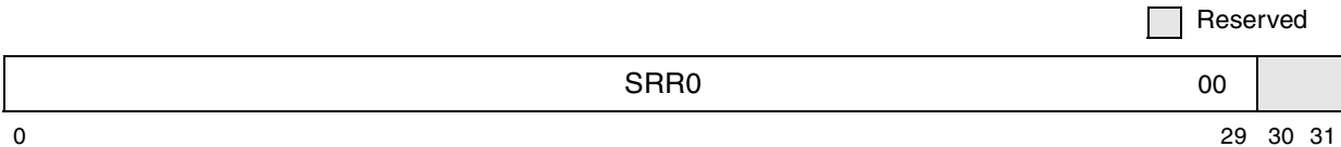
Figure D-18. Machine Status Save/Restore Register 0 (SRR0)
