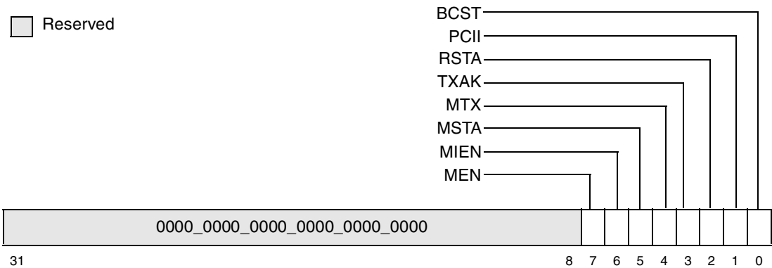
Figure 10-5. I 2 C Control Register (I2CCR)
