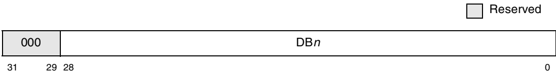
Figure 9-3. Outbound Doorbell Register (ODBR)
