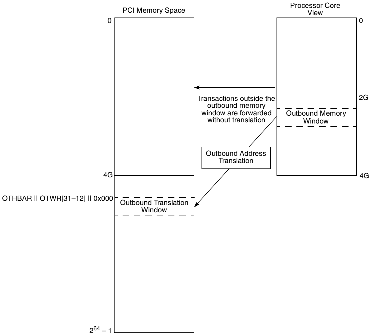
Figure 3-10. Outbound Dual Address Cycles, OTHBAR ≠ 0
