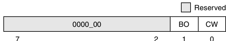
Figure 12-15. Alternate Function Register (UAFR)
