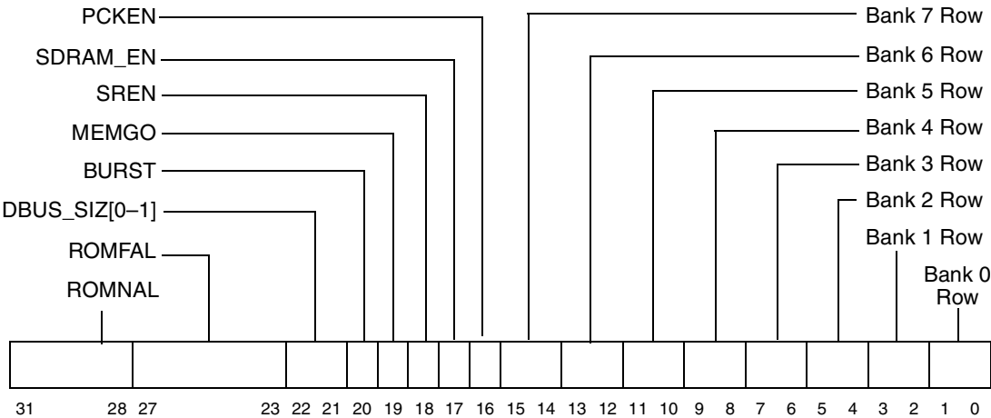
Figure 4-34. Memory Control Configuration Register 1 (MCCR1)—0xF0
