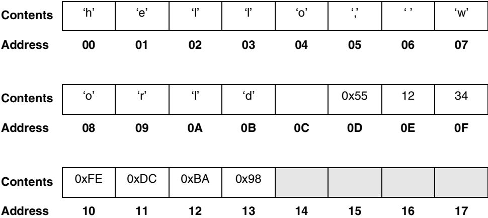
Figure A-2. Big-Endian Memory Image in Local Memory
