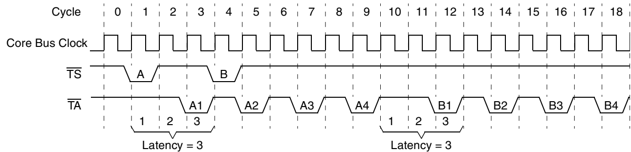
Figure 16-4. Processor Latency
