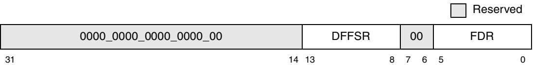
Figure 10-4. I 2 C Frequency Divider Register (I2CFDR)
