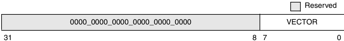
Figure 11-19. Processor Interrupt Acknowledge Register (IACK)
