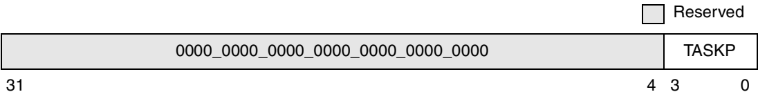
Figure 11-18. Processor Current Task Priority Register (PCTPR)
