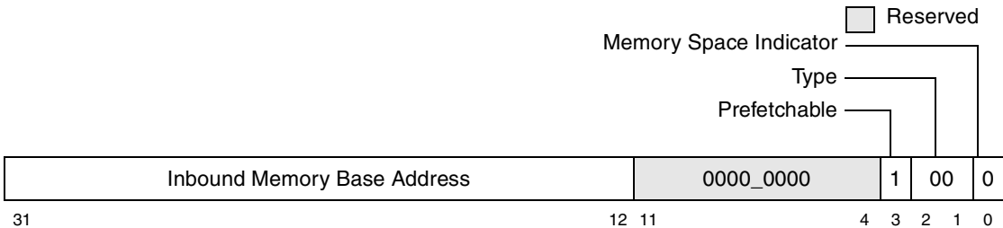
Figure 3-11. Local Memory Base Address Registers (LMBAR n )—Offset 0x10 and 0x18
