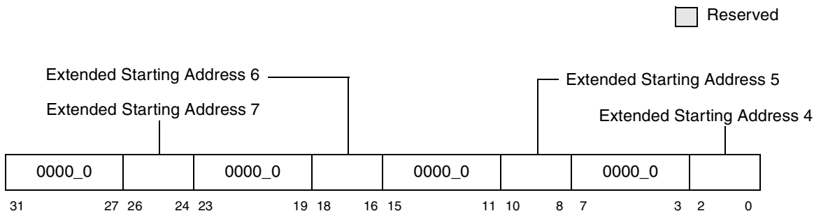
Figure 4-13. Extended Memory Starting Address Register 2—0x8C
