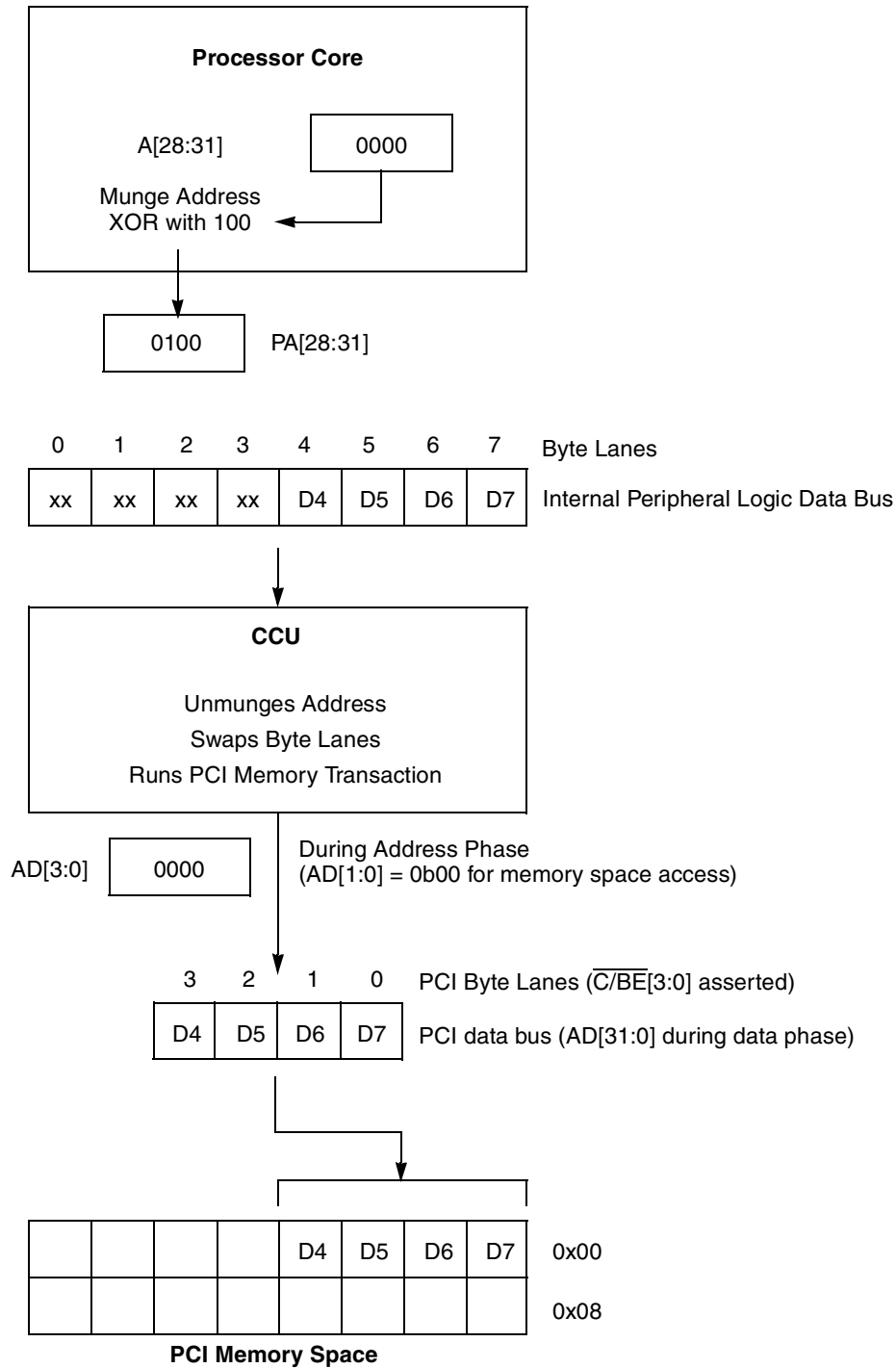
Figure A-8. 4-Byte Transfer to PCI Memory Space—Little-Endian Mode
