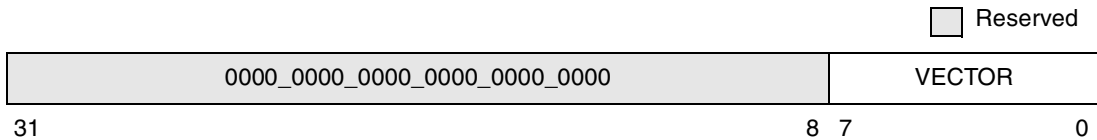
Figure 11-9. Spurious Vector Register (SVR)
