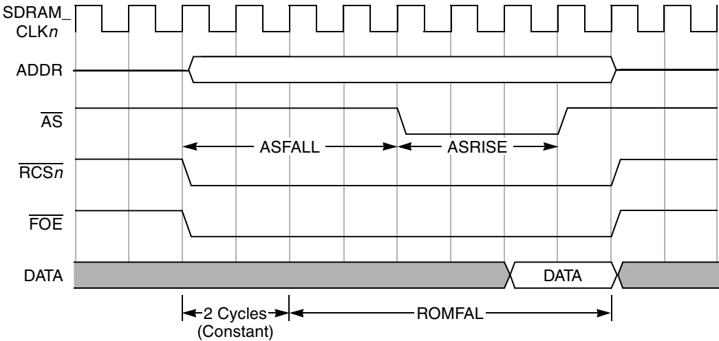
Figure 6-50. Port X Read Access Timing
