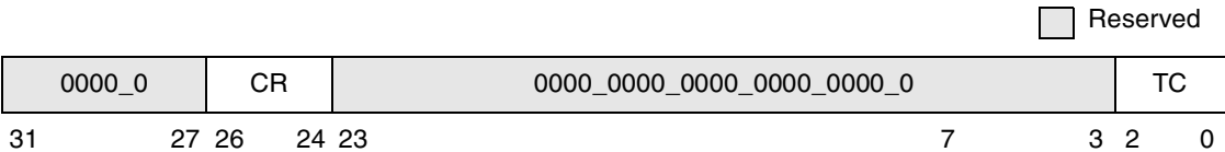
Figure 11-11. Timer Control Register
