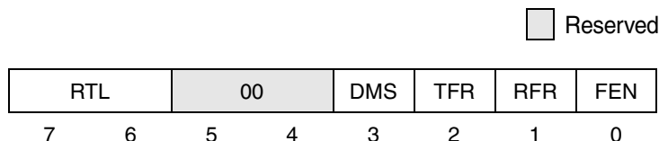
Figure 12-9. FIFO Control Register (UFCR)
