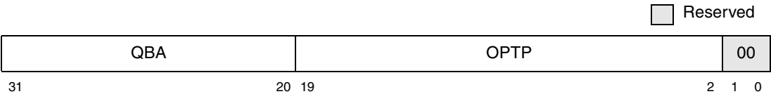
Figure 9-18. Outbound Post_FIFO Tail Pointer Register (OPTPR)
