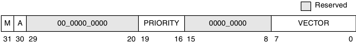
Figure 11-14. Global Timer Vector/Priority Registers (GTVPRs)
