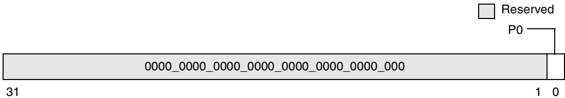
Figure 11-15. Global Timer Destination Registers (GTDRs)
