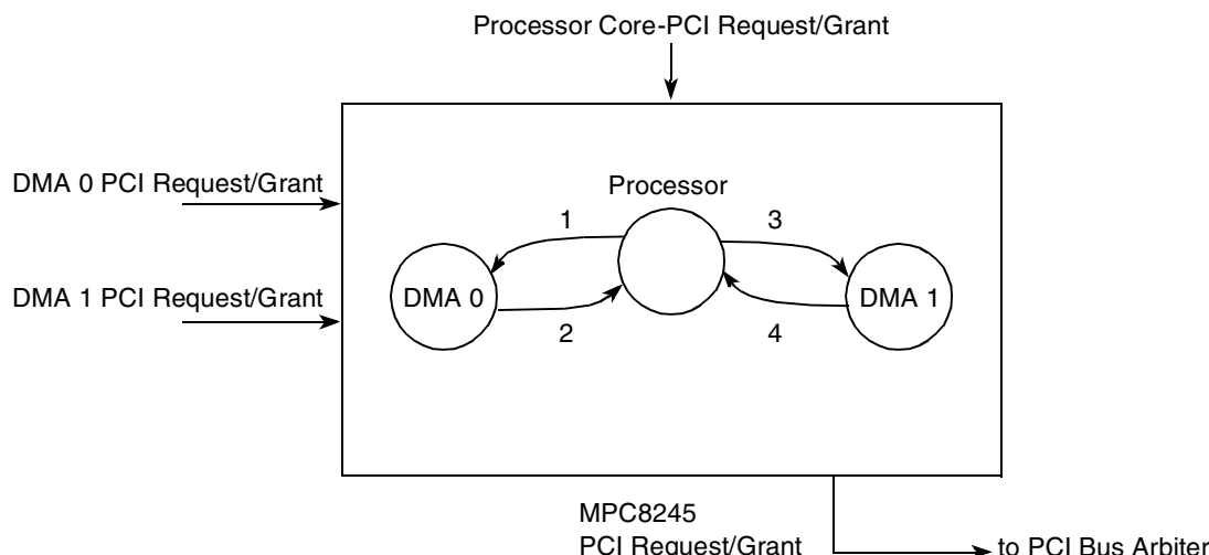
Figure 7-1. Internal Processor DMA Arbitration for PCI Bus
