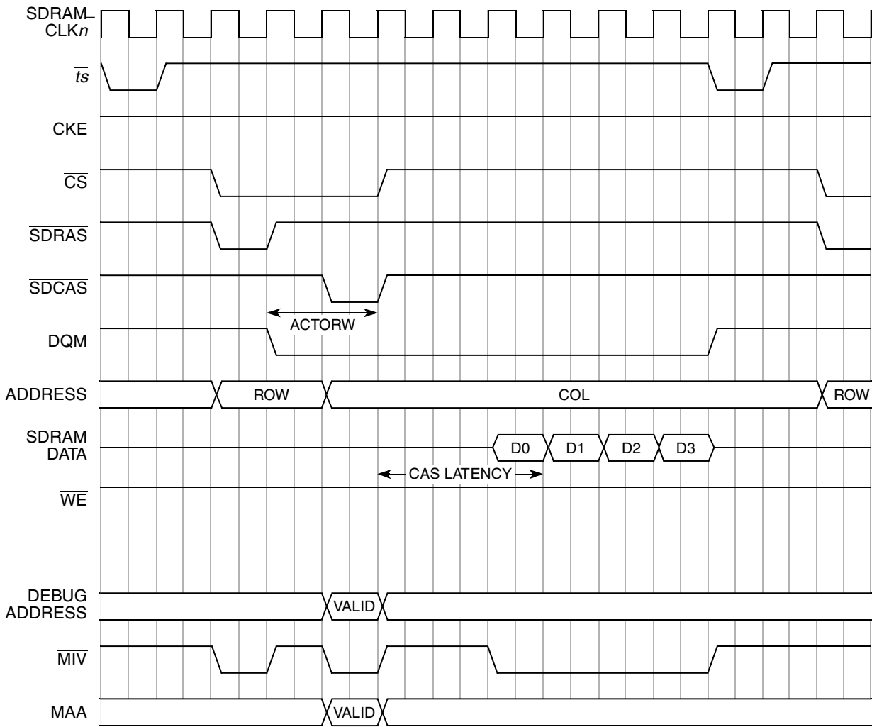
Figure 17-9. SDRAM Debug Address, \overline{MIV} , and MAA Timings for Burst Read Operation
