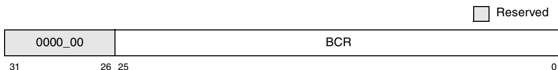
Figure 8-12. Byte Count Register (BCR)
