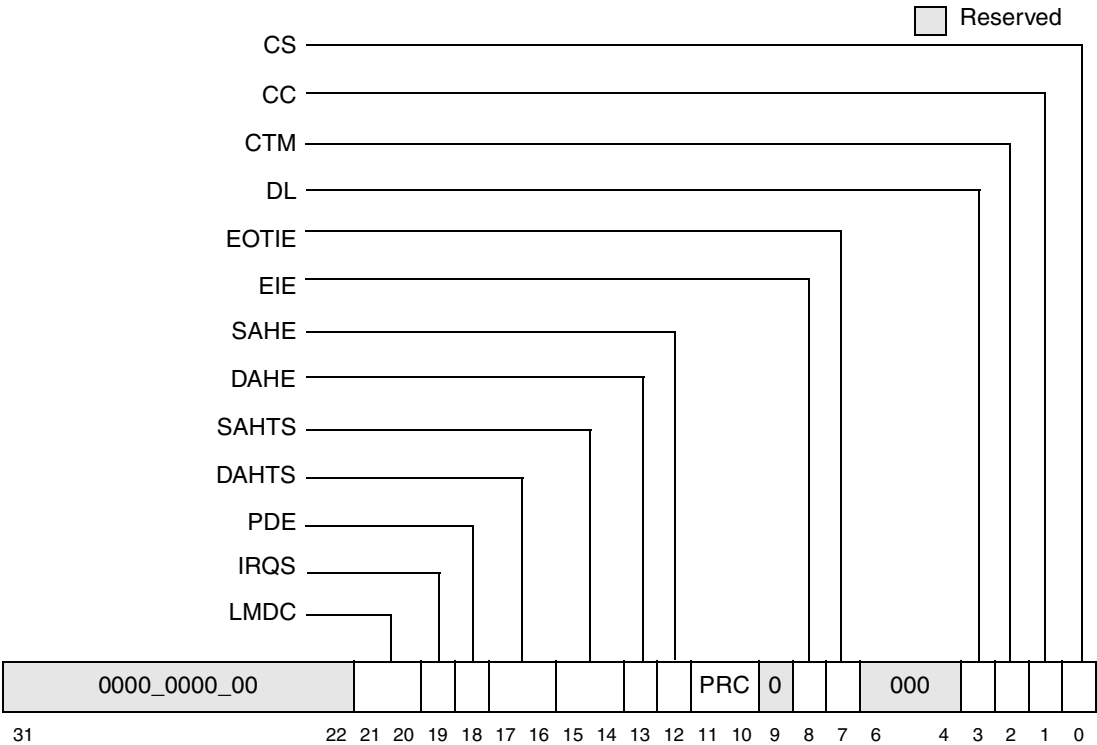
Figure 8-4. DMA Mode Register (DMR)
