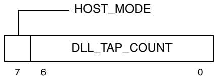
Figure 4-33. DLL Tap Count Register (DTCR)
