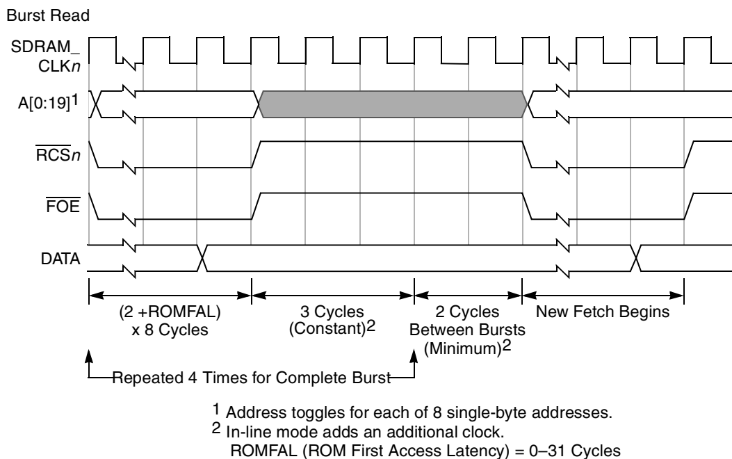
Figure 6-43. 8-Bit ROM/Flash Interface—Cache-Line Read Timing
