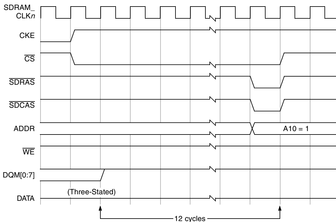
Figure 6-19. SDRAM Self-Refresh Exit
