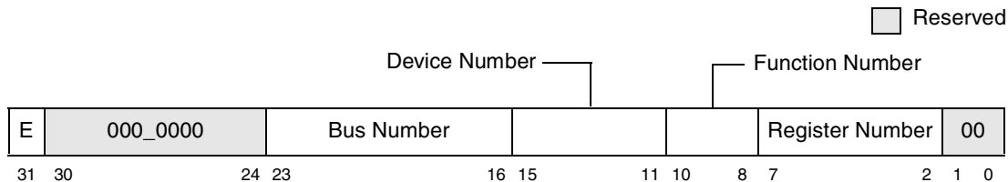
Figure 7-13. CONFIG_ADDR Register Format
