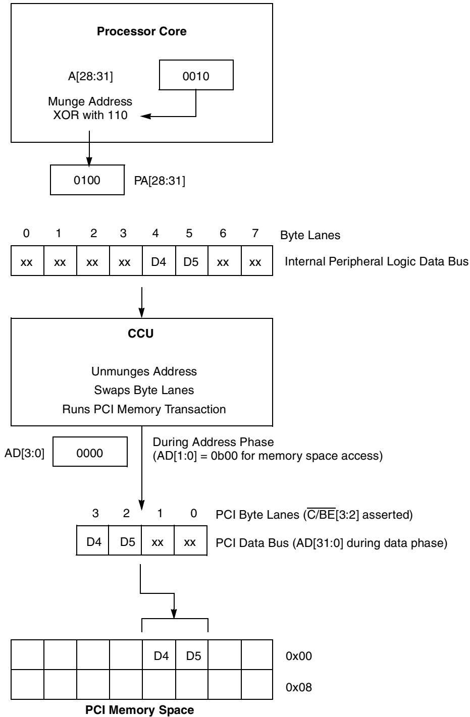
Figure A-7. 2-Byte Transfer to PCI Memory Space—Little-Endian Mode
