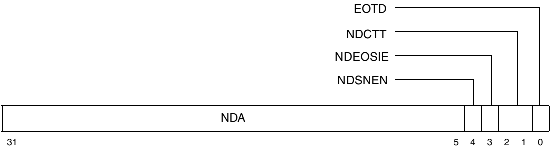
Figure 8-13. Next Descriptor Address Register (NDAR)
