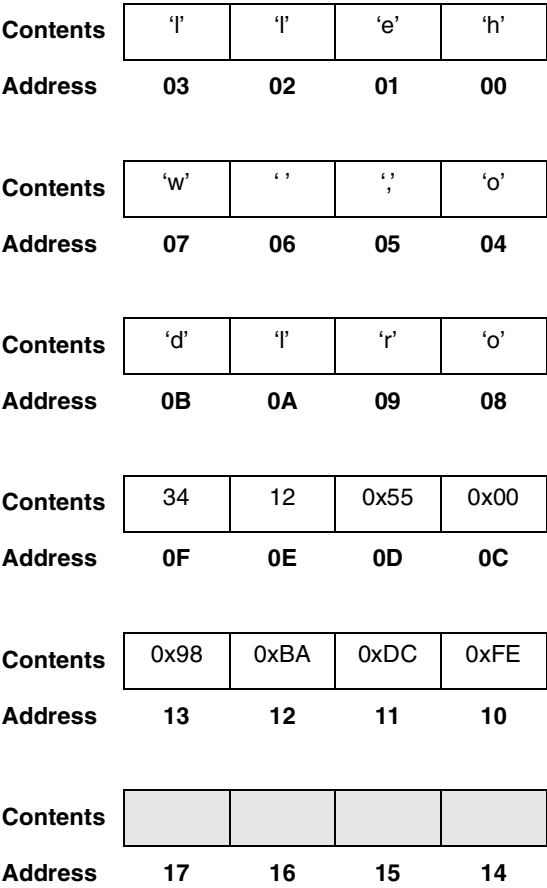
Figure A-3. Big-Endian Memory Image in Big-Endian PCI Memory Space
