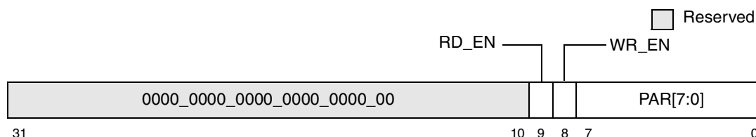
Figure 17-17. Parity Error Injection Mask—Offsets 0xF_F008, 0xF08
