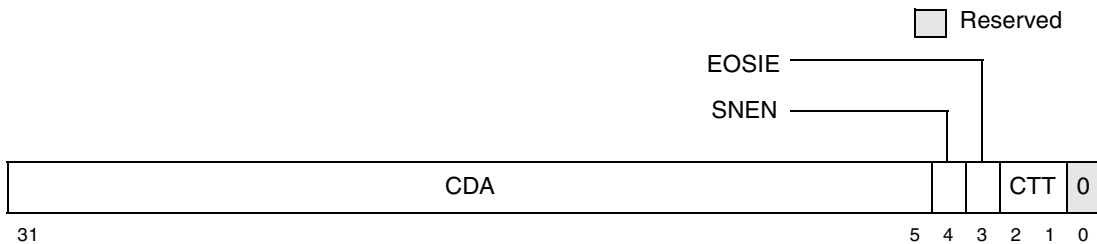
Figure 8-6. Current Descriptor Address Register (CDAR)
