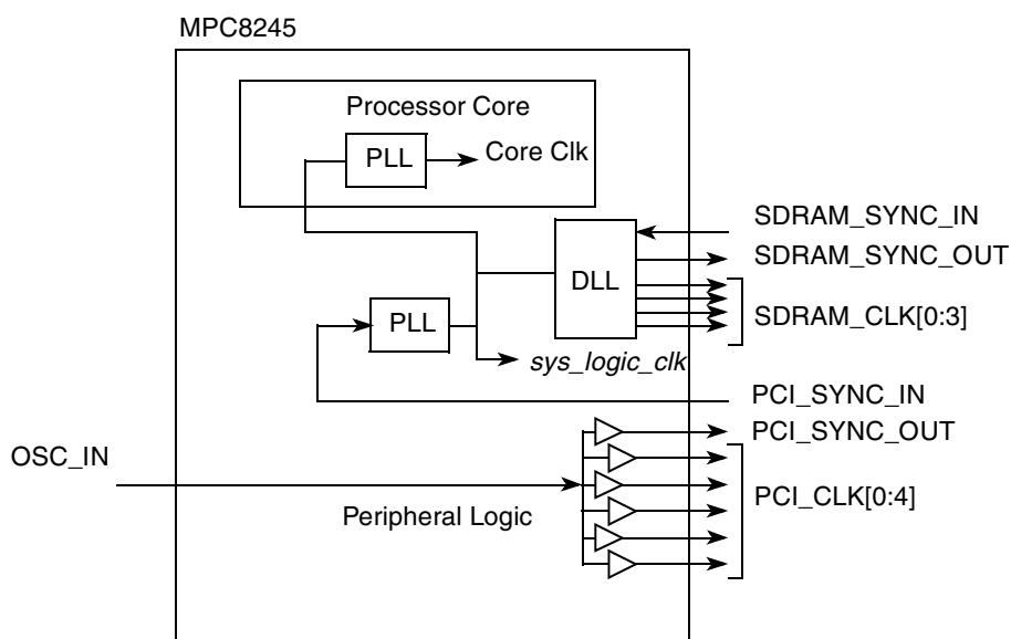
Figure 2-2. Clock Subsystem Block Diagram
