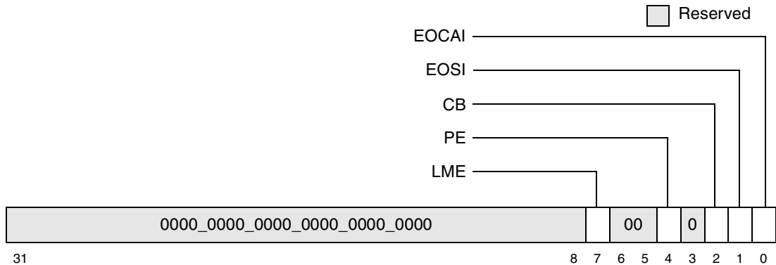
Figure 8-5. DMA Status Register (DSR)
