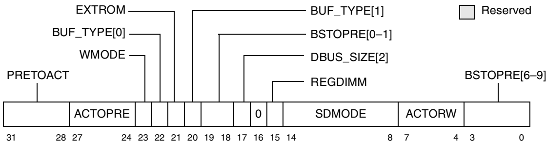
Figure 4-37. Memory Control Configuration Register 4 (MCCR4)—0xFC
