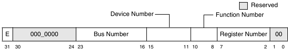
Figure 7-13. CONFIG_ADDR Register Format
