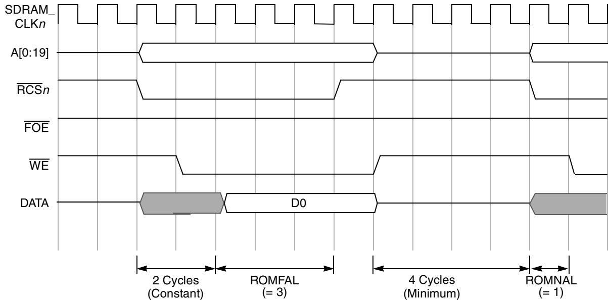
Figure 6-47. 8-, 32-, or 64-Bit Flash Write Access Timing
