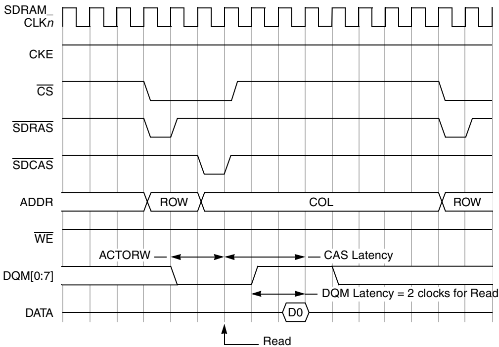
Figure 6-10. SDRAM Single-Beat Read Timing (SDRAM Burst Length = 4)
