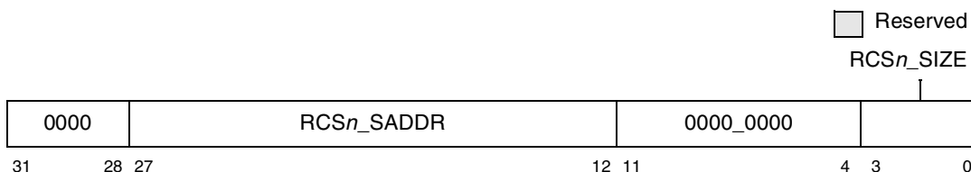
Figure 4-29. ERCCR3 and ERCCR4—0xDC
