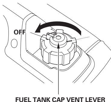
NON-CALIFORNIA TYPE
