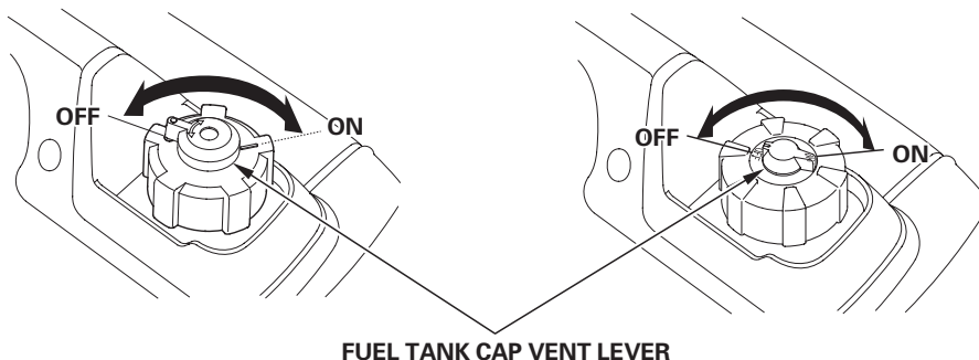
NON-CALIFORNIA TYPE
