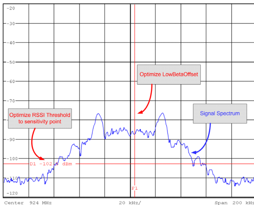
Figure 9. Signal Spectrum with LowBetaOffset and sensitivity illustrated
