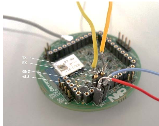
Fig 22. Connections for serial flashing
