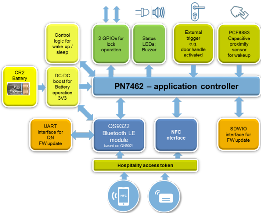
Fig 3. Main building blocks
