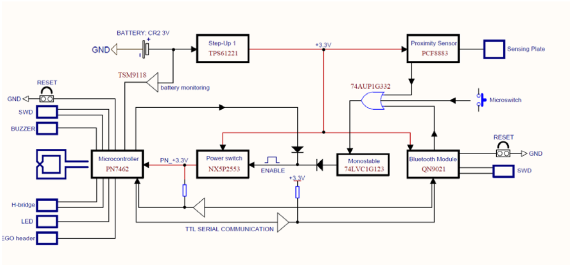
Fig 4. OM27642NBR NFC- Bluetooth Low Energy Module with PN7462 stack on core module
