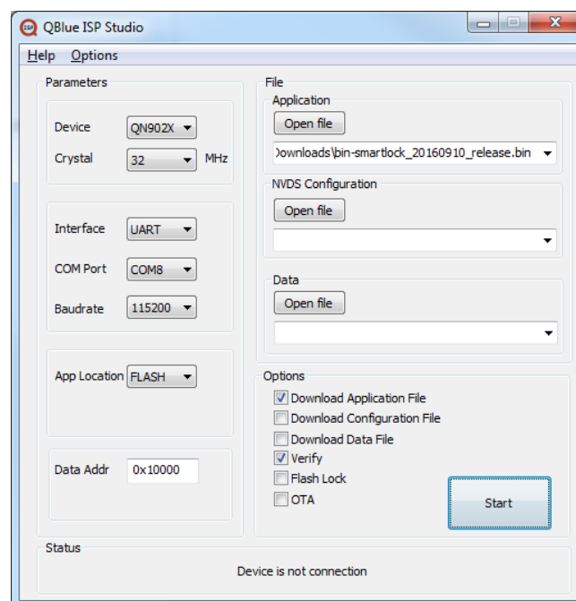
Fig 23. Options for serial flashing
