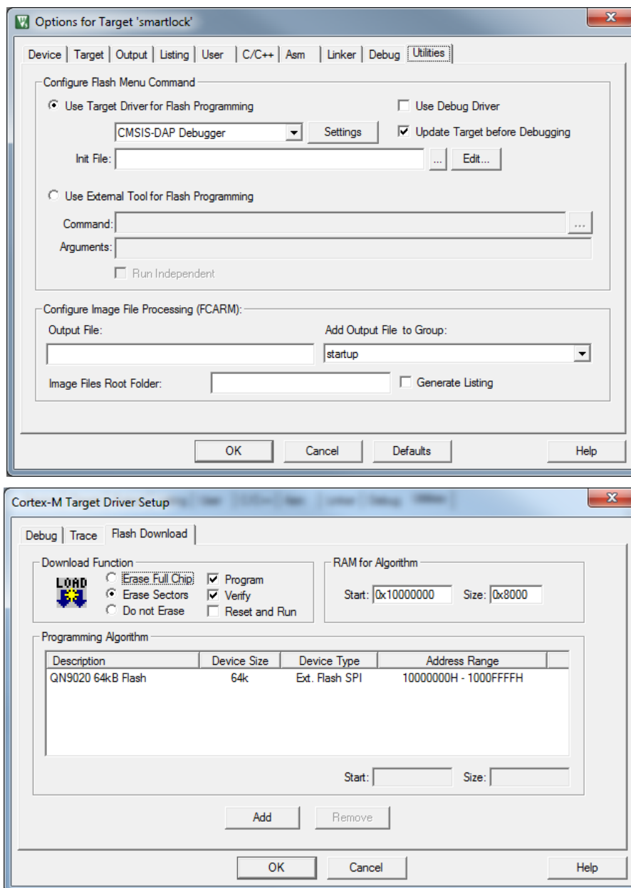
Fig 21. Configure Utilities in Keil
