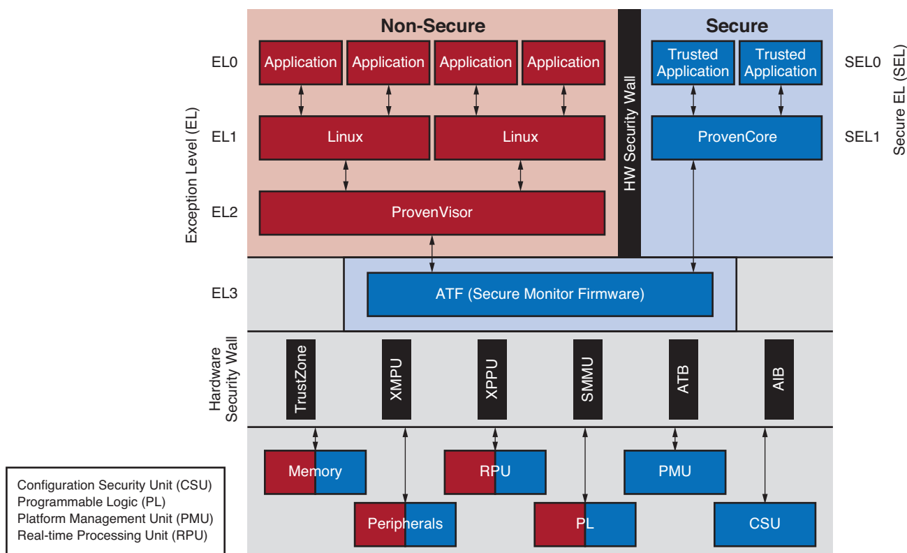
Figure 4: ProvenCore Running on Zynq UltraScale+ Platform
