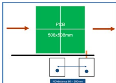
Cerno® 508.1PD 2seg soldering one panelized board with dual nozzles
