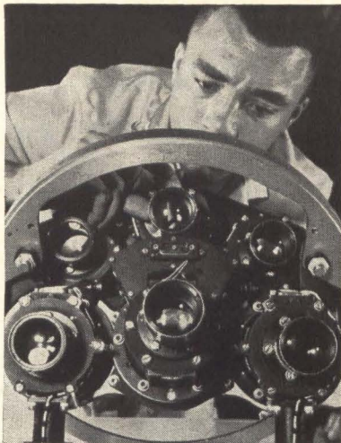
SIX TV CAMERAS—three wide-angle and three narrow-angle—will take the first close-up tv pictures of the moon
