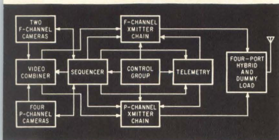
CAMERA CHAINS for the full-scan and partial-scan channels are independent. F-channel is transmitted at 959.52 Mc, P-channel at 960.58 Mc
