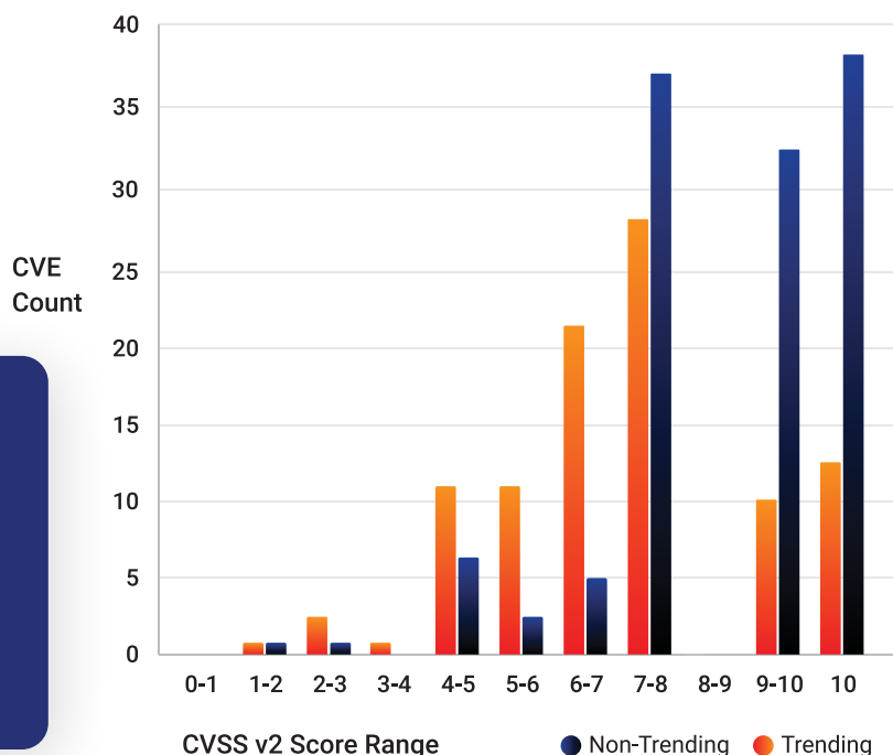
Vulnerabilities Tied to Ransomware with Severity Scoring CVSS v2 (2018-2020)
