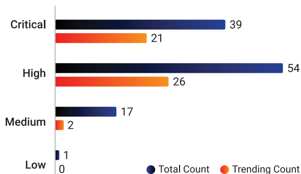
Vulnerabilities Tied to Ransomware with CVSS v3 Scoring (2018-2020)
