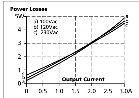
Fig. 8-2 Losses vs. output current at 5V, typ.
