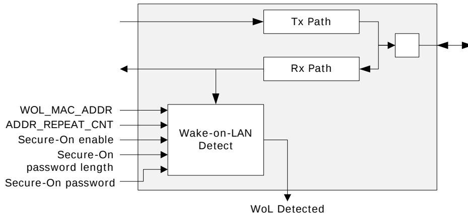
FIGURE 4-15: WAKE-ON-LAN FUNCTIONALITY
