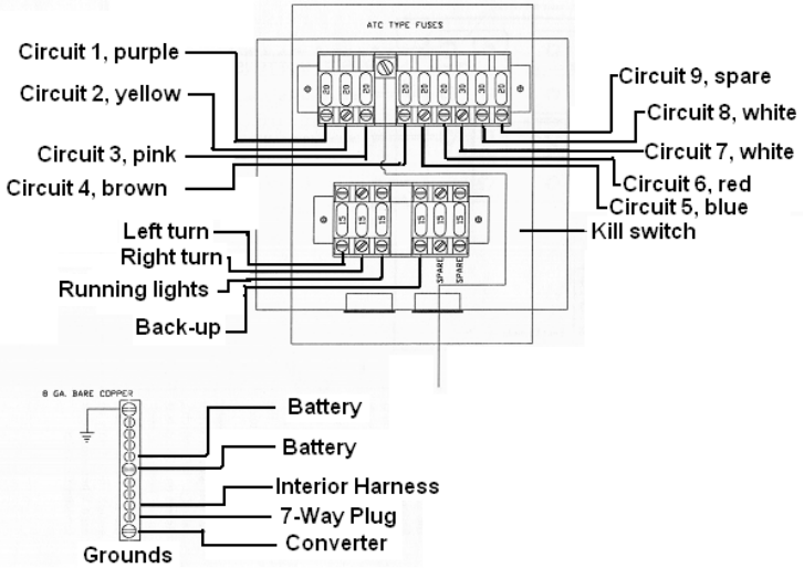
Canadian 12-Volt Distribution
