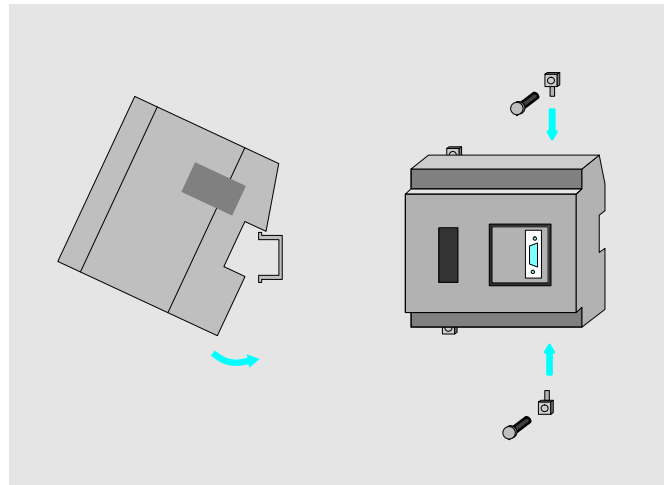
Fig. 2/2 Mounting
