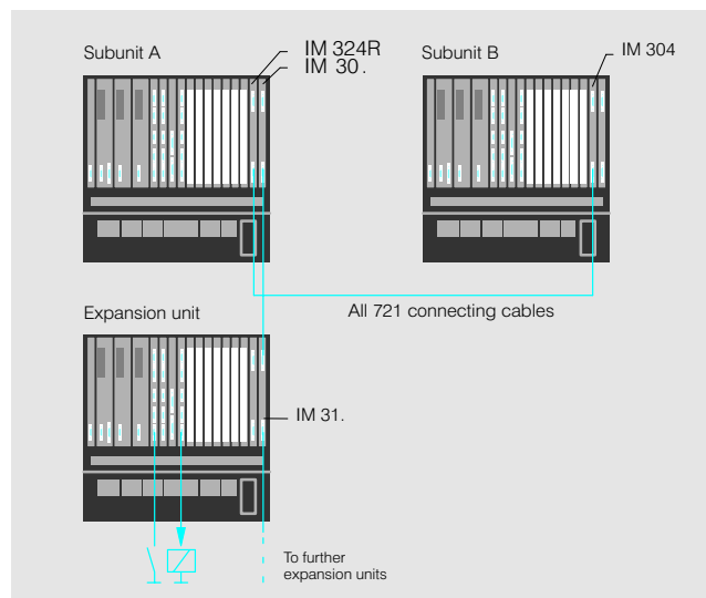
Fig. 4/14 Single-sided configuration (normal availability)
