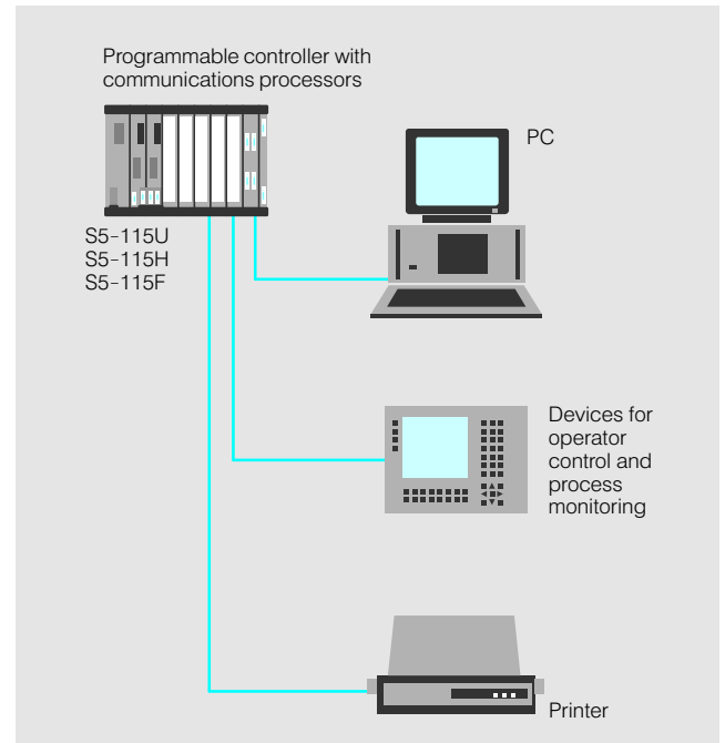
Fig. 3/6 Connections between programmable controller and PC, operator control and process monitoring equipment and printer
