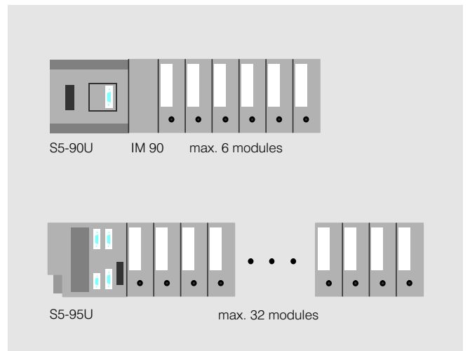
Fig. 2/3 Expansion
