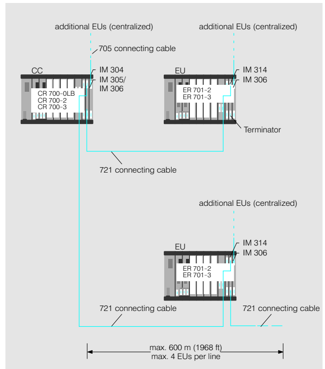
Fig. 3/34 Connection of expansion units to the central controller in distributed configuration using IM 304 and IM 314 interface modules
