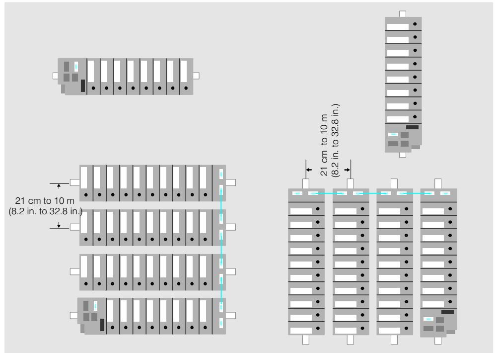
Fig. 2/14 Possible configurations
