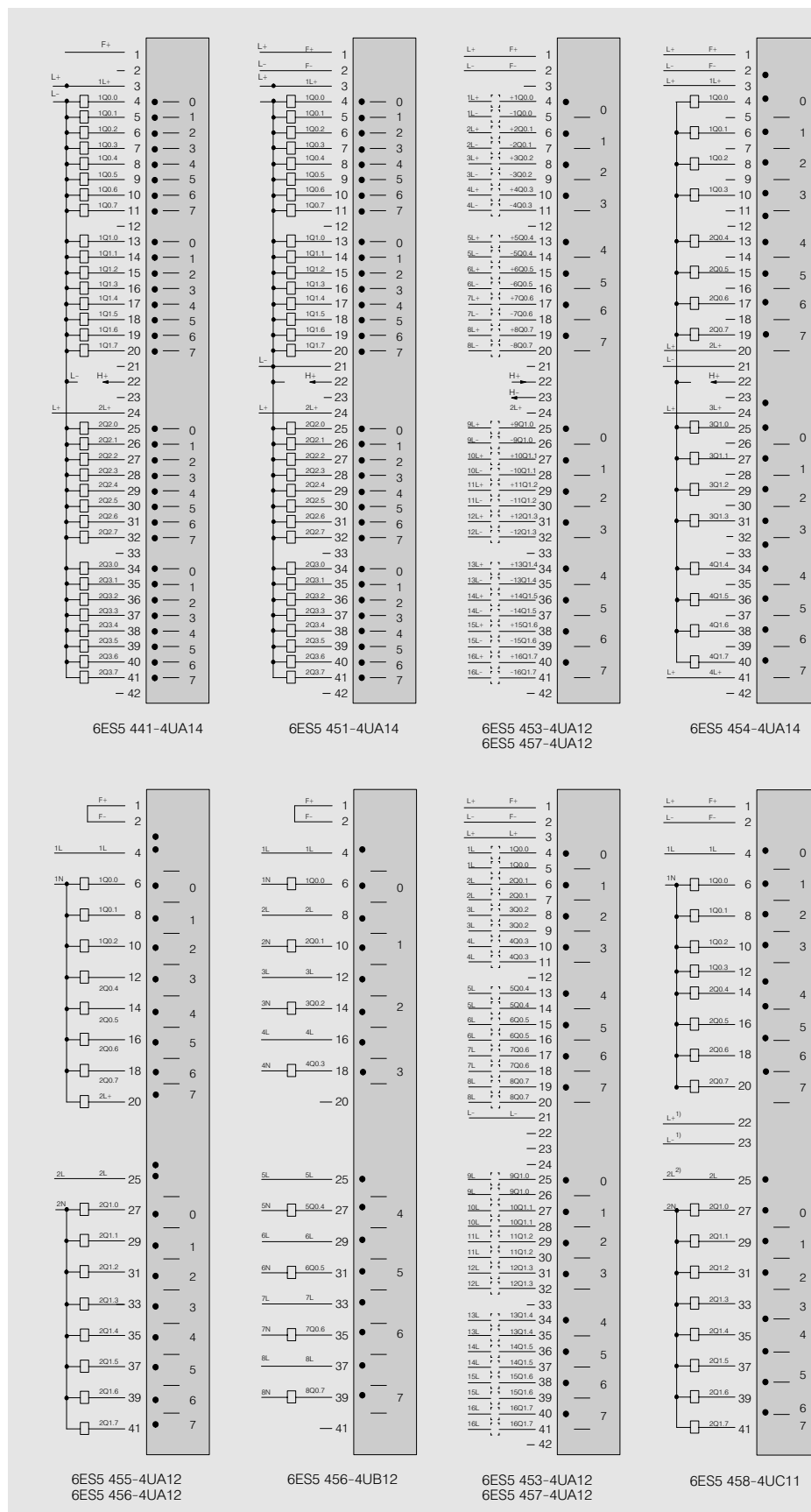
Fig. 4/24 Connection diagrams of digital output modules
