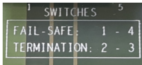
Figure 18: Fail-safe Status and Termination Resistor on PCB
