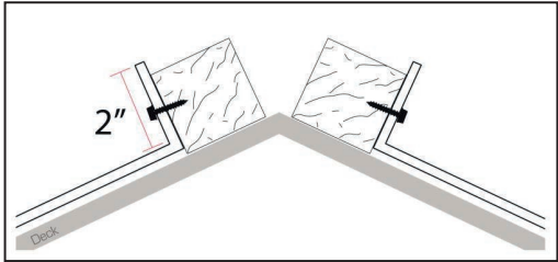
Figure 13. Panels at ridge
