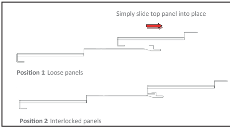
Figure 1. Znap Mechanism
