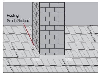
Figure 20. (1) Install roof-to-wall channel on both sides and at the back of the chimney; bend the front panel upwards as you would at a ridge. (2) Seal all around the chimney with roofing grade sealant. (3) Install Z bar around chimney.
