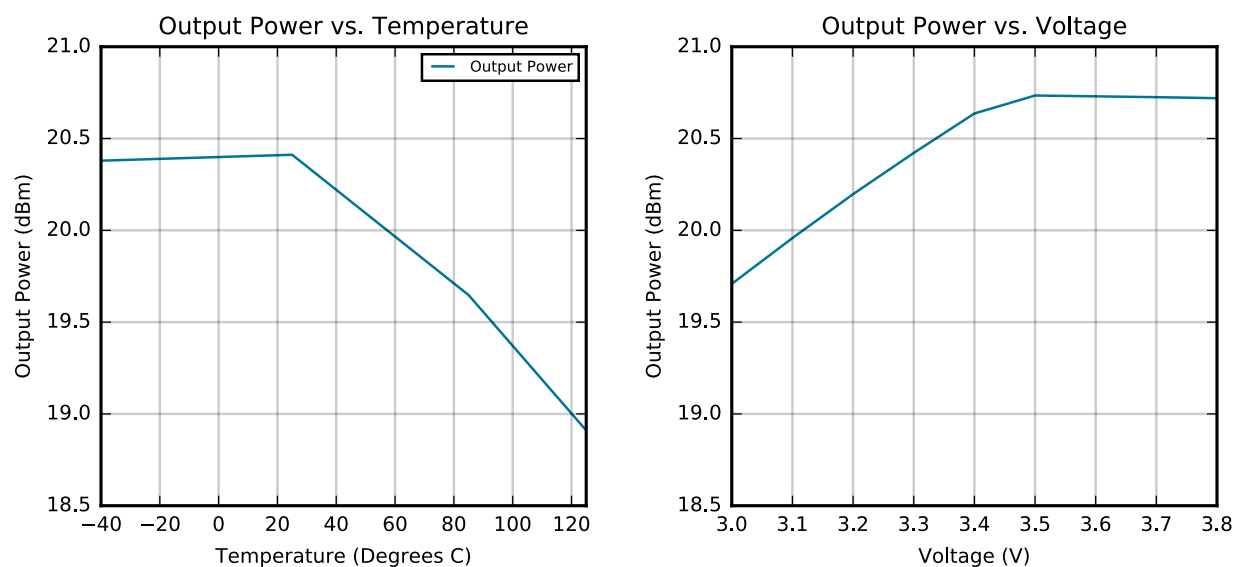
Figure 4.3. 2.4 GHz 20 dBm PA RF Transmitter Output Power
