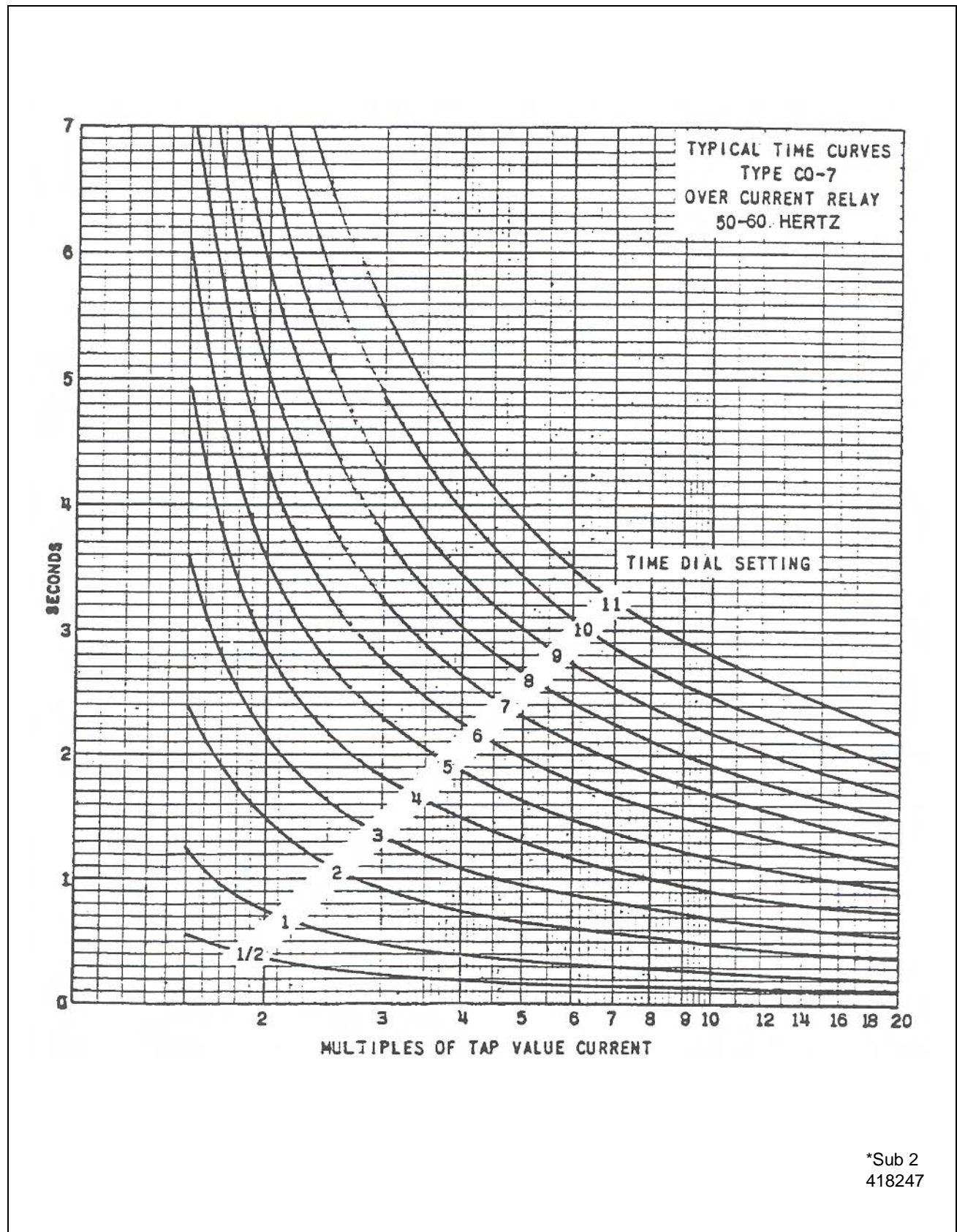
Figure 10: Typical Time Curves of the Type CO-7 Relay
