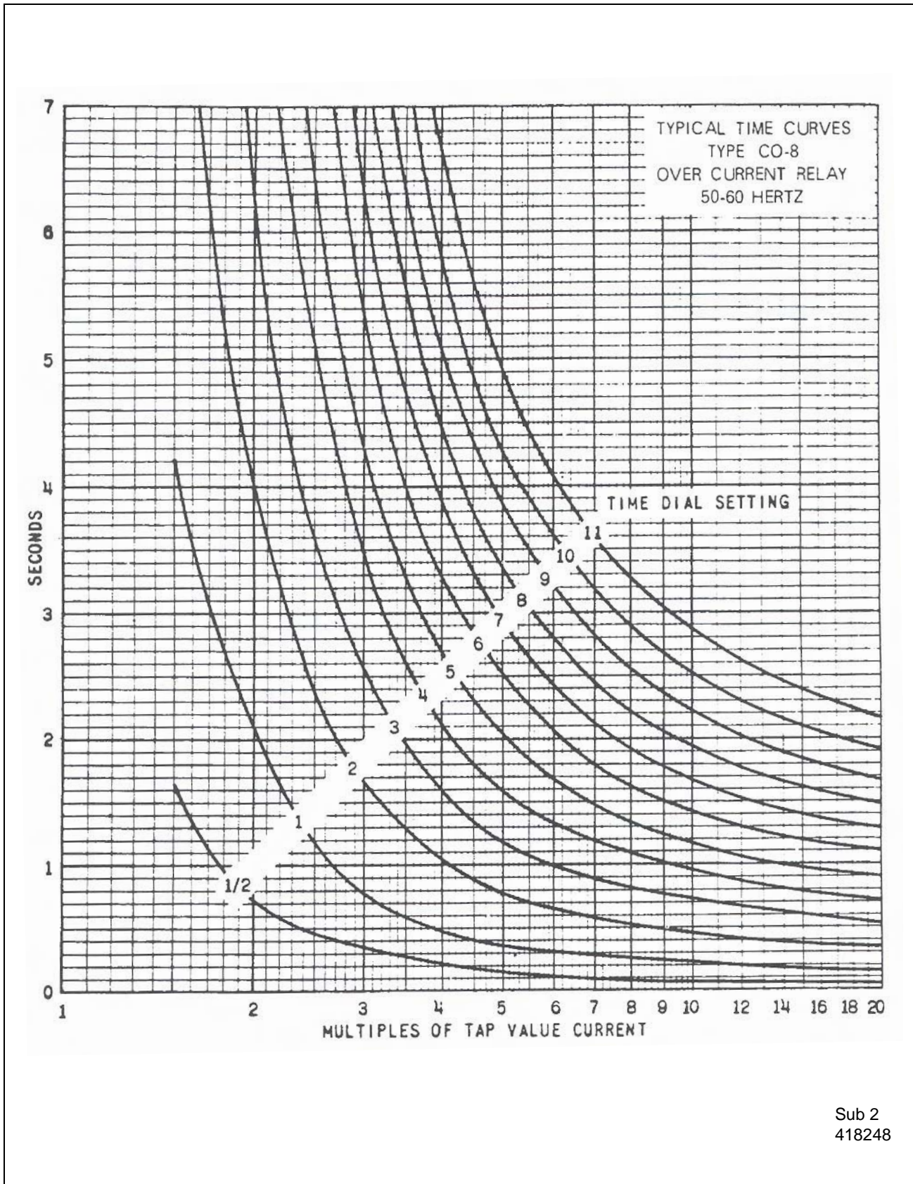
Figure 11: Typical Time Curves of the Type CO-8 Relay
