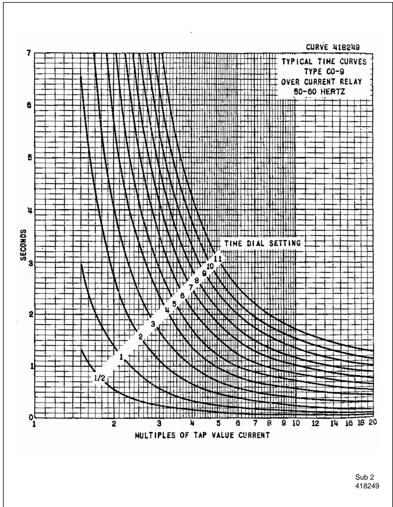
Figure 12: Typical Time Curves of the Type CO-9 Relay.
