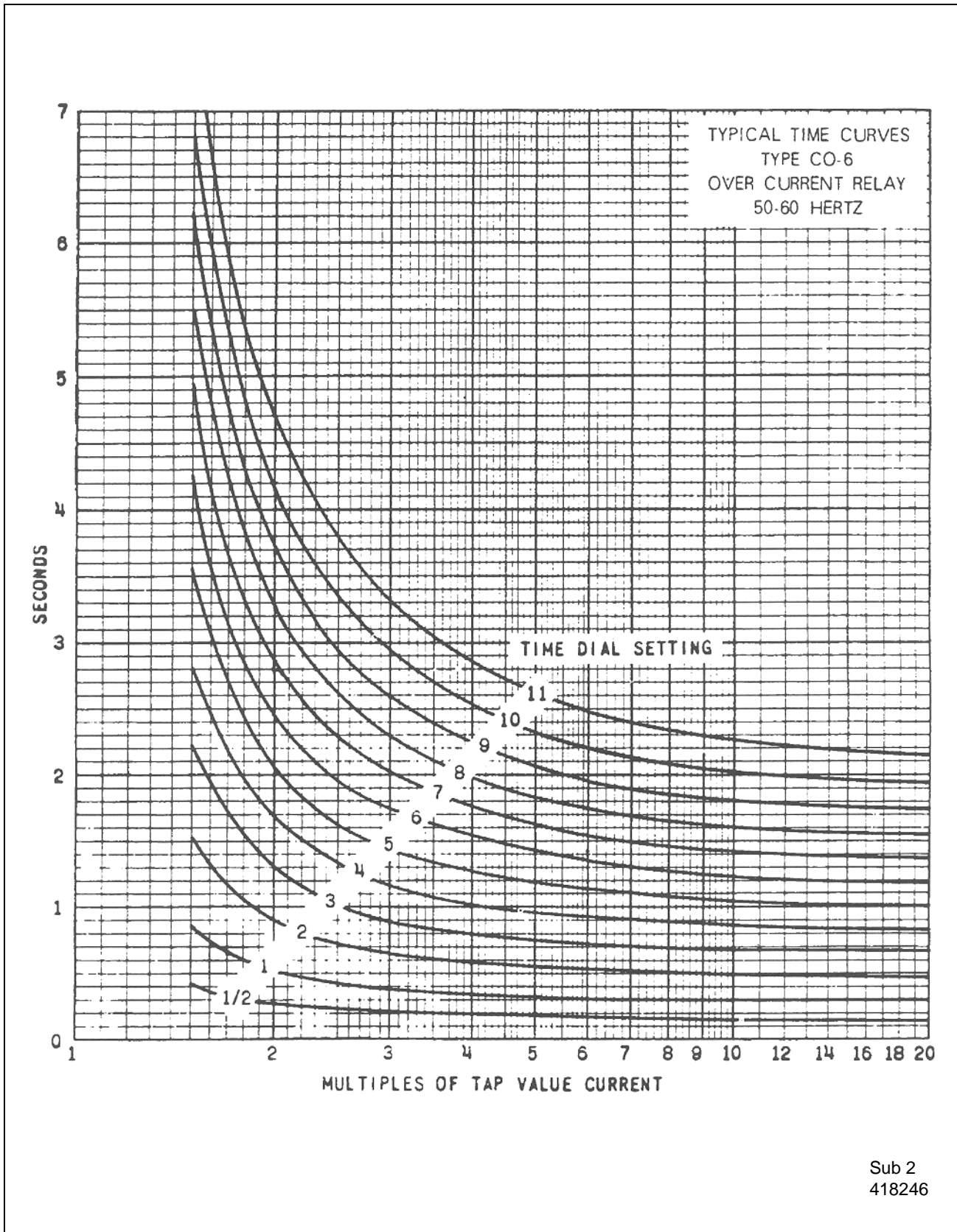
Figure 9: Typical Time Curves of the Type CO-6 Relay
