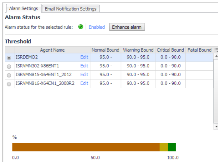
Figure 32. The colored bar across the bottom of the view indicates the percentage of collections that fall within each threshold.
