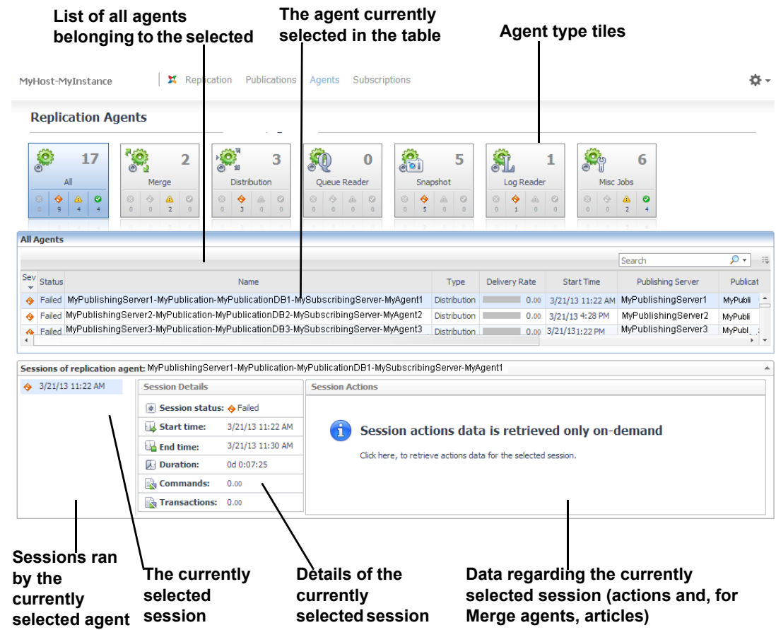
Figure 9. The Replication Agents drilldown.
