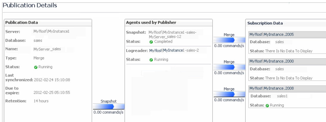
Figure 8. The Publication Details screen.
