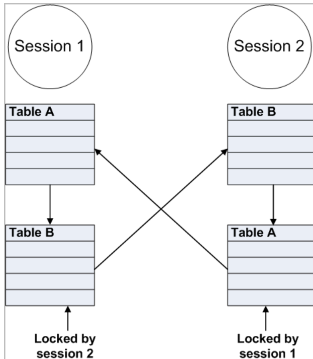
Figure 34. The following scenario details the simplest example of a deadlock, which involves only two sessions:
