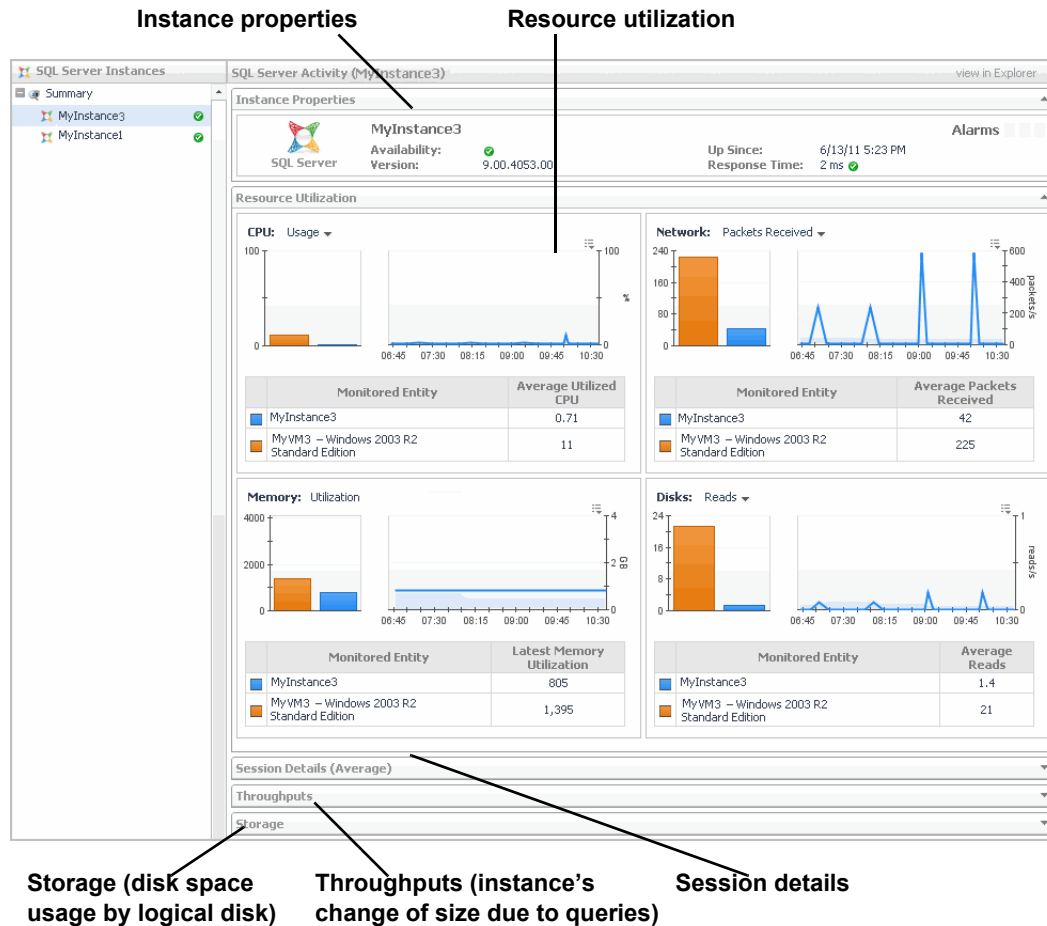
Figure 36. The SQL Server Activity view.
