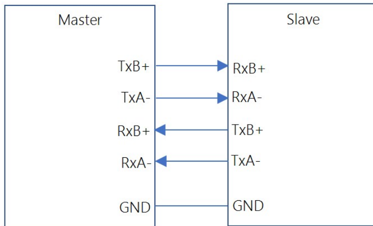
FIGURE 7-2. Differential-pair full-duplex communications
