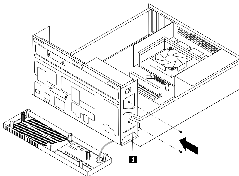
Figure 31. Installing the optical drive
