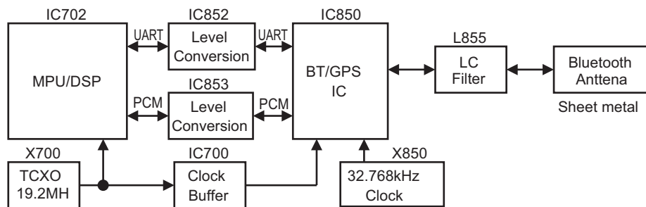
Fig.6 Bluetooth circuit
