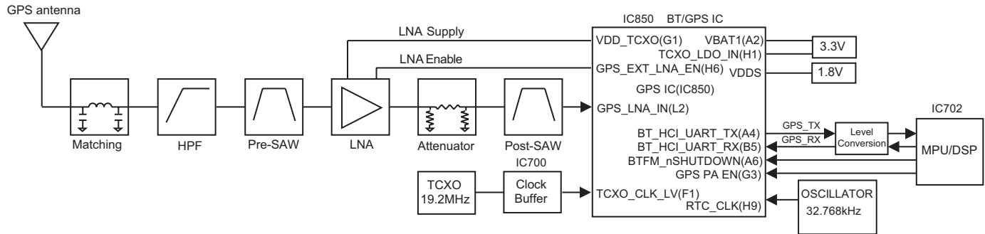
Fig.7 GPS circuit
