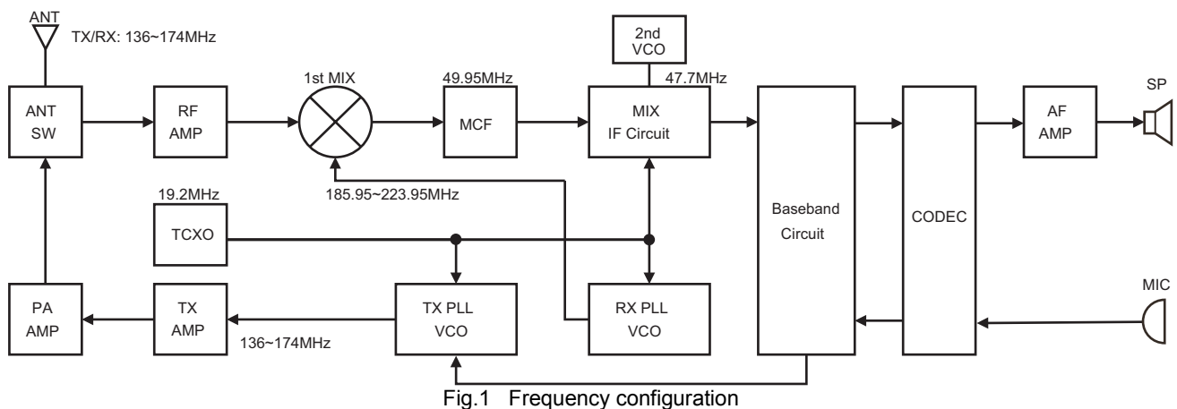
Fig.1 Frequency configuration
