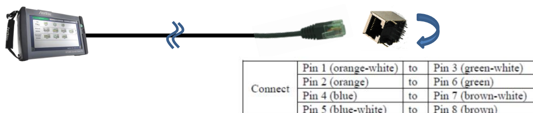
Fig. 3.4-1 Network configuration for sample scenario commissioning test
