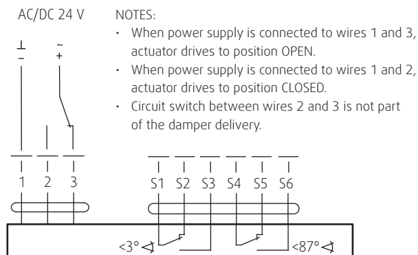
Fig. 5: Connection of the actuator BELIMO BLE 24
