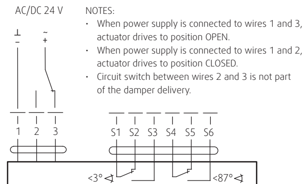
Fig. 6: Connection of the actuator BELIMO BE 24-12-ST
