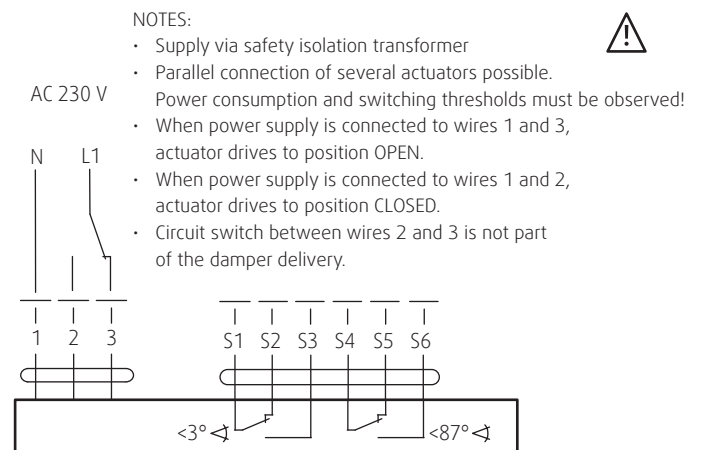
Fig. 4: Connection of the actuator BELIMO BE 230-12
