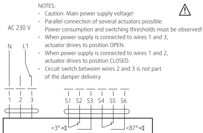
Fig. 3: Connection of the actuator BELIMO BLE 230
