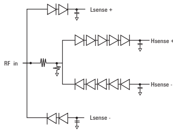
Figure 5. Simplified block diagram of the two-path-diode-stack topology.
