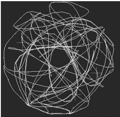
Figure 1. The 3/8 shifted-8PSK digital modulation format, emerging for use in wideband data transmission on wireless channels, as with EDGE technology.
