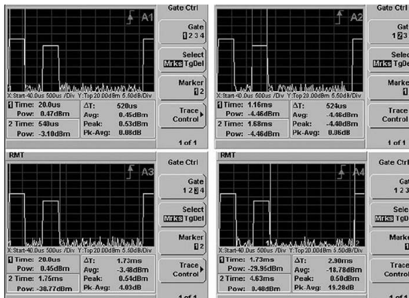
Figure 9. Measurement flexibility with four independent time gates
