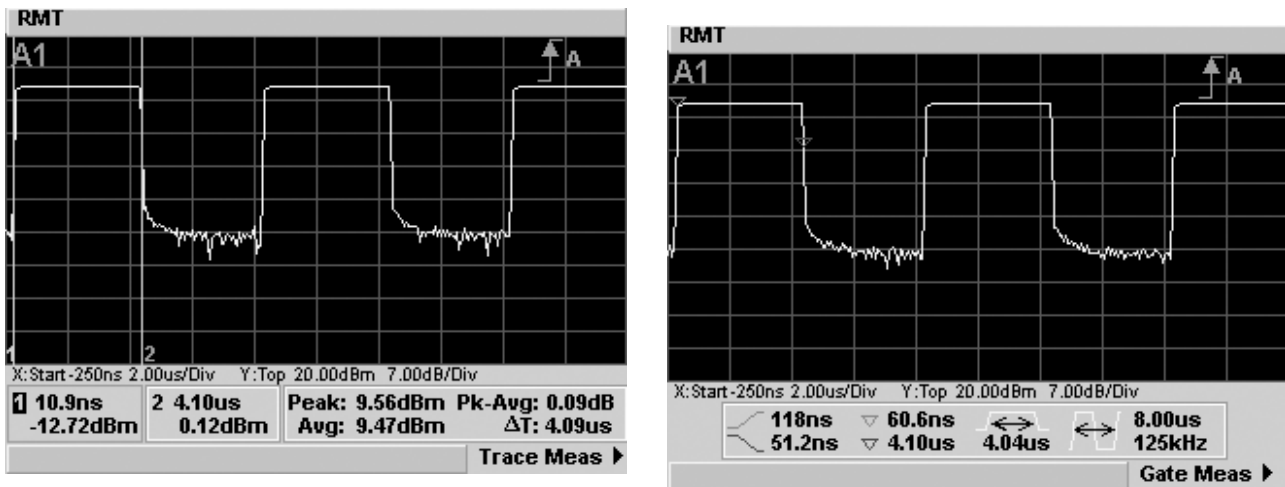
Figure 8. Large color display with automatic power and time measurements
