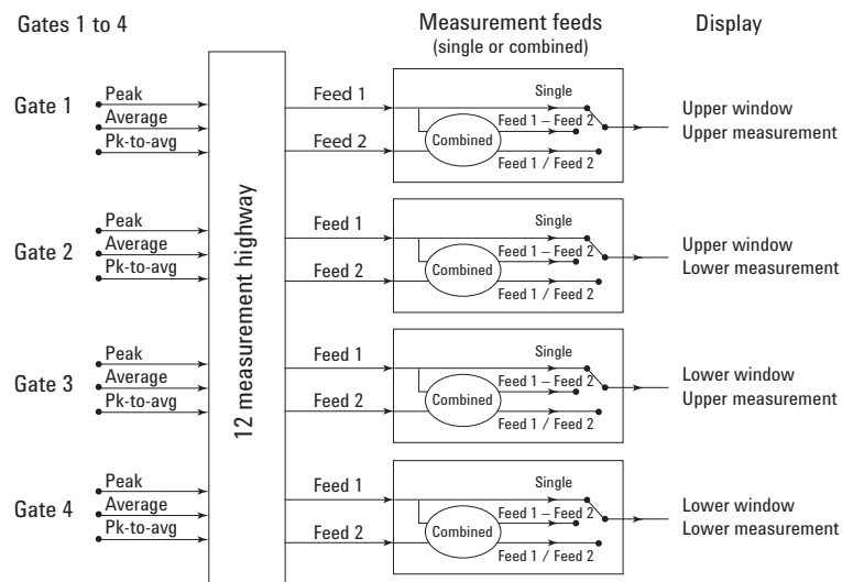
Figure 20. User-configured data manipulations: a major feature of the EPM-P Series power meters.
