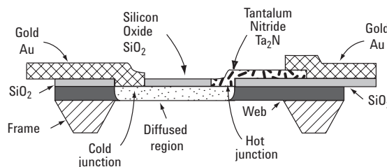
Figure 3. Cross section of Keysight thermocouple chip, where power dissipated in the tantalum-nitride resistor heats the hot junction.
