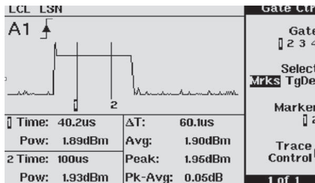
Figure 15. On this GSM pulse, powerful data configuration routines during four gate times, provide the feeds for the display.
