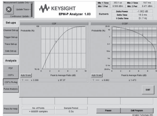
Figure 17. Y-axis shows the percent time the signal power is at or above the power specified by the X-axis.
