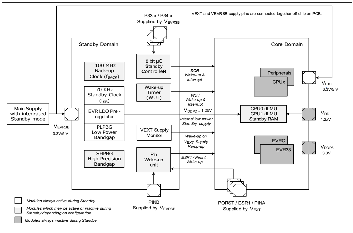
Figure 116 Standby domain supplied via a common supply rail connected to both VEXT and VEVRSB
