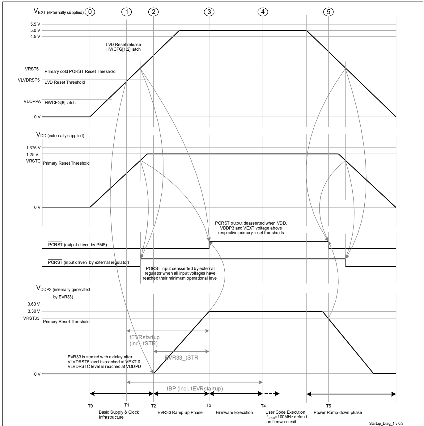
Figure 125 External Supply mode (d) - VEXT and VDD externally supplied
