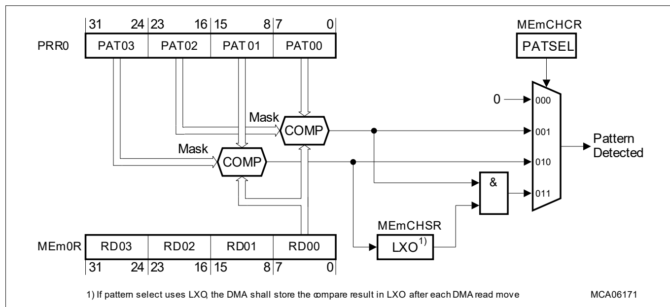
Figure 208 PATDET for 8-bit Channel Data Width and Move Data Byte stored in MEm0R.RD00
