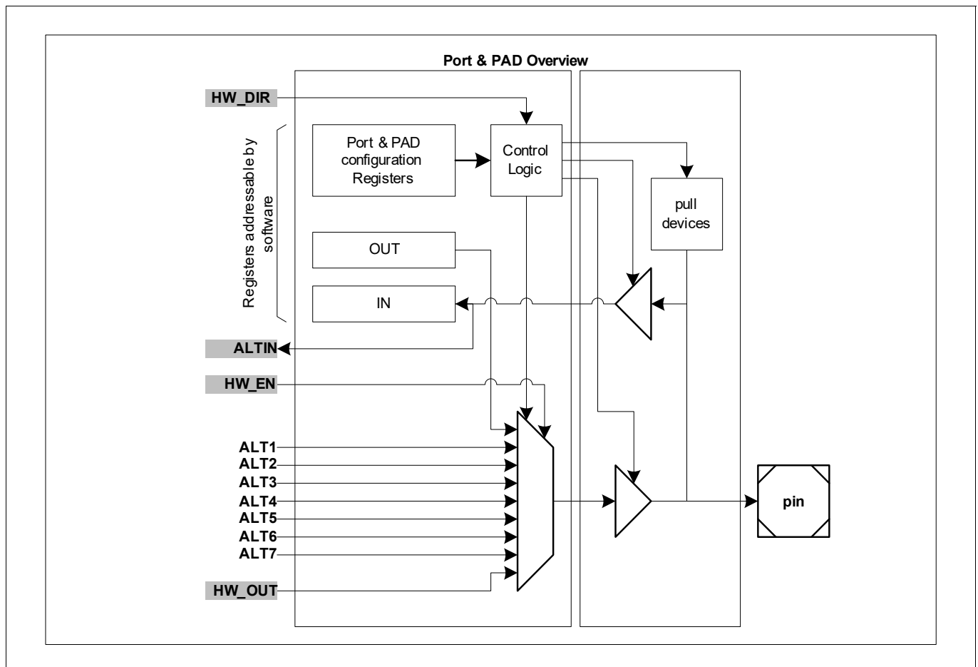
Figure 158 Generic Port Structure
