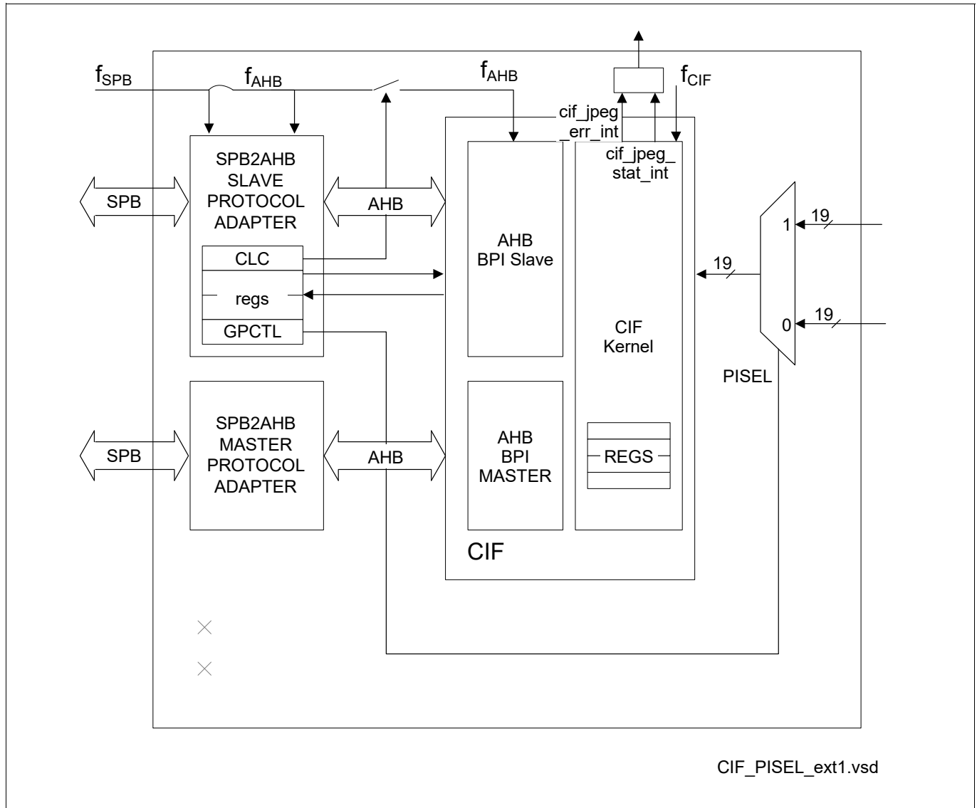
Figure 336 Overview of the SPB2AHB adapter
