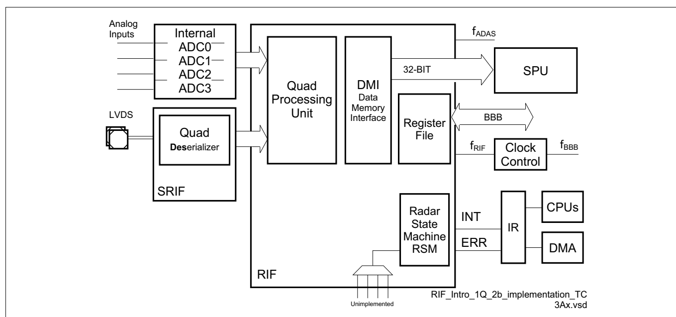
Figure 301 RIF Implementation for TC3Ax
