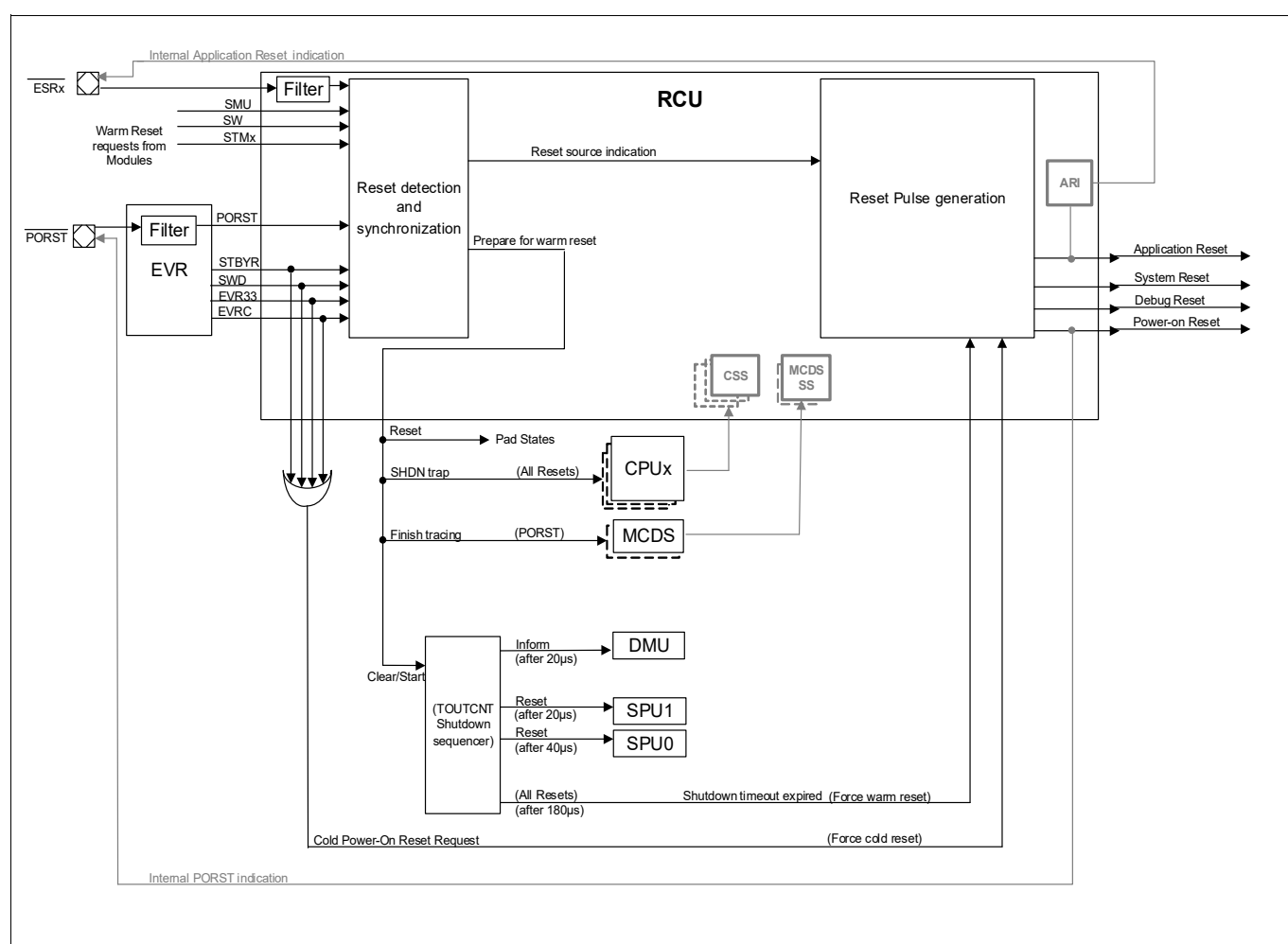
Figure 66 Reset Overview
