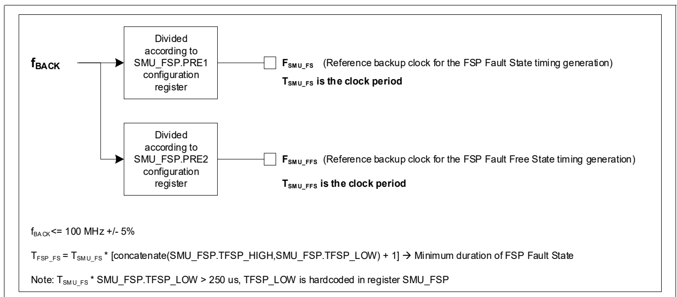
Figure 163 Reference clocks for FSP timings
