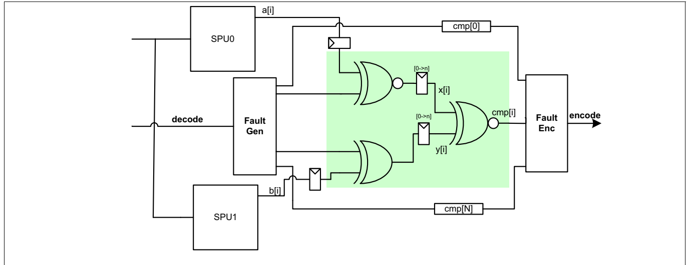
Figure 259 Node Comparator with Fault Injection
