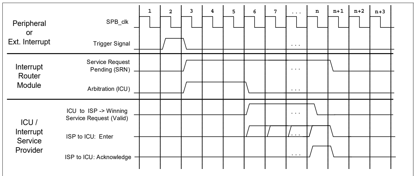
Figure 176 Interrupt System Timing (Schematic Overview, 3 Cycle Arbitration)
