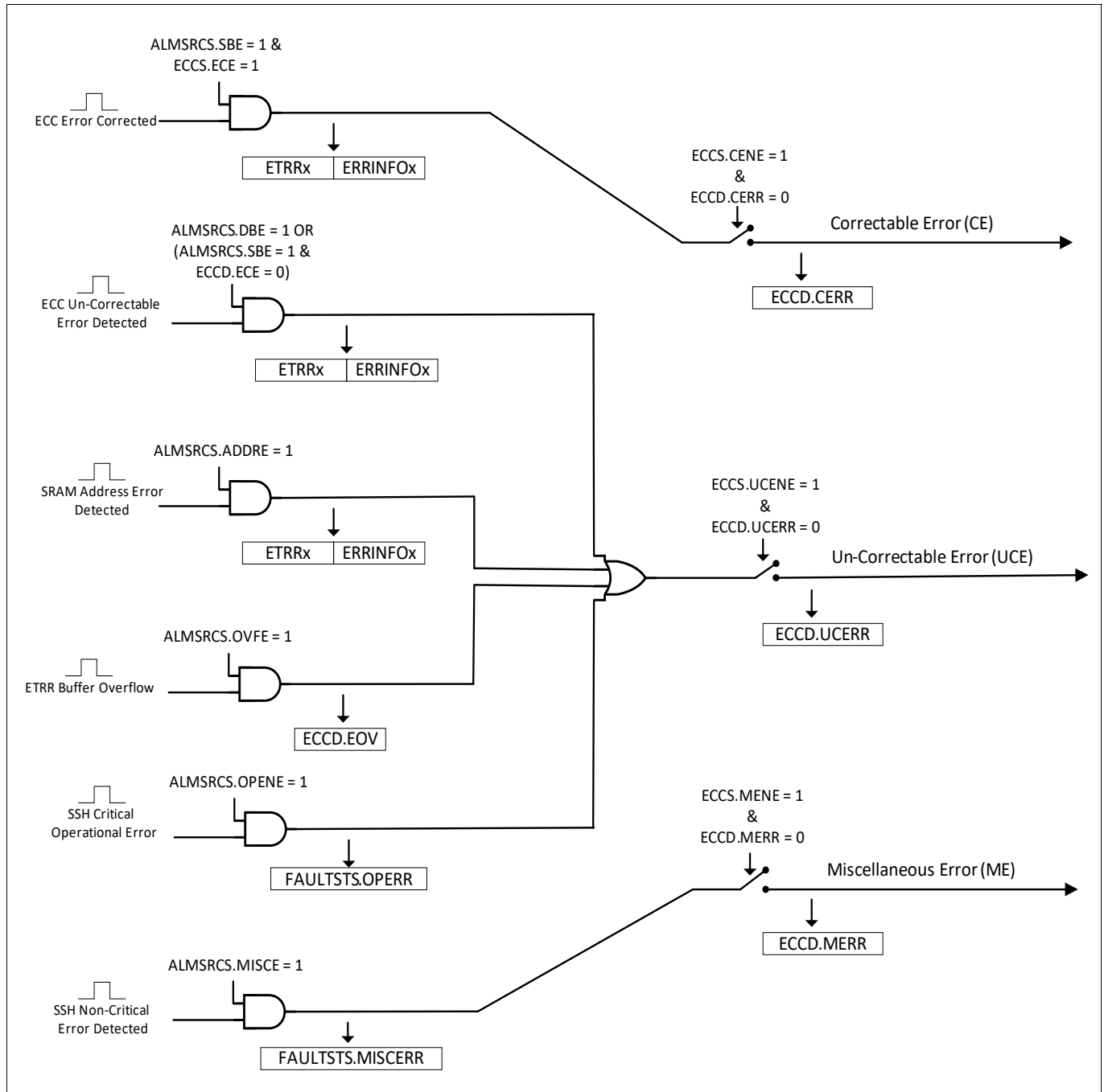
Figure 154 Alarms and Error Detection enabling (ECCS.TRE assumed to be set).
