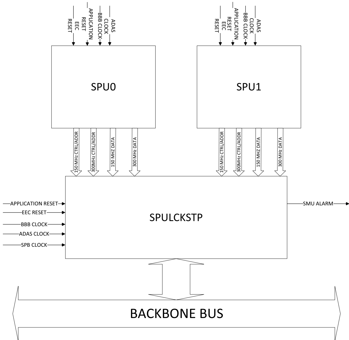
Figure 256 SPULCKSTP Interfaces
