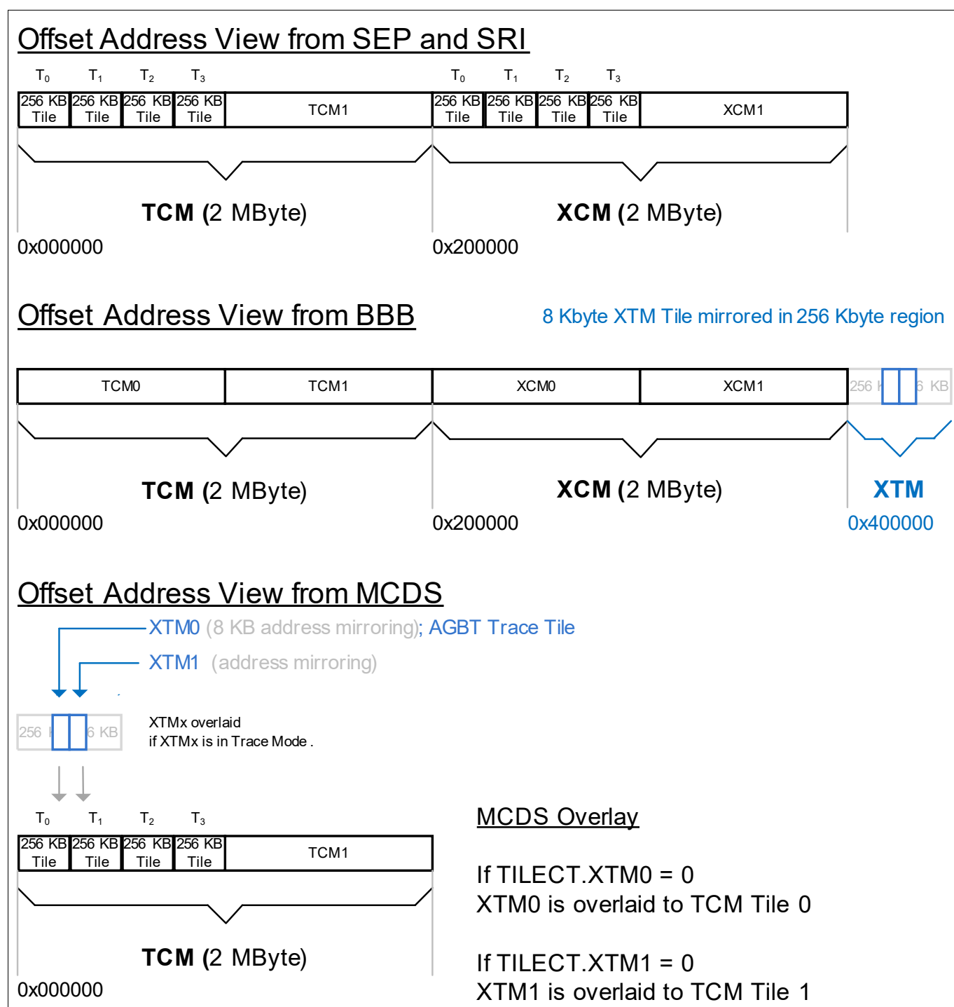
Figure 262 Offset Address View of TCM, XCM and XTM
