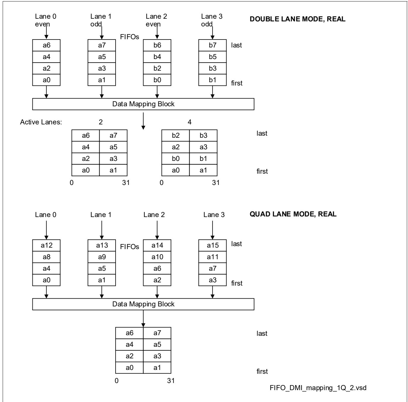
Figure 281 Multi Lane Real Sampling
