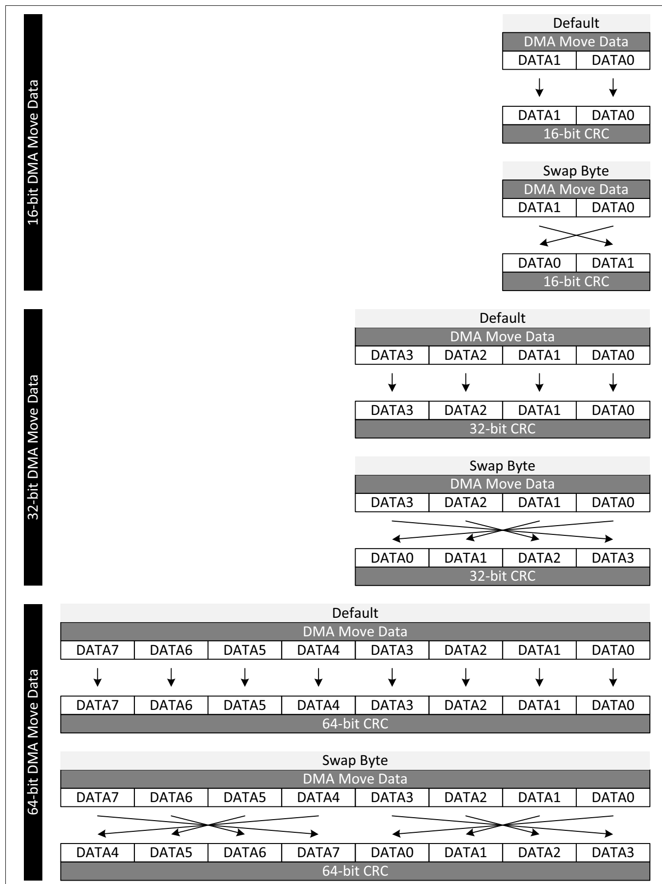
Figure 219 DMA Data Checksum - Swap Byte Order
