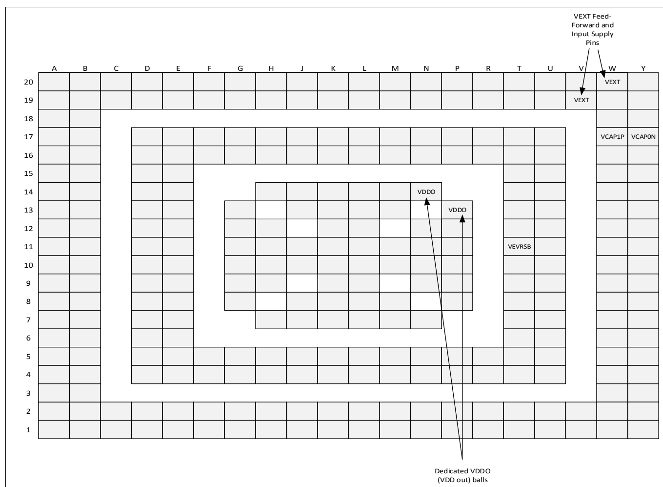
Figure 134 EVRC SC-DCDC Supply Pins for BGA Package (LFBGA292)
