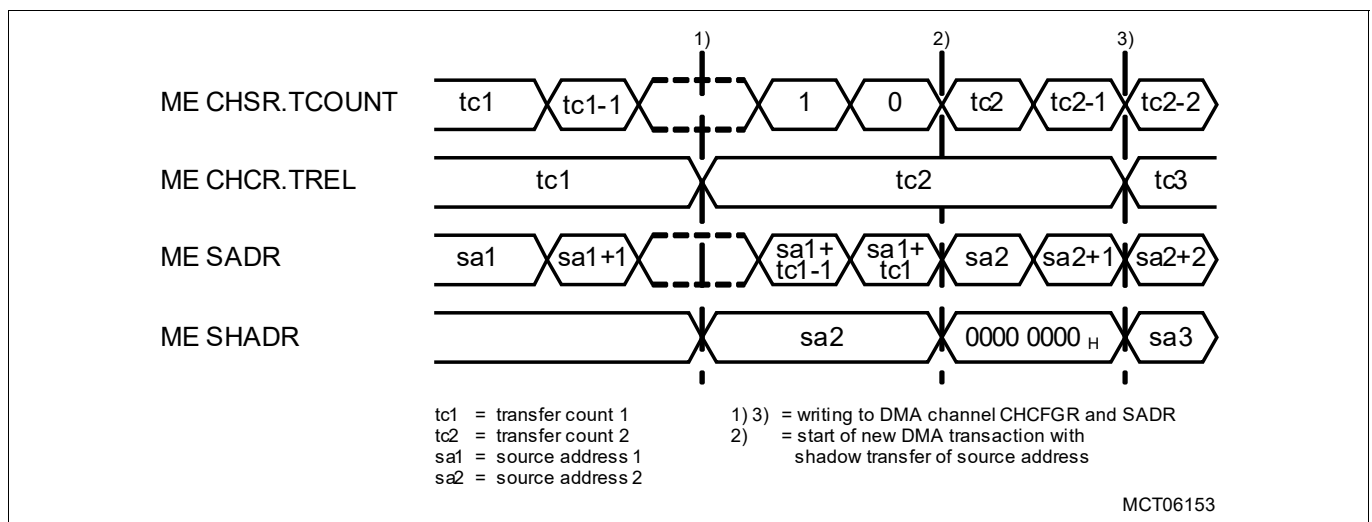
Figure 203 Shadow Operation Read Only Mode Source Address: Transfer Count and Source Address Update
