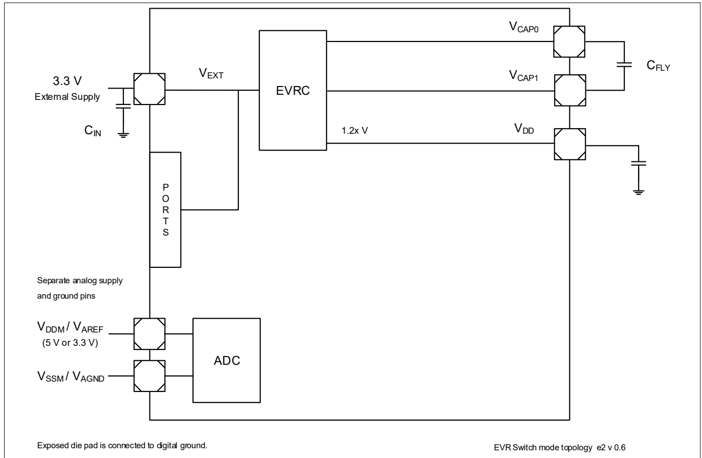
Figure 132 EVR Switch mode topology (e) - 3.3 V single supply
