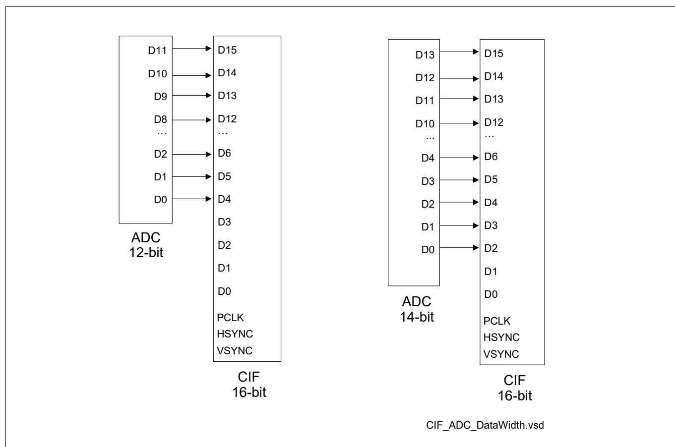
Figure 321 External ADC Data Alignment
