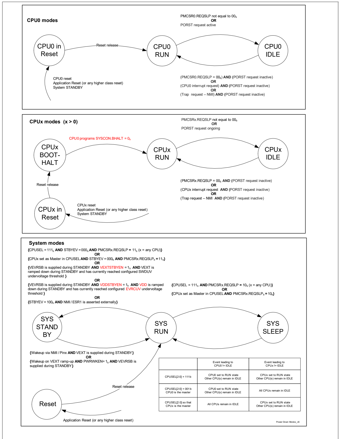
Figure 145 Power down modes and transitions
