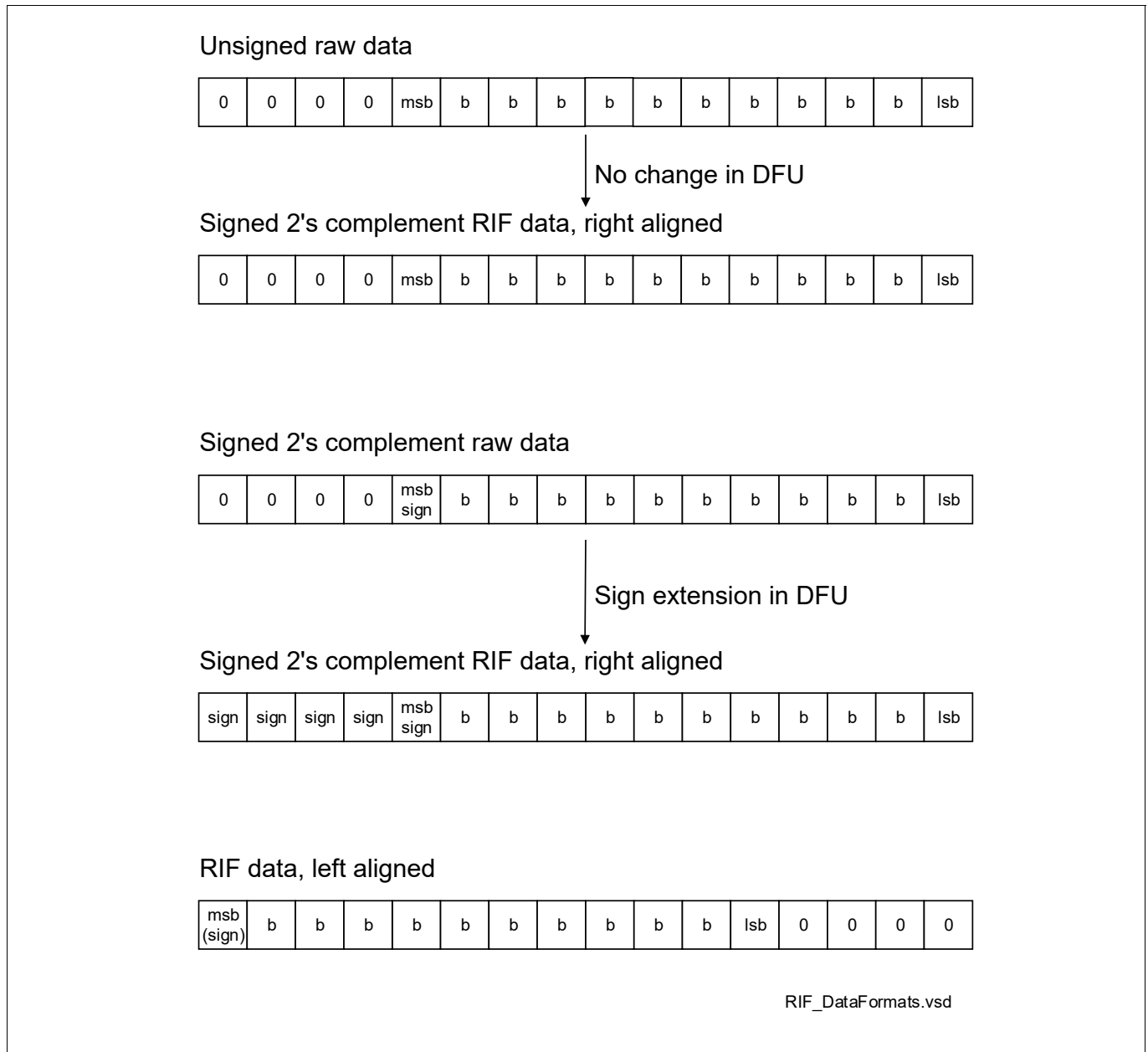
Figure 277 DFU Processing of the Data Formats
