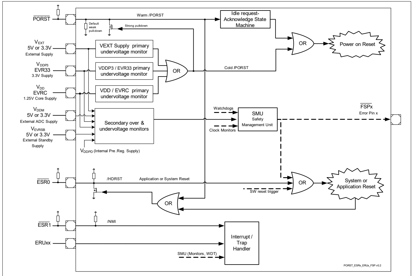
Figure 110 Monitoring and Reset Pins
