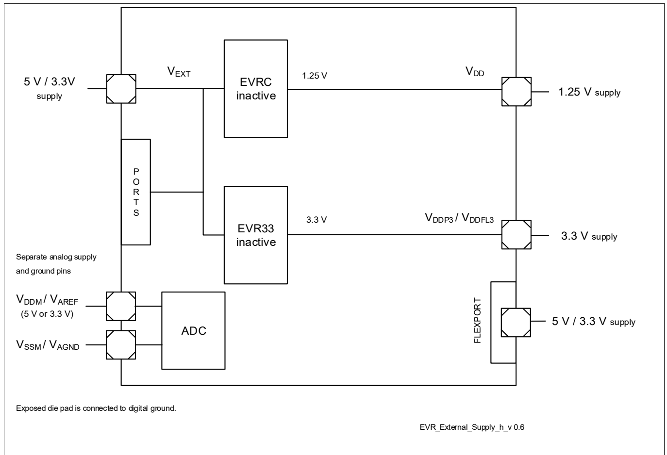
Figure 138 External Supply mode (h) - VEXT, VDDP3 and VDD externally supplied
