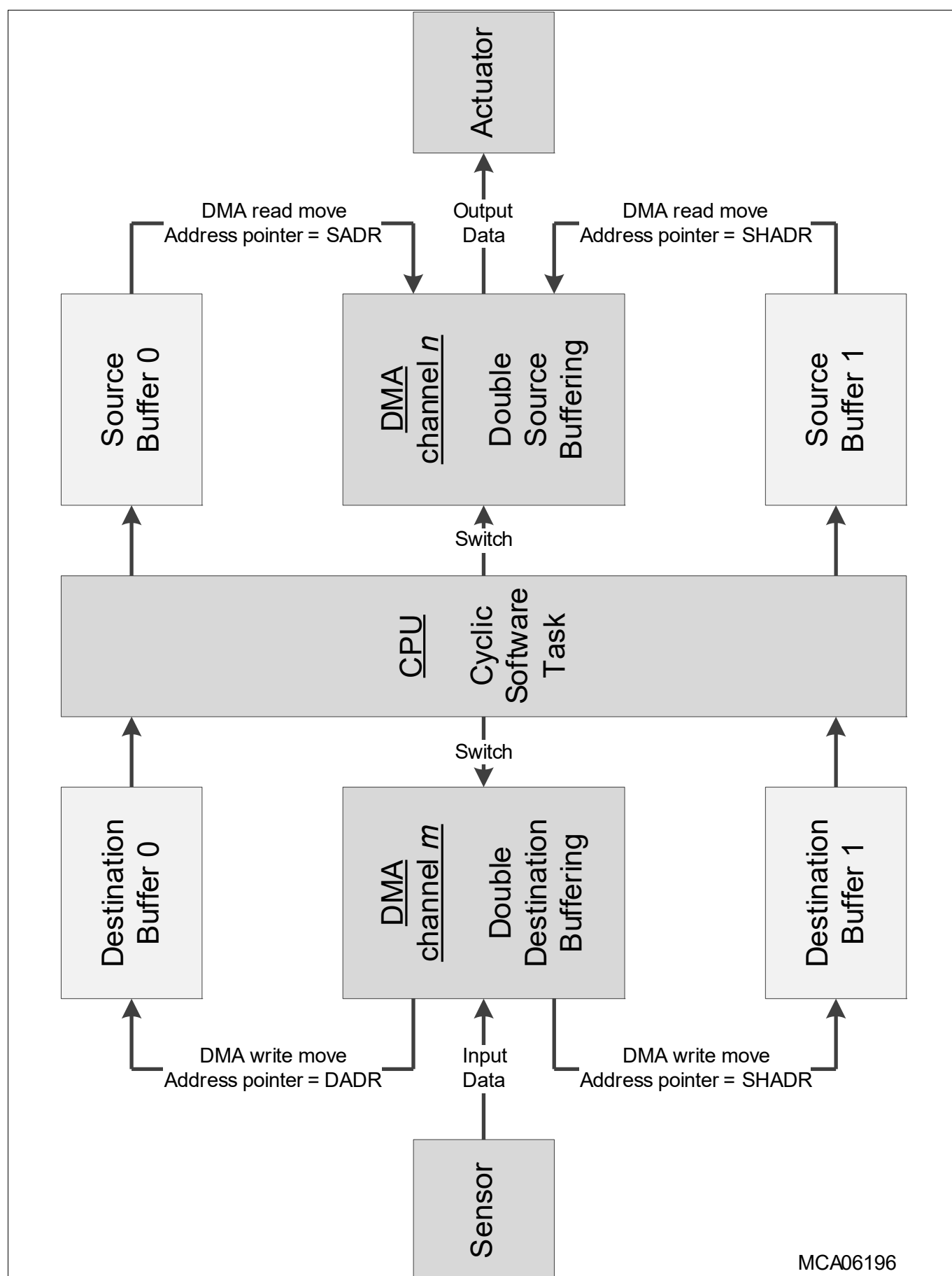
Figure 212 Application of Double Buffering
