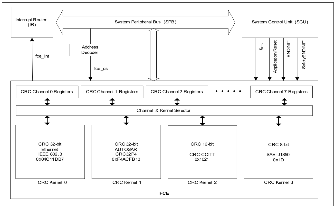
Figure 179 FCE Block Diagram
