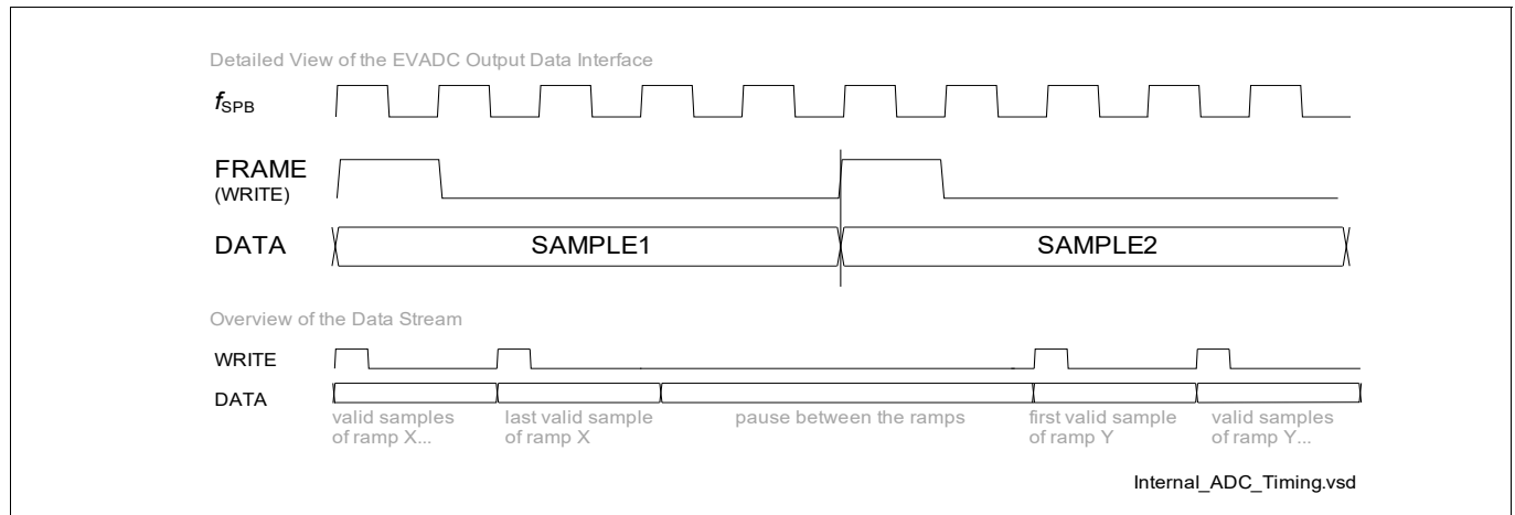
Figure 269 Waveforms of the Internal Parallel Interface to the internal ADC
