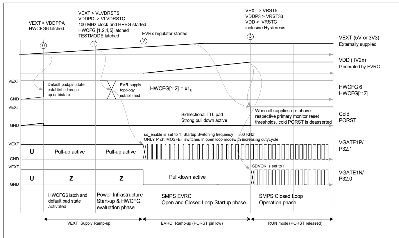
Figure 99 VGATE behavior during start-up when EVRC regulator is used
