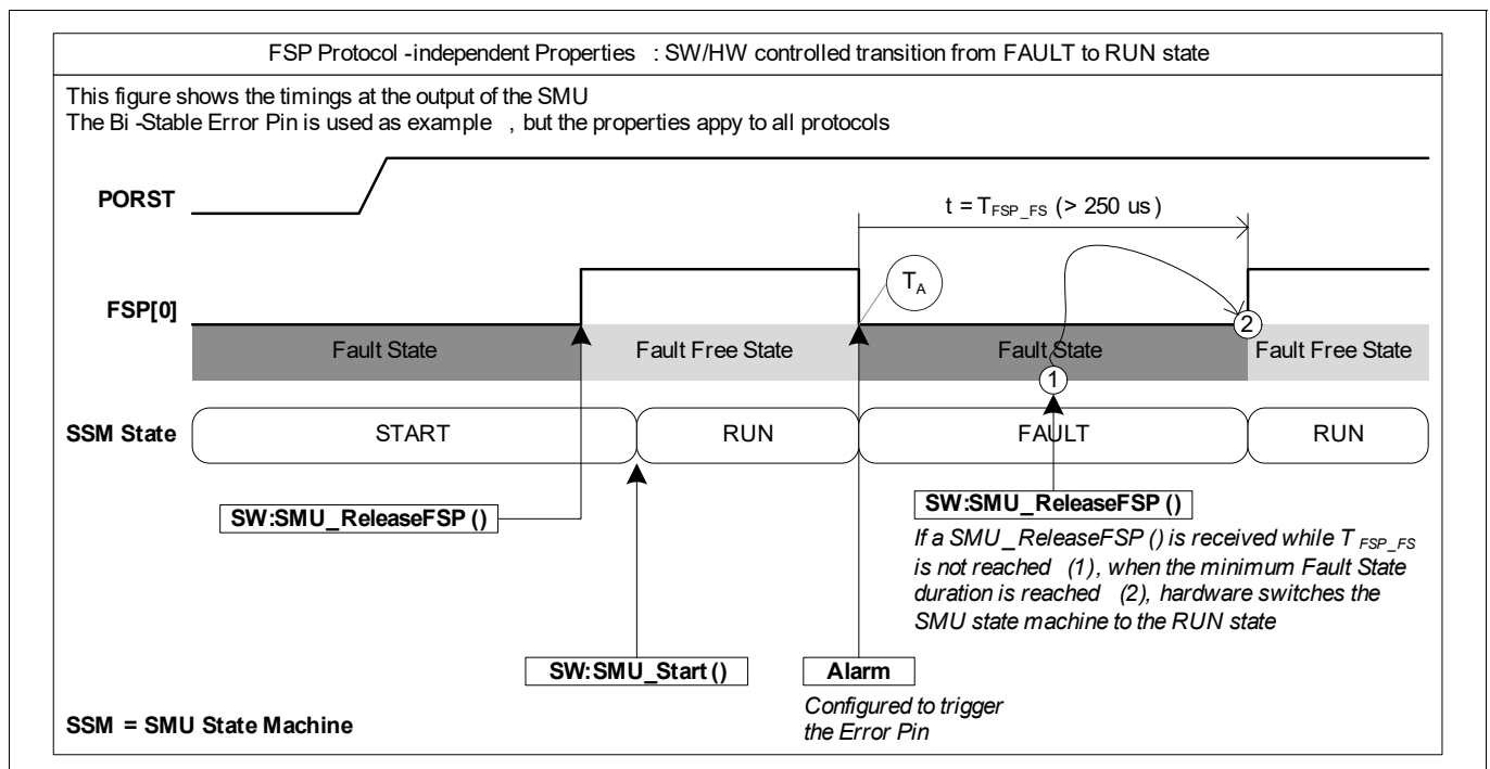
Figure 167 FSP: Fault State to Fault Free State Transition
