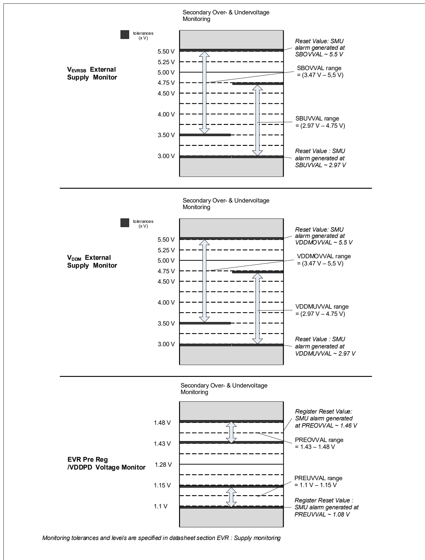
Figure 112 Voltage Monitoring - VEVRSB, VDDM &amp; VDDPD
