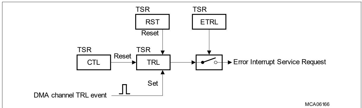
Figure 193 DMA Channel Transaction Request Lost Interrupt Service Request
