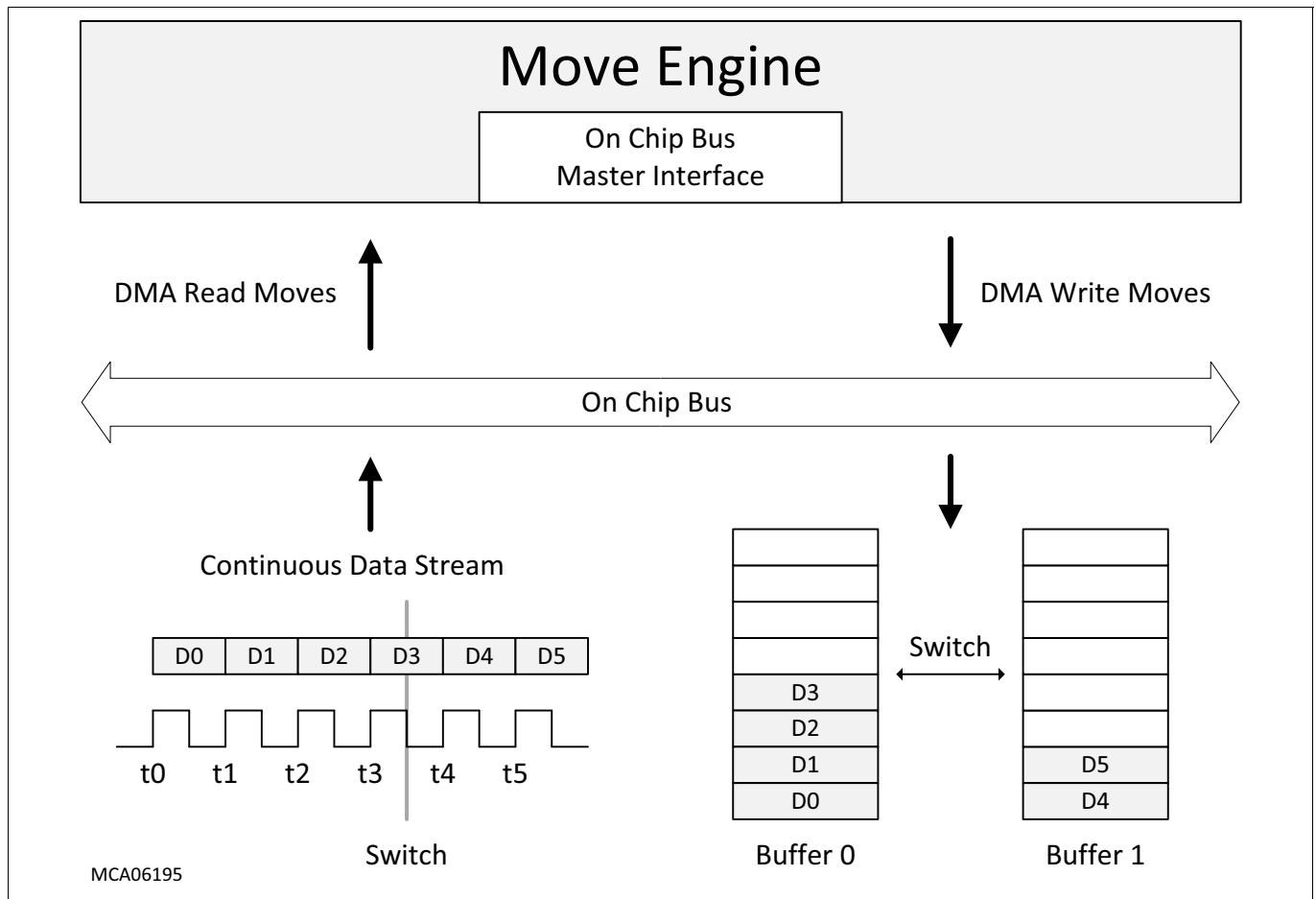
Figure 211 DMA Double Buffering
