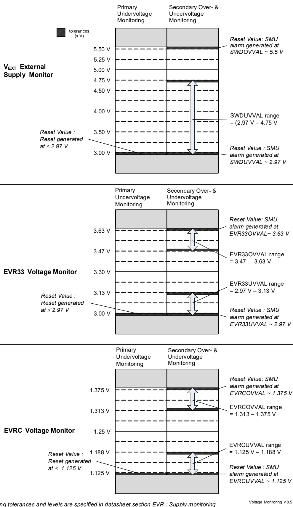
Figure 111 Voltage Monitoring - VEXT, VDDP3 &amp; VDD
