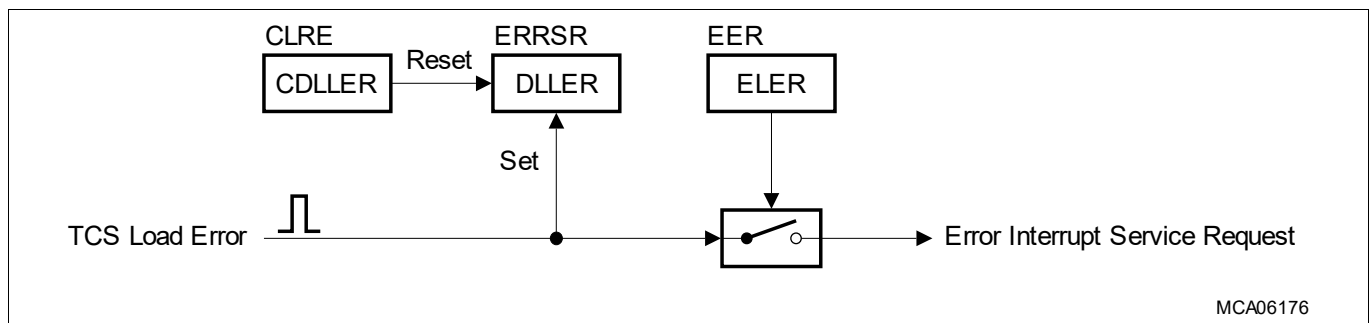
Figure 221 Linked List Operation TCS Error Interrupt Service Request
