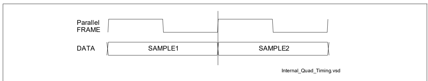
Figure 270 Waveforms of the Internal Parallel Interface to the Quad Deserializer
