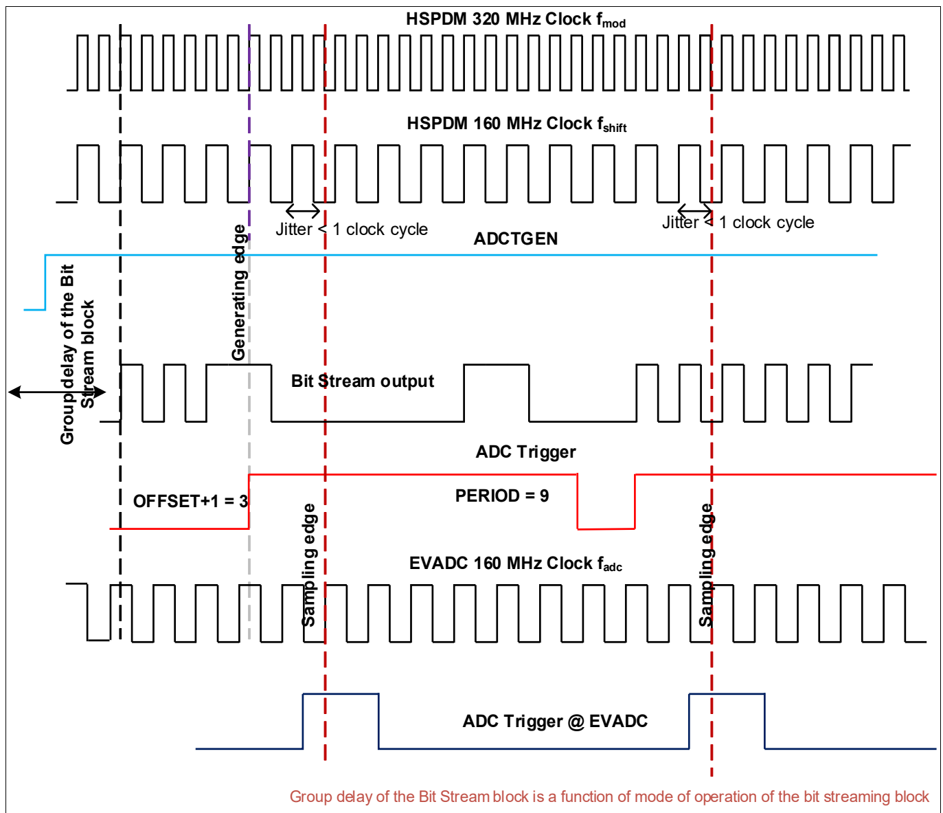
Figure 310 ADC Trigger Concept
