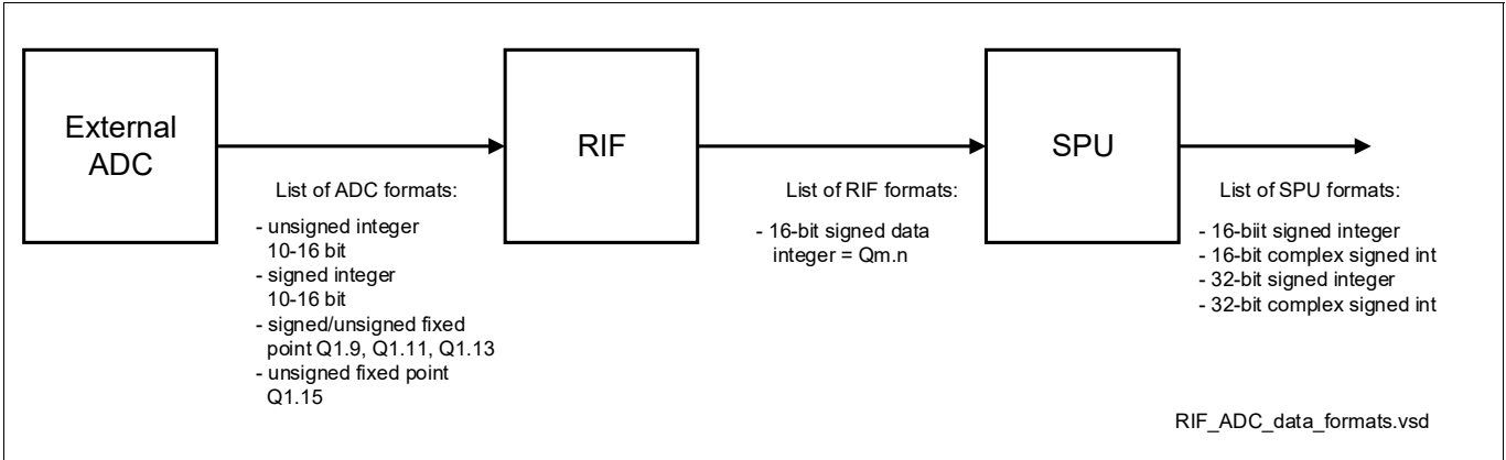
Figure 275 Data Formats from the External ADC
