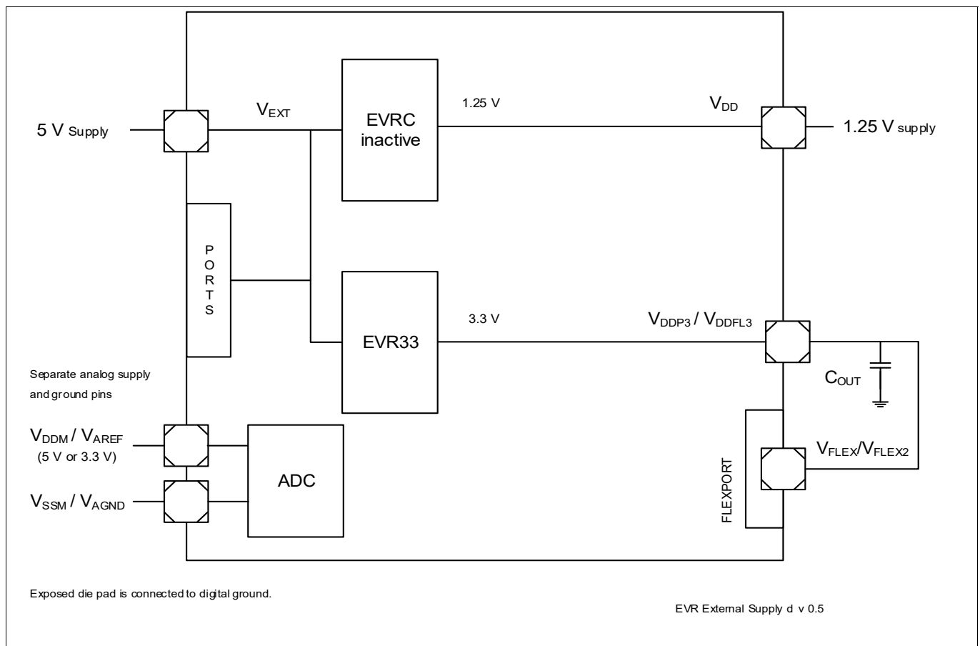
Figure 137 External Supply mode (d) - V_{EXT} and V_{DD} externally supplied
