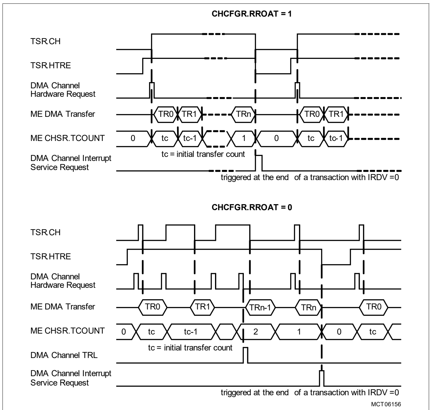
Figure 191 Hardware Control in Single Mode
