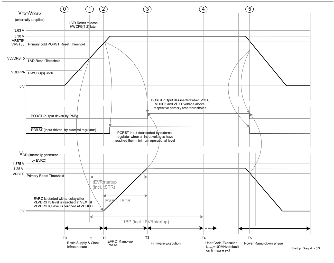
Figure 124 Single Supply mode (e) - ( V_{EXT} & V_{DDP3} ) 3.3 V single supply
