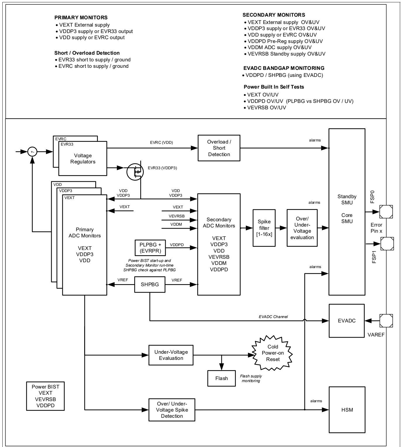
Figure 139 Supply Monitor Overview
