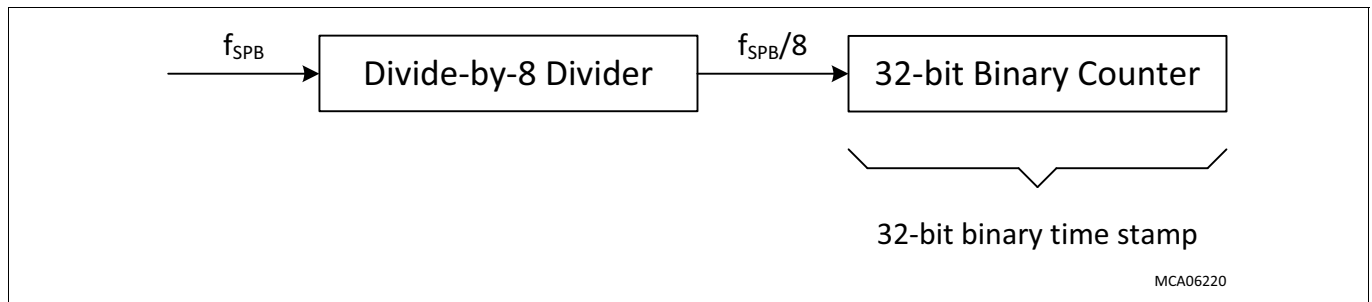
Figure 204 Generation of DMA Timestamp
