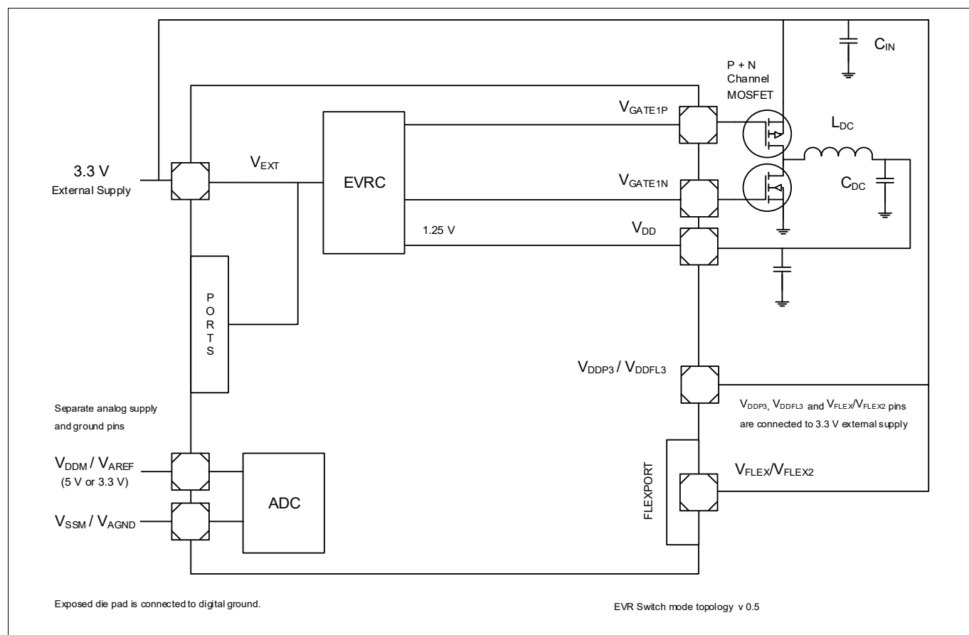
Figure 104 EVR Switch mode topology (e) - 3.3 V single supply
