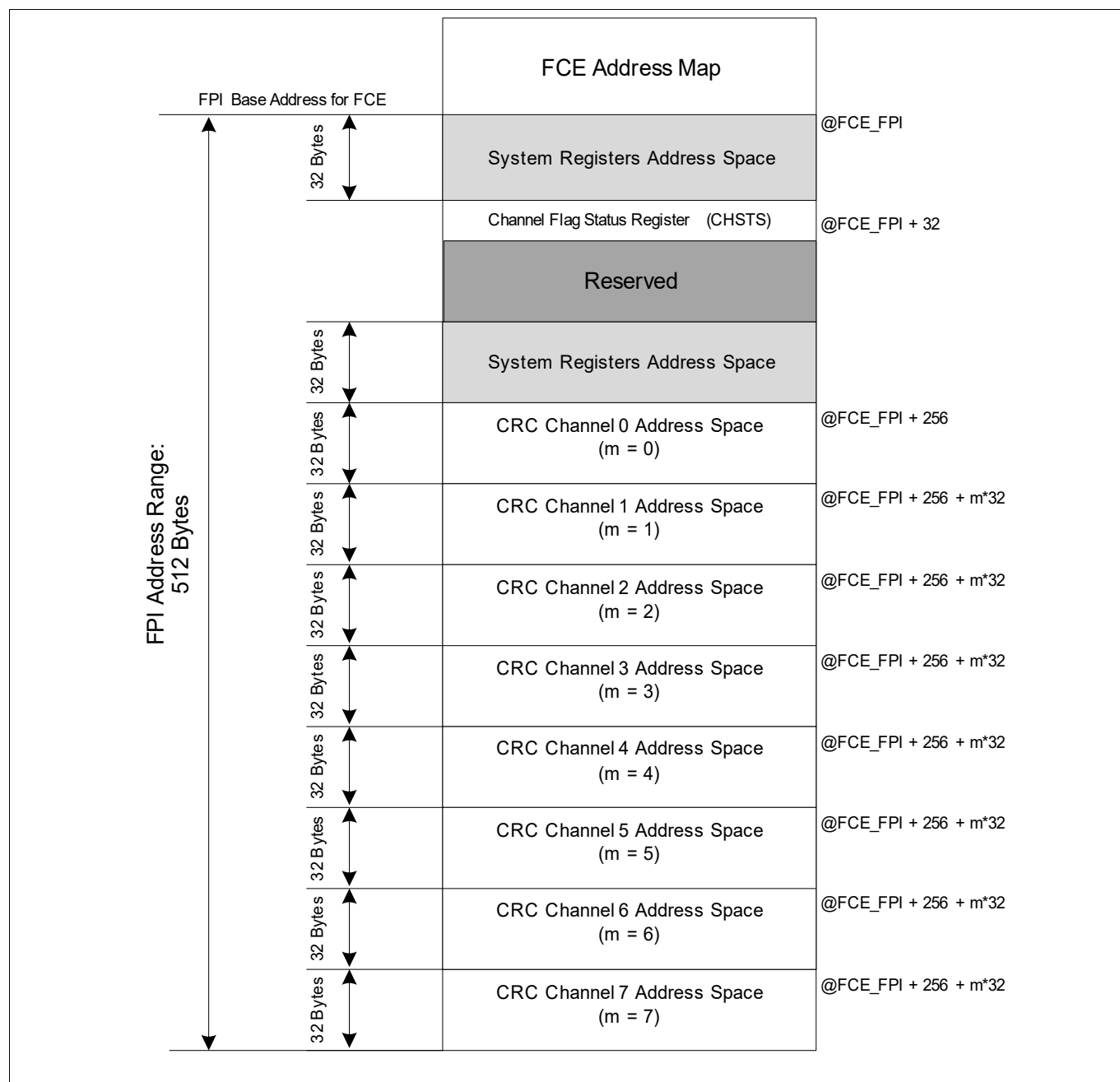
Figure 187 FCE Registers Address Map
