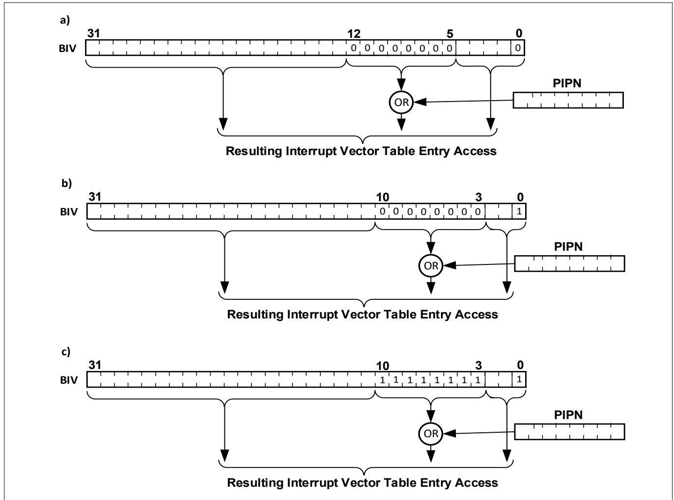
Figure 177 Interrupt Vector Table Address Calculation for a) 32 Byte b) 8 Byte vector entry or c) single entry
