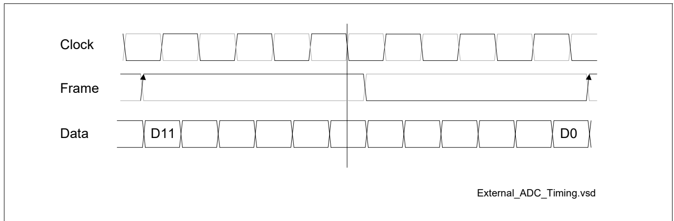
Figure 267 Waveforms of the External Serial Interface, Detailed View
