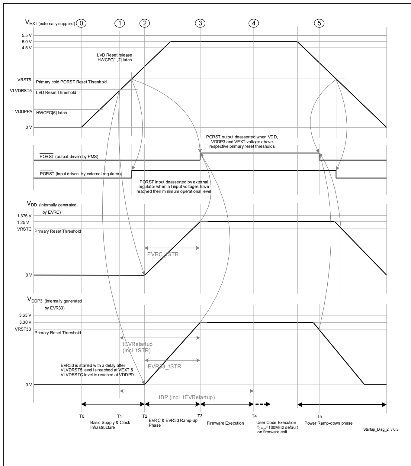
Figure 123 Single Supply mode (a) - VEXT (5 V) single supply
