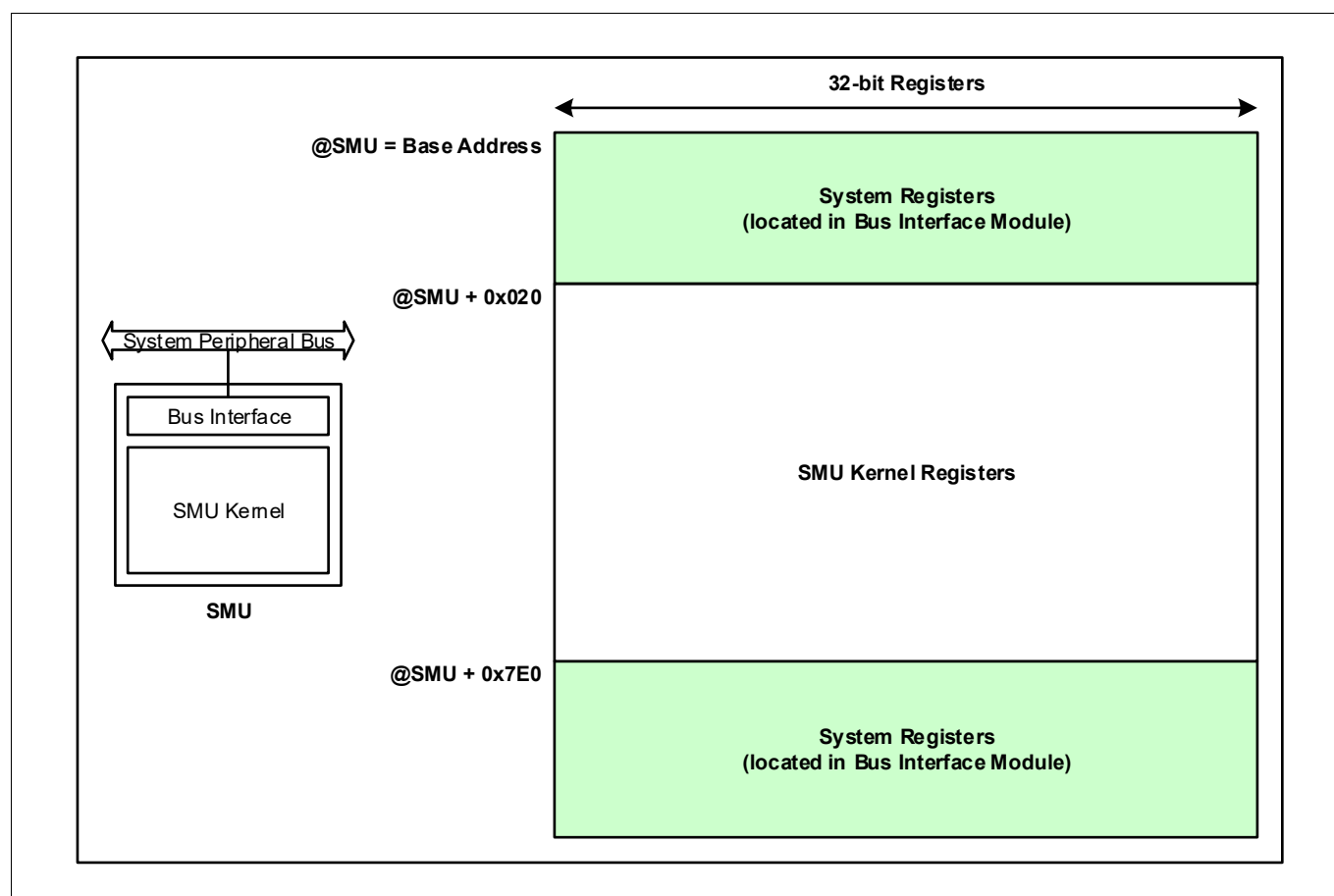
Figure 170 SMU_core
