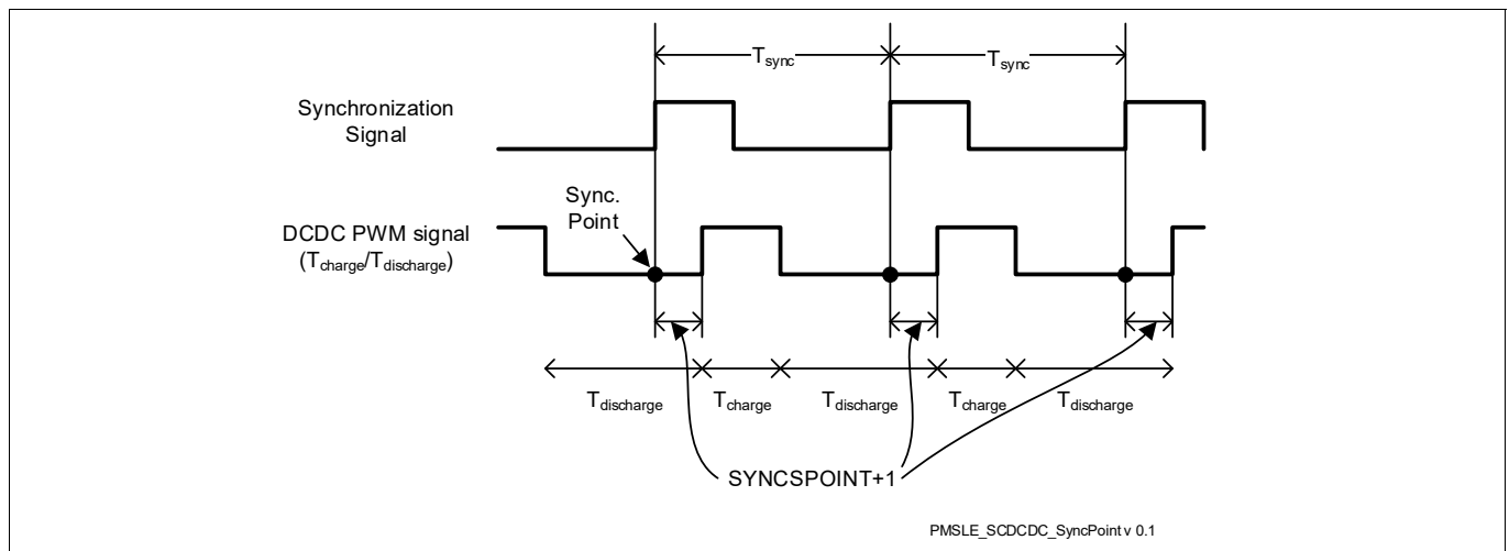
Figure 136 Synchronization Point between External Synchronization Signal and DCDC PWM Signal
