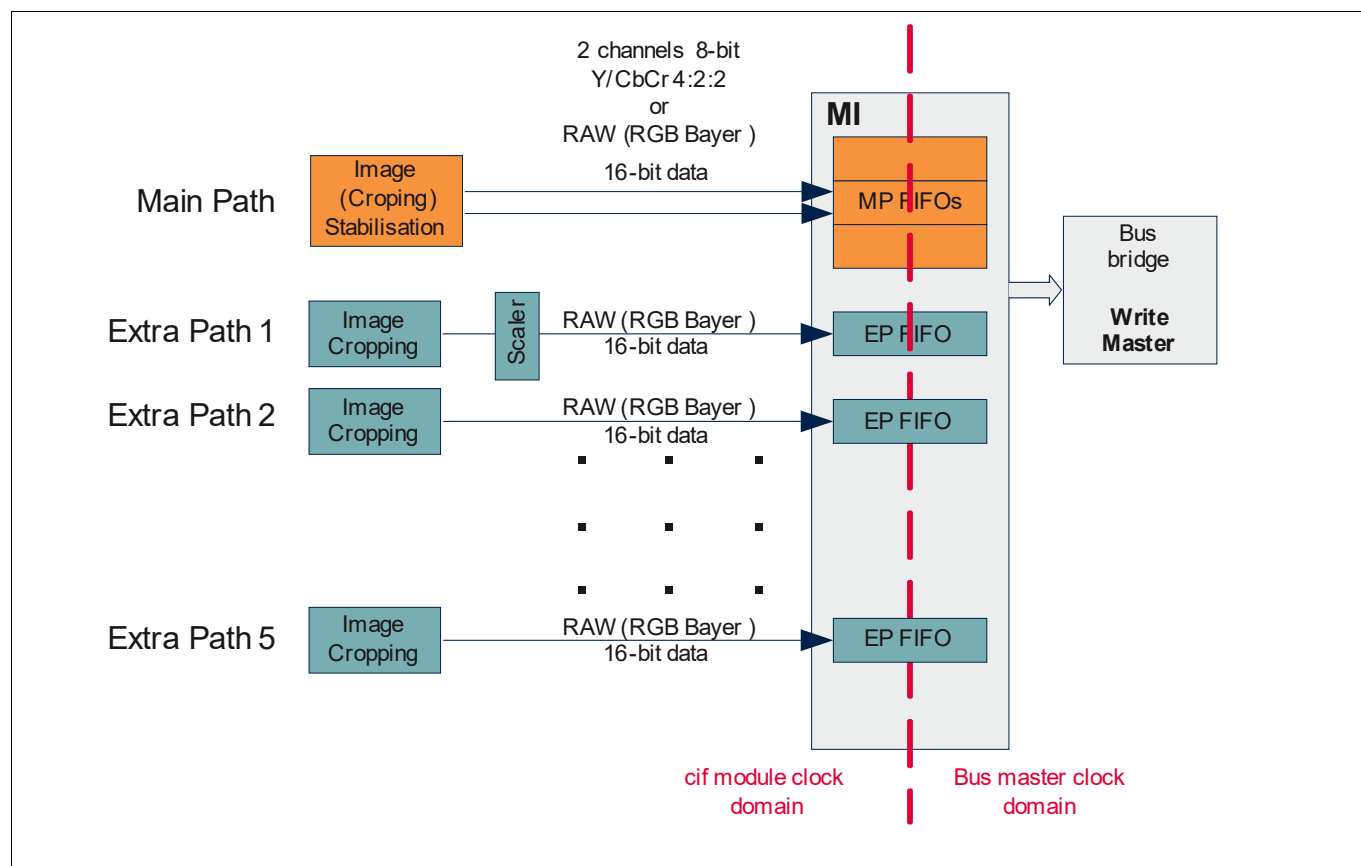
Figure 332 Overview Memory Interface connections
