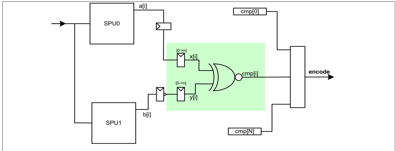
Figure 258 Node Comparator
