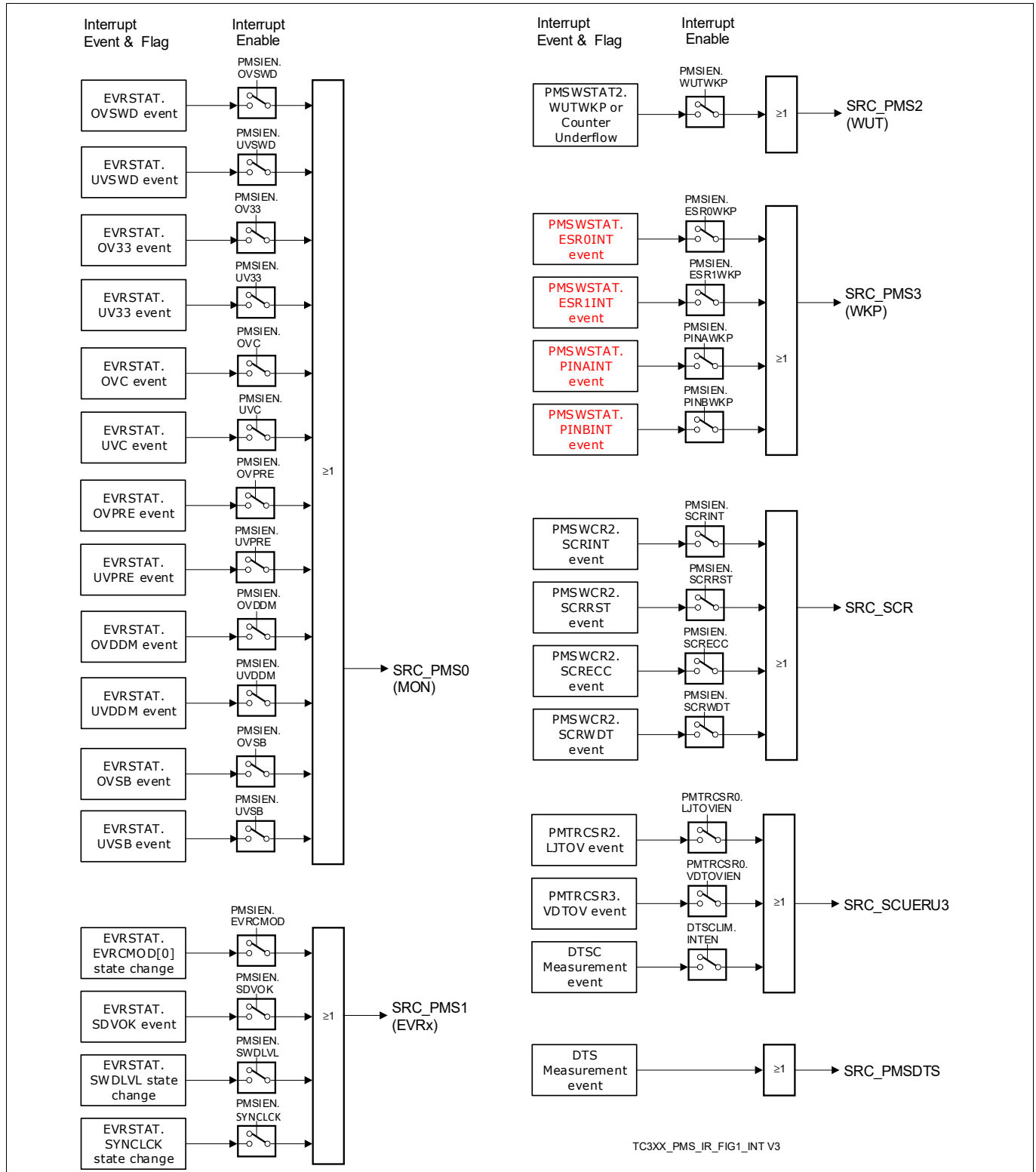
Figure 113 Interrupt Sources and Events
