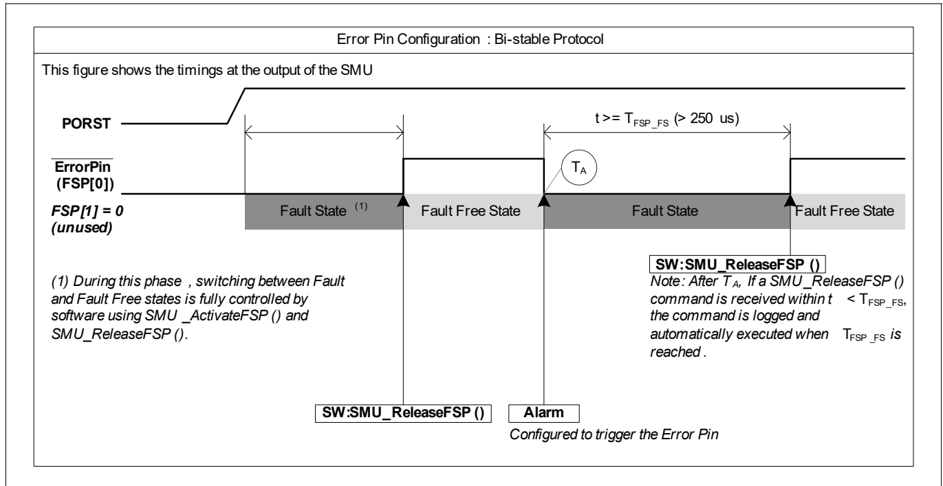
Figure 164 Bi-stable fault signaling protocol
