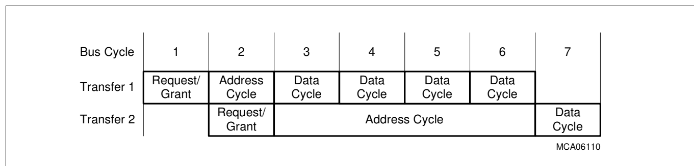
Figure 36 FPI Bus Block Transactions
