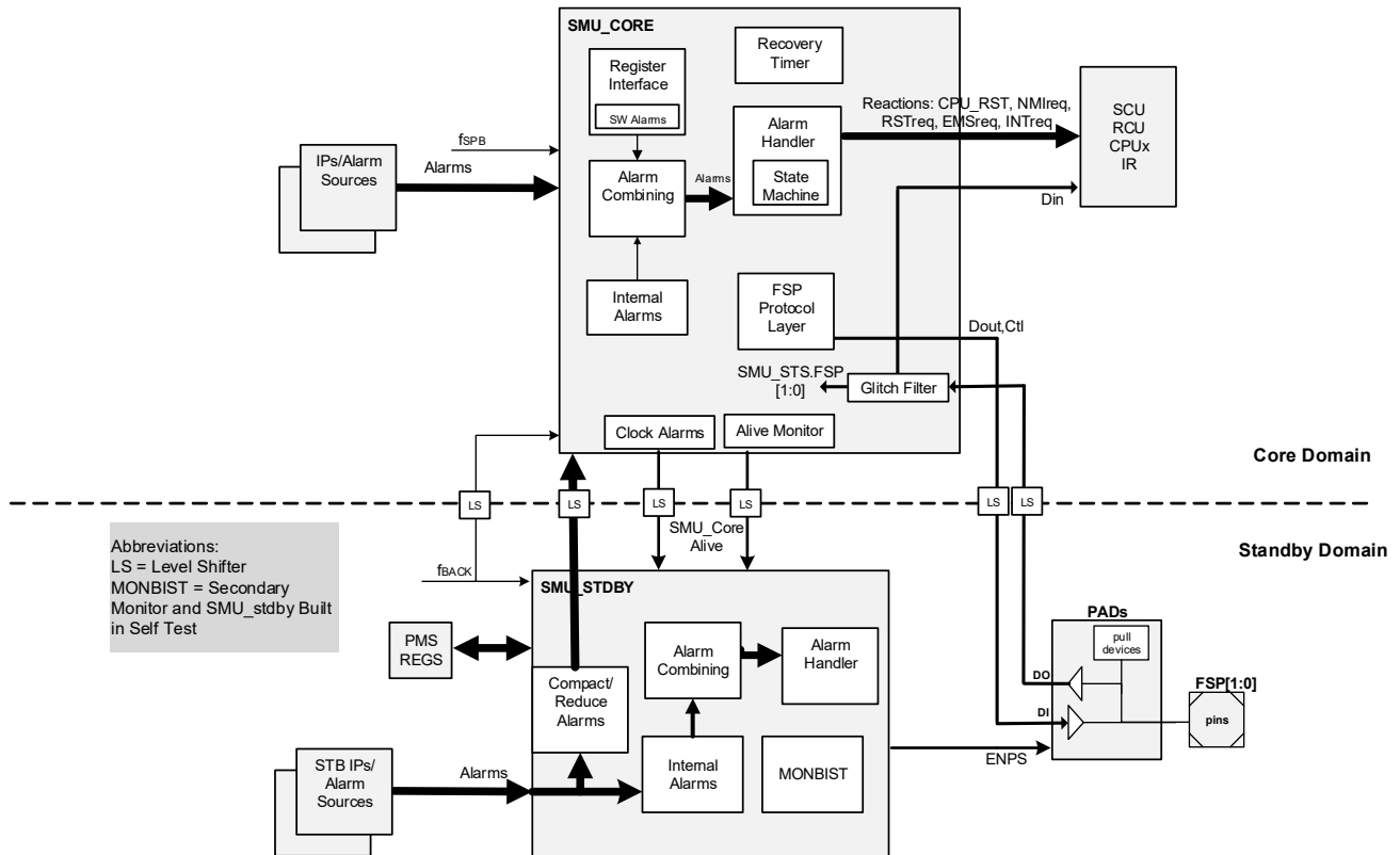
Figure 157 SMU Architecture
