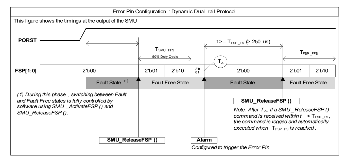
Figure 165 Dynamic dual-rail fault signaling protocol
