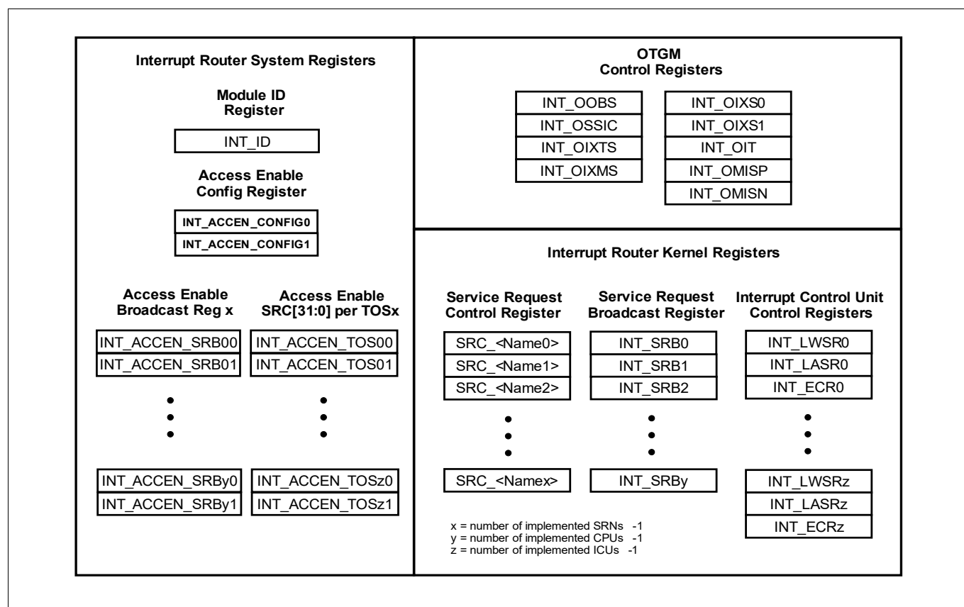
Figure 178 Interrupt Router module registers
