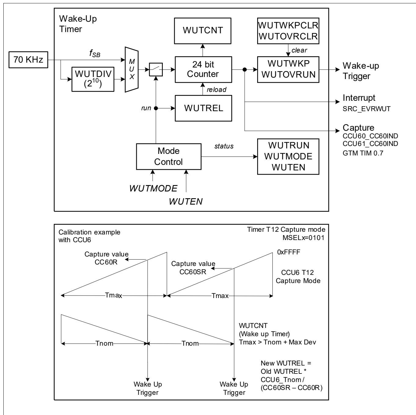
Figure 117 Wake-up Timer (WUT)
