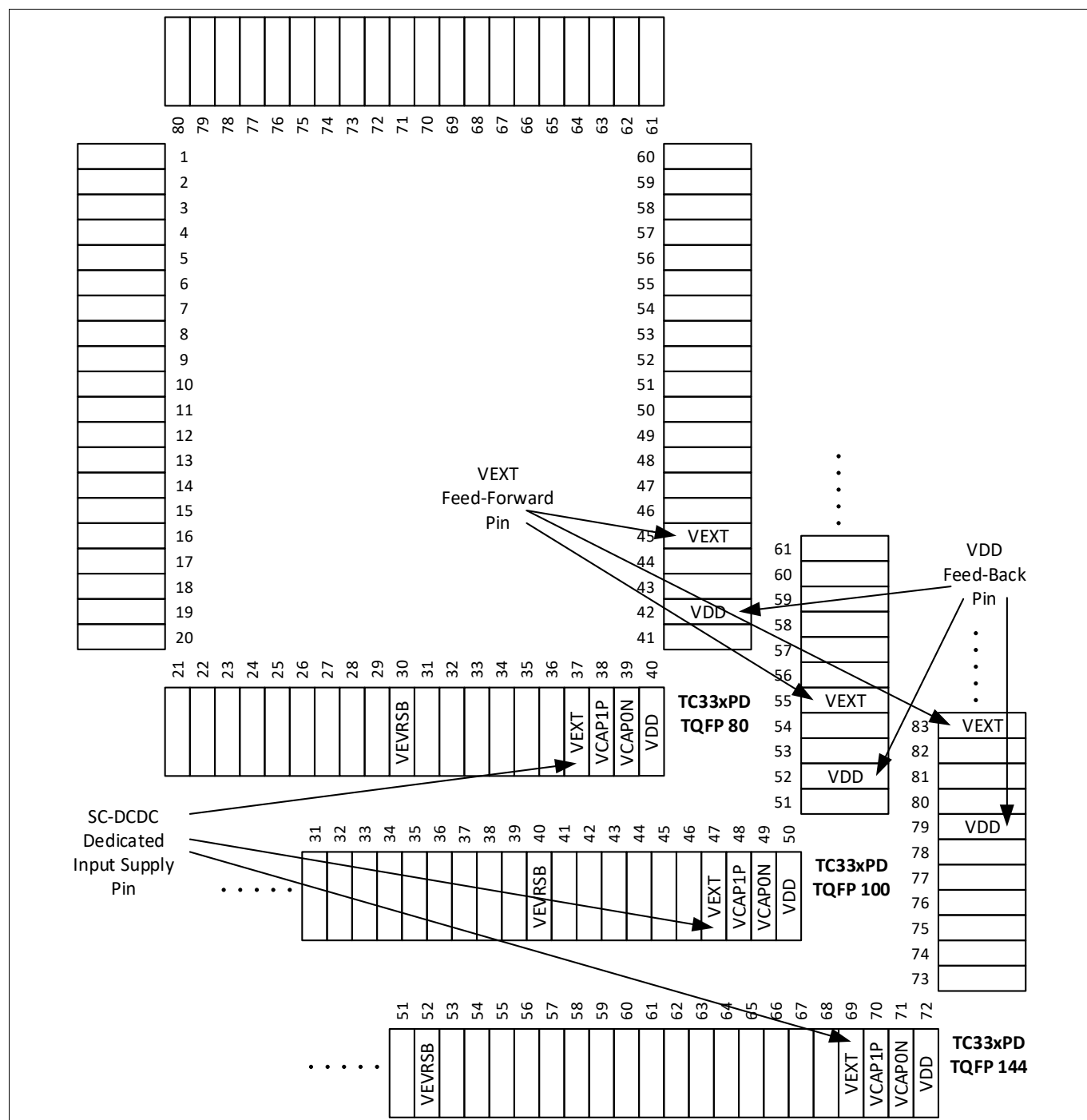
Figure 133 EVRC SC-DCDC Supply Pins for QFP Packages
