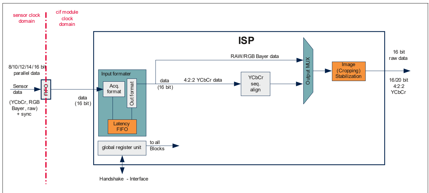
Figure 323 Block Diagram of the ISP Sub Module
