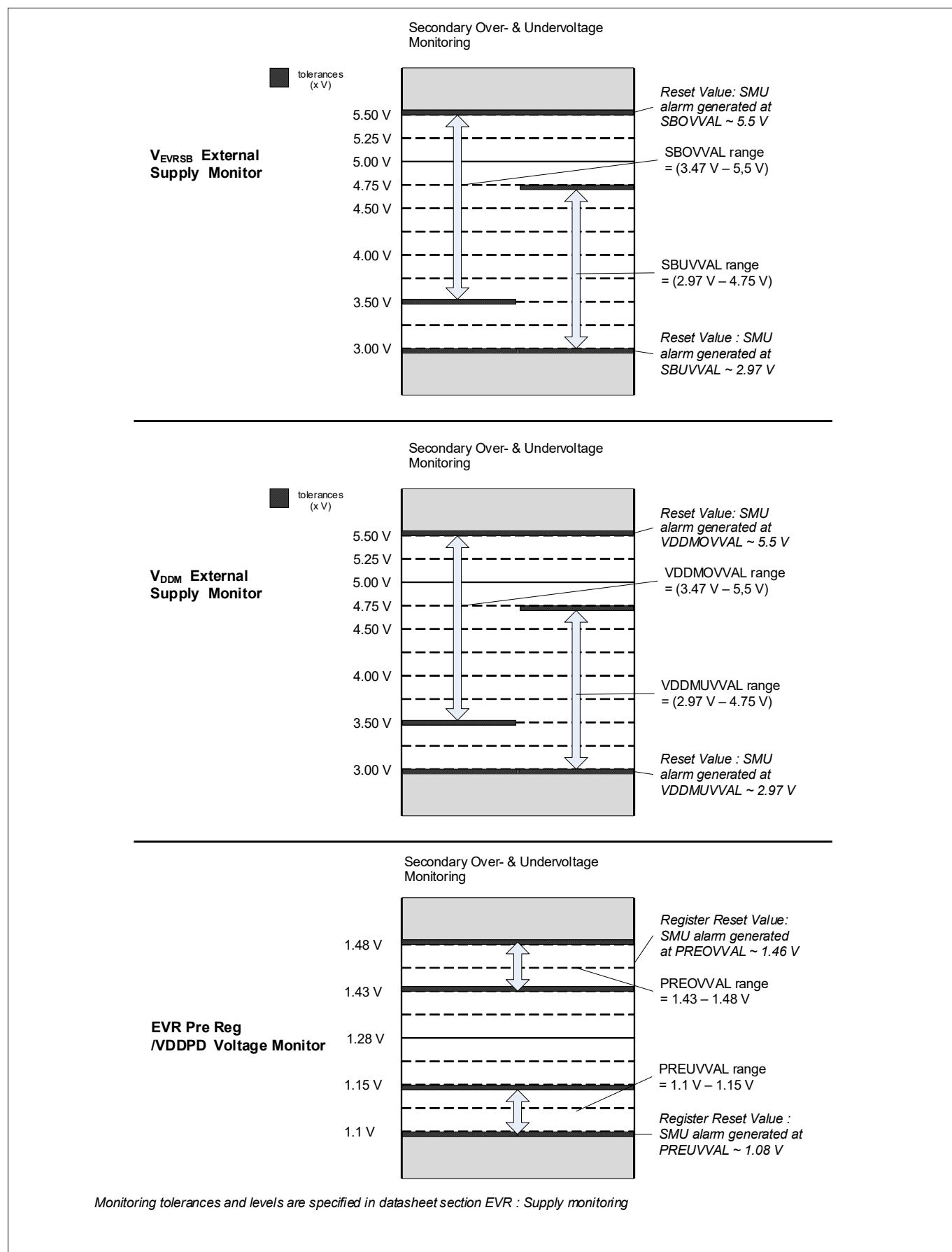
Figure 143 Voltage Monitoring - VEVRSB, VDDM &amp; VDDPD
