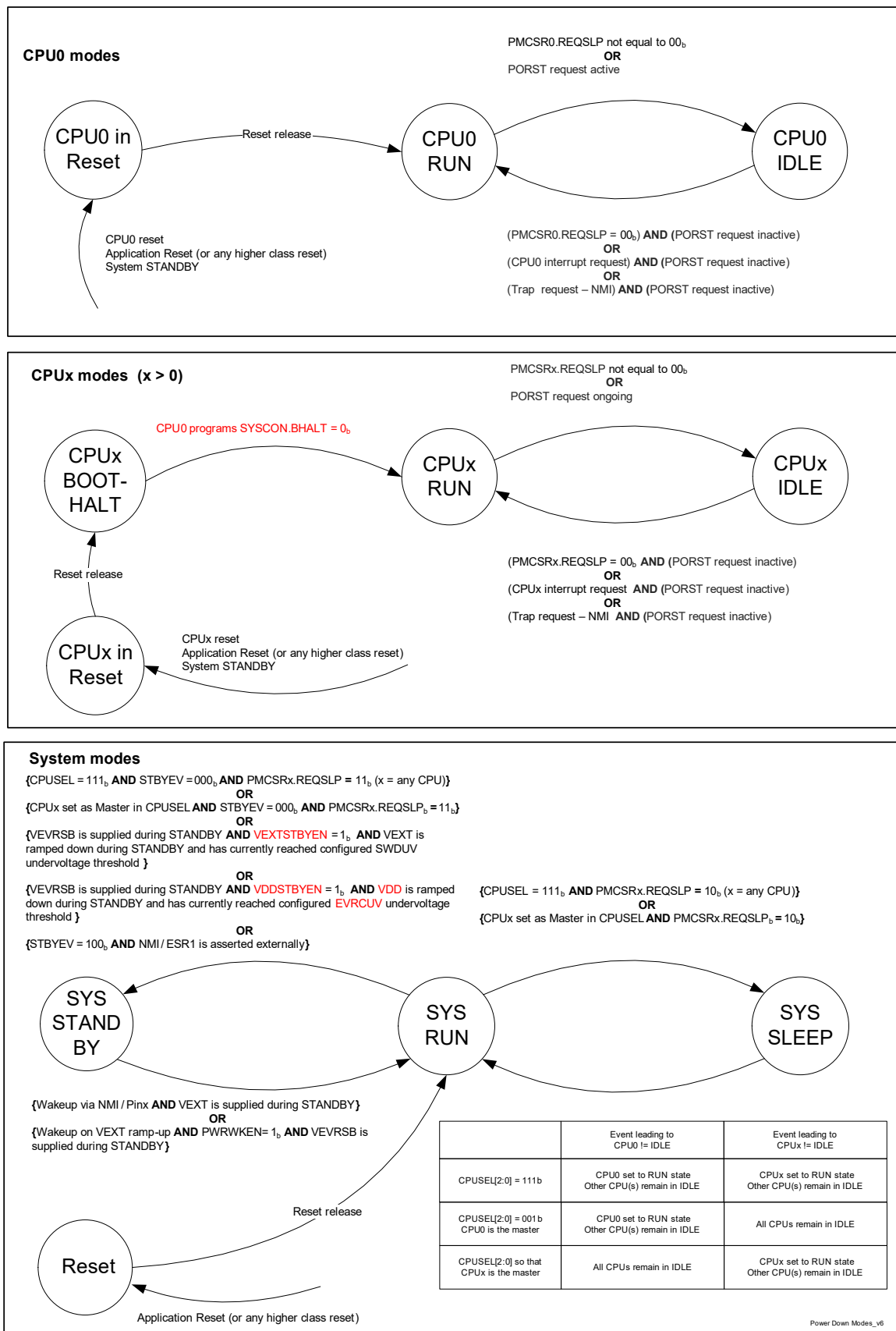
Figure 114 Power down modes and transitions
