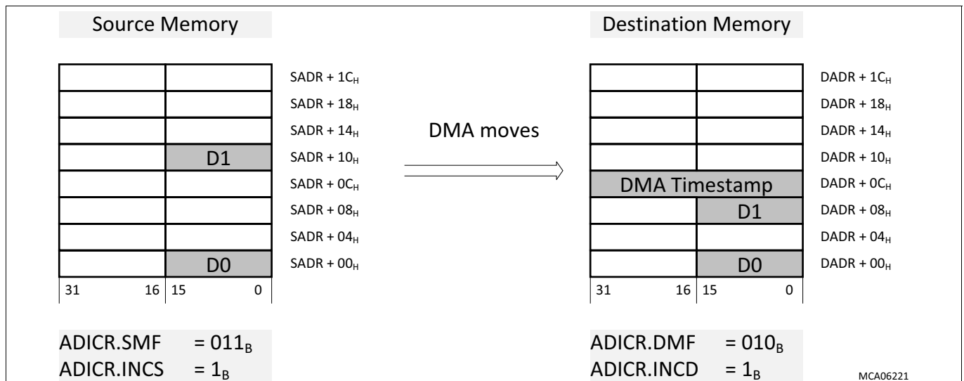
Figure 205 Incrementing Destination Address: DMA Timestamp appended above DMA Write Move Data
