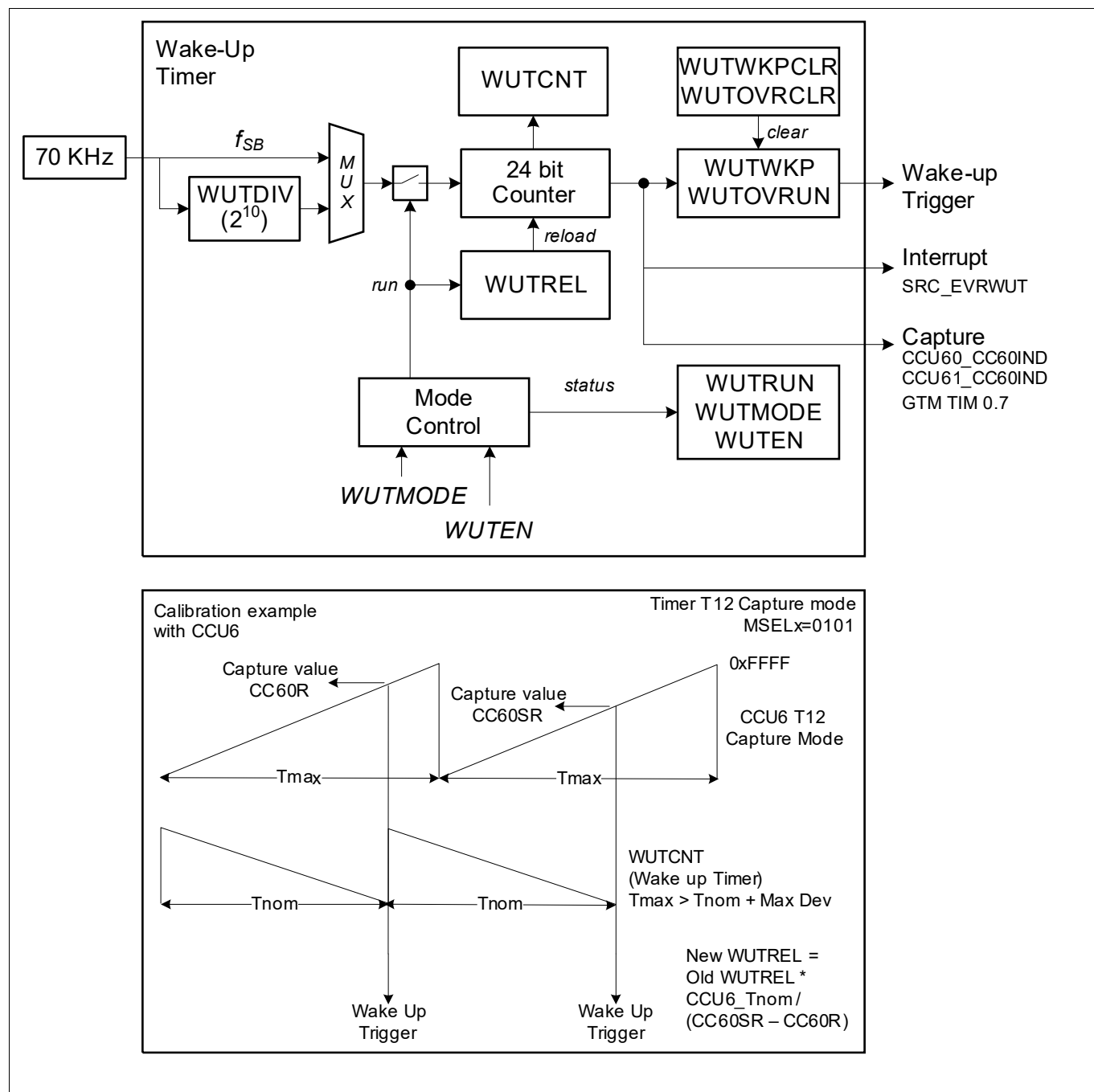
Figure 148 Wake-up Timer (WUT)
