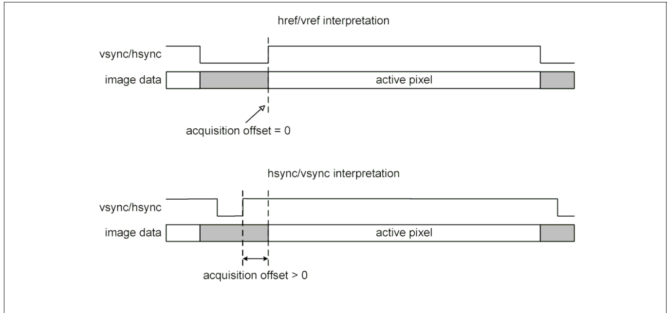
Figure 345 Reference and Synchronization Signals for ITU-R BT 601 Mode
