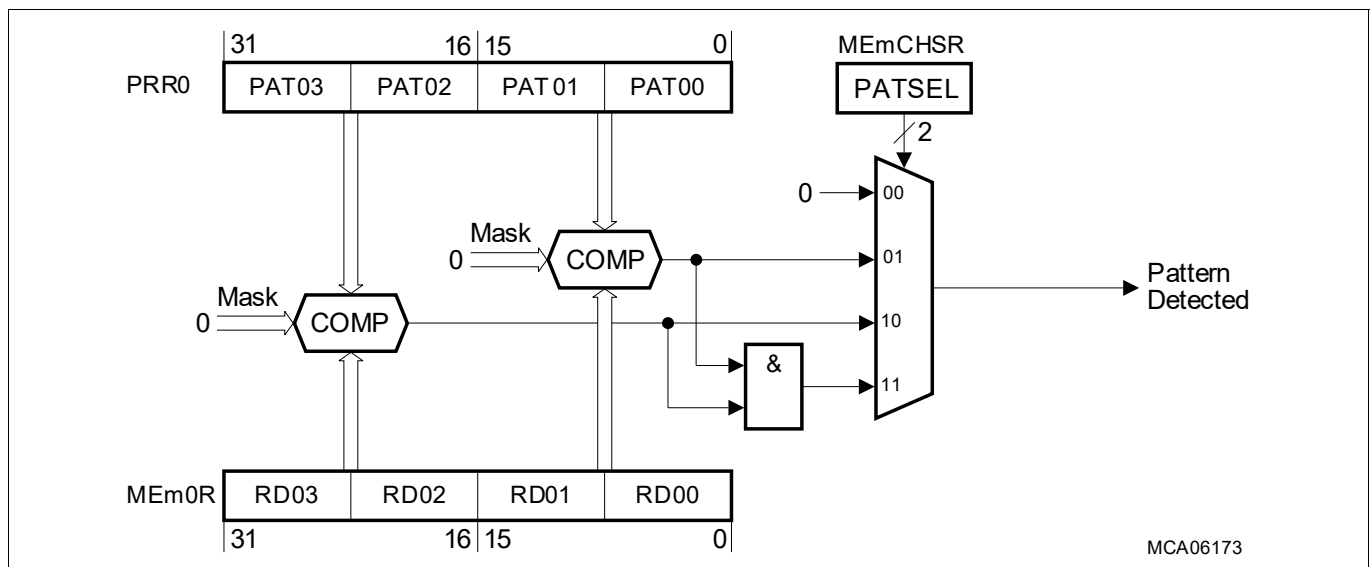
Figure 210 PATDET for 32-bit Channel Data Width and Move Data stored in MEm0R
