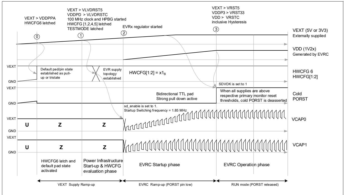
Figure 127 VCAP behavior during start-up when EVRC regulator is used
