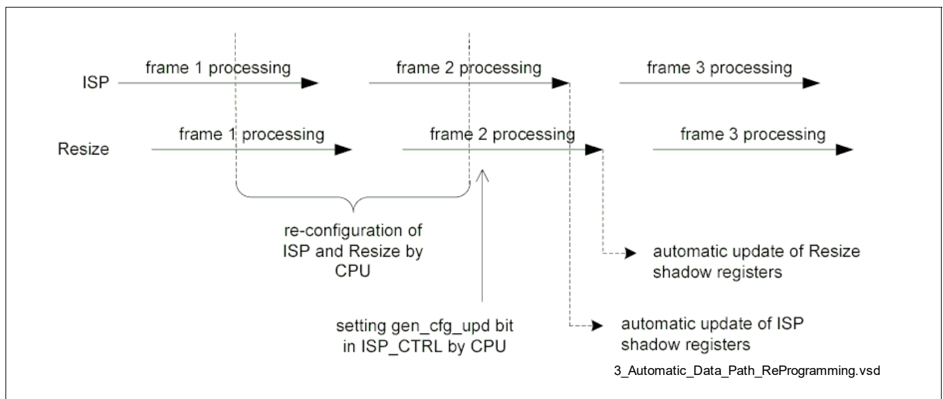
Figure 338 Automatic Data Path Re-Programming
