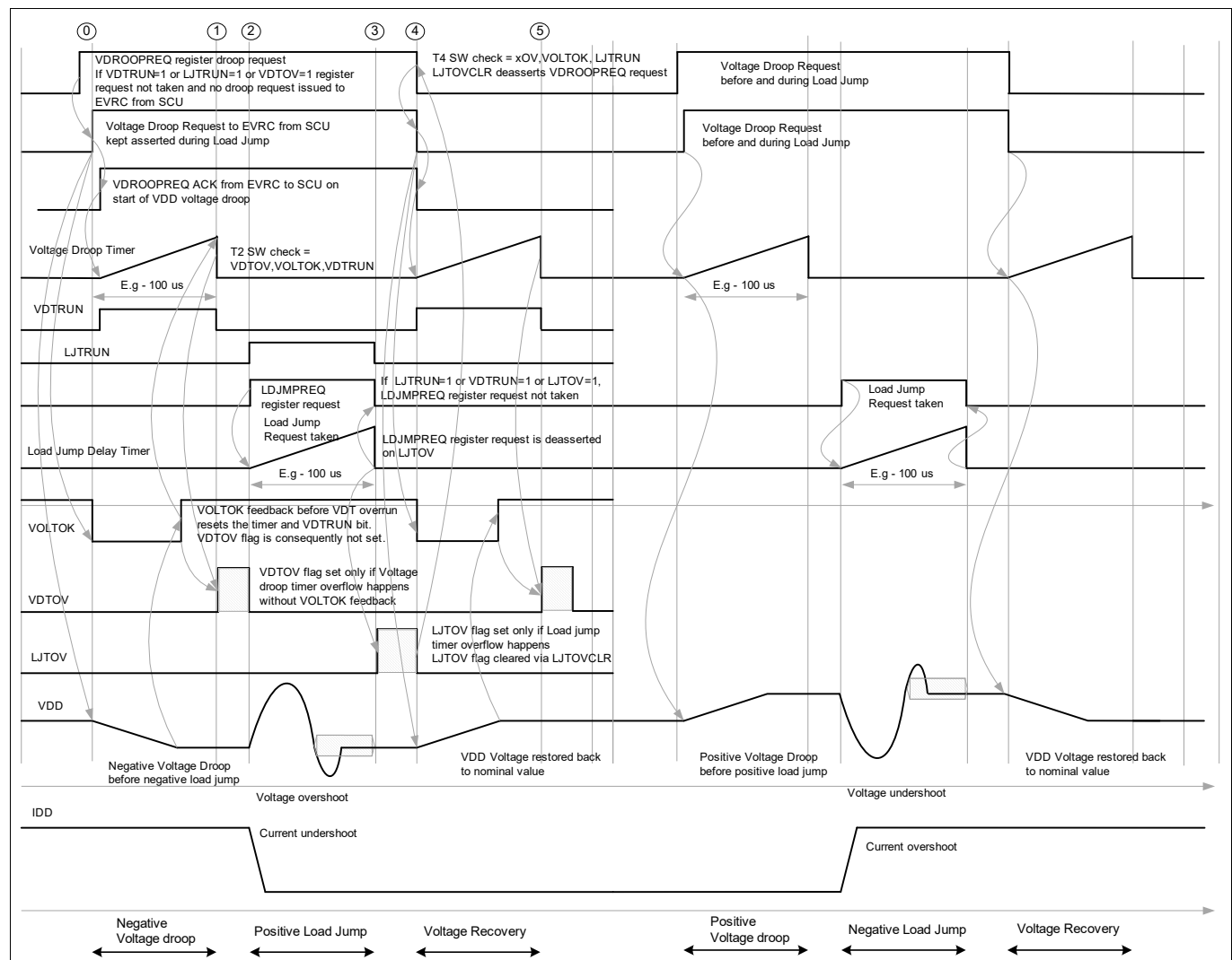
Figure 151 Load jumps and Voltage Droop
