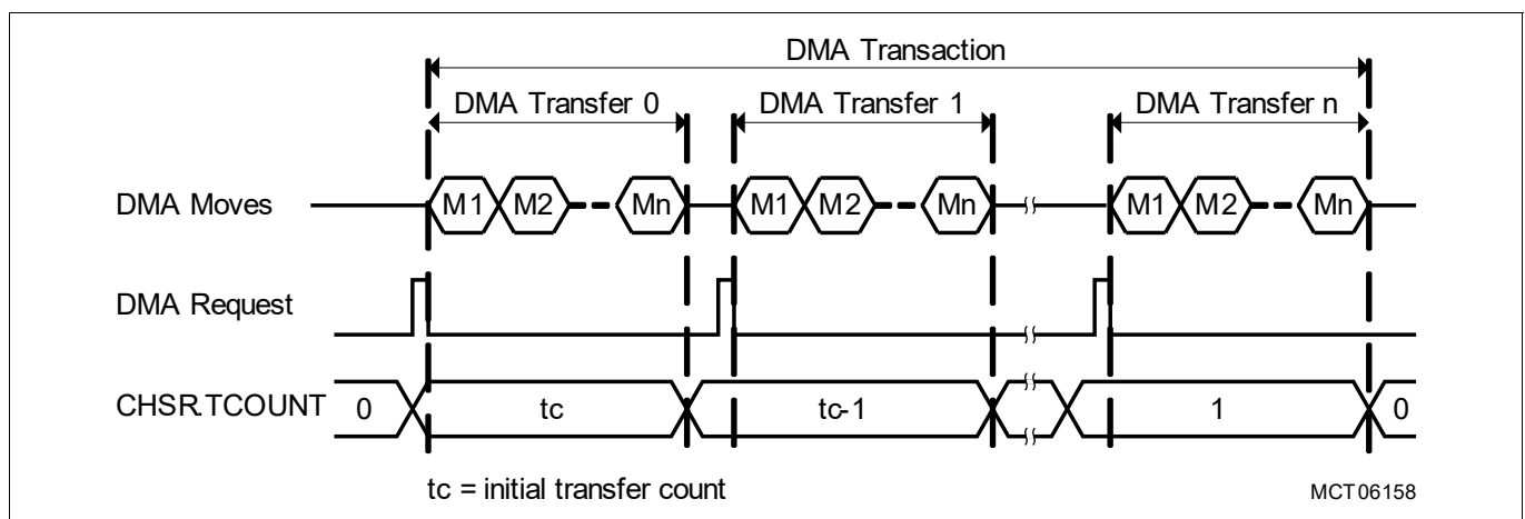
Figure 197 Block Mode and Transfer Count
