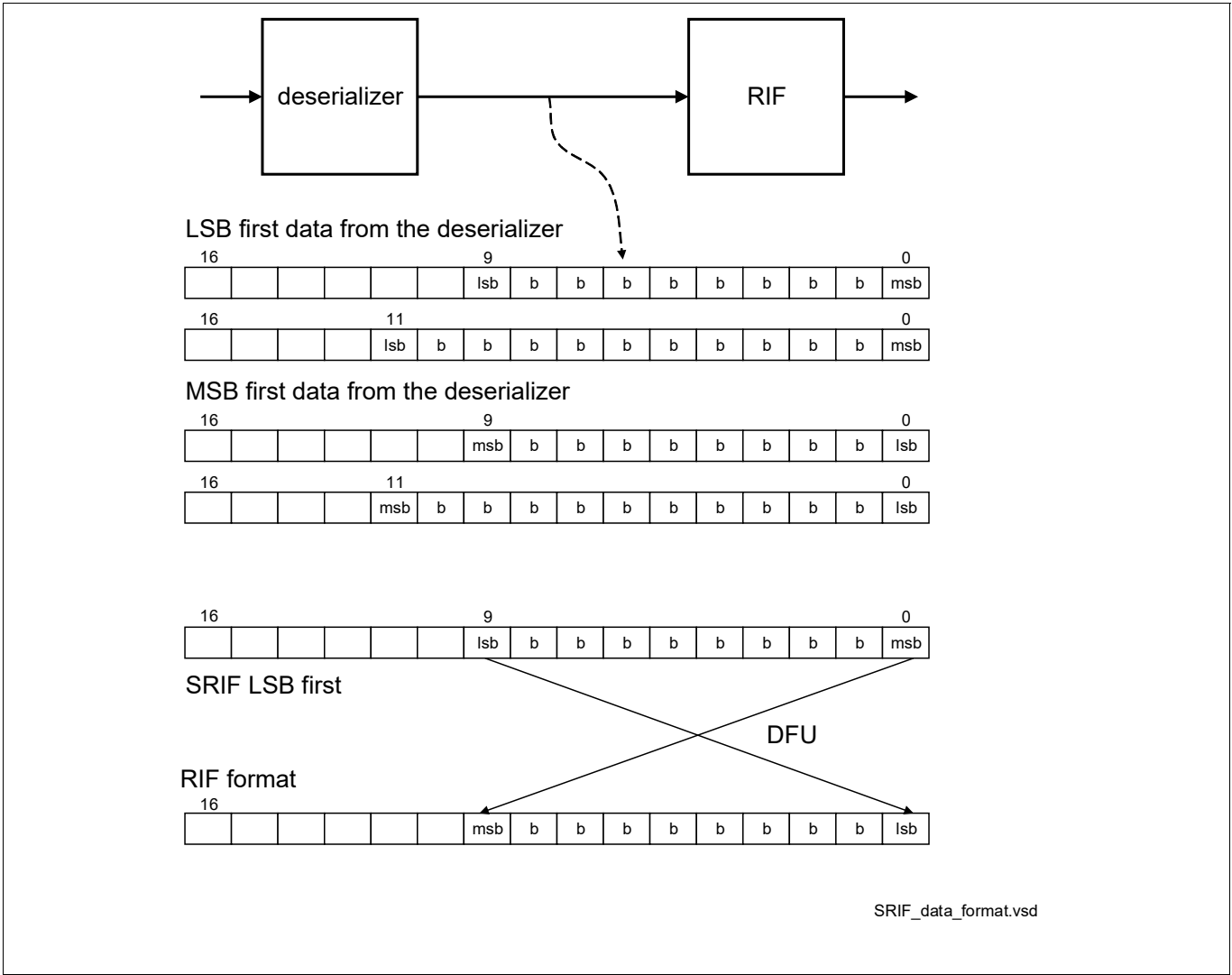
Figure 276 Shift Direction Management
