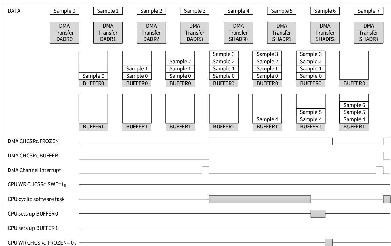
Figure 214 DMA Double Destination Buffering Software Switch and Automatic Hardware Switch
