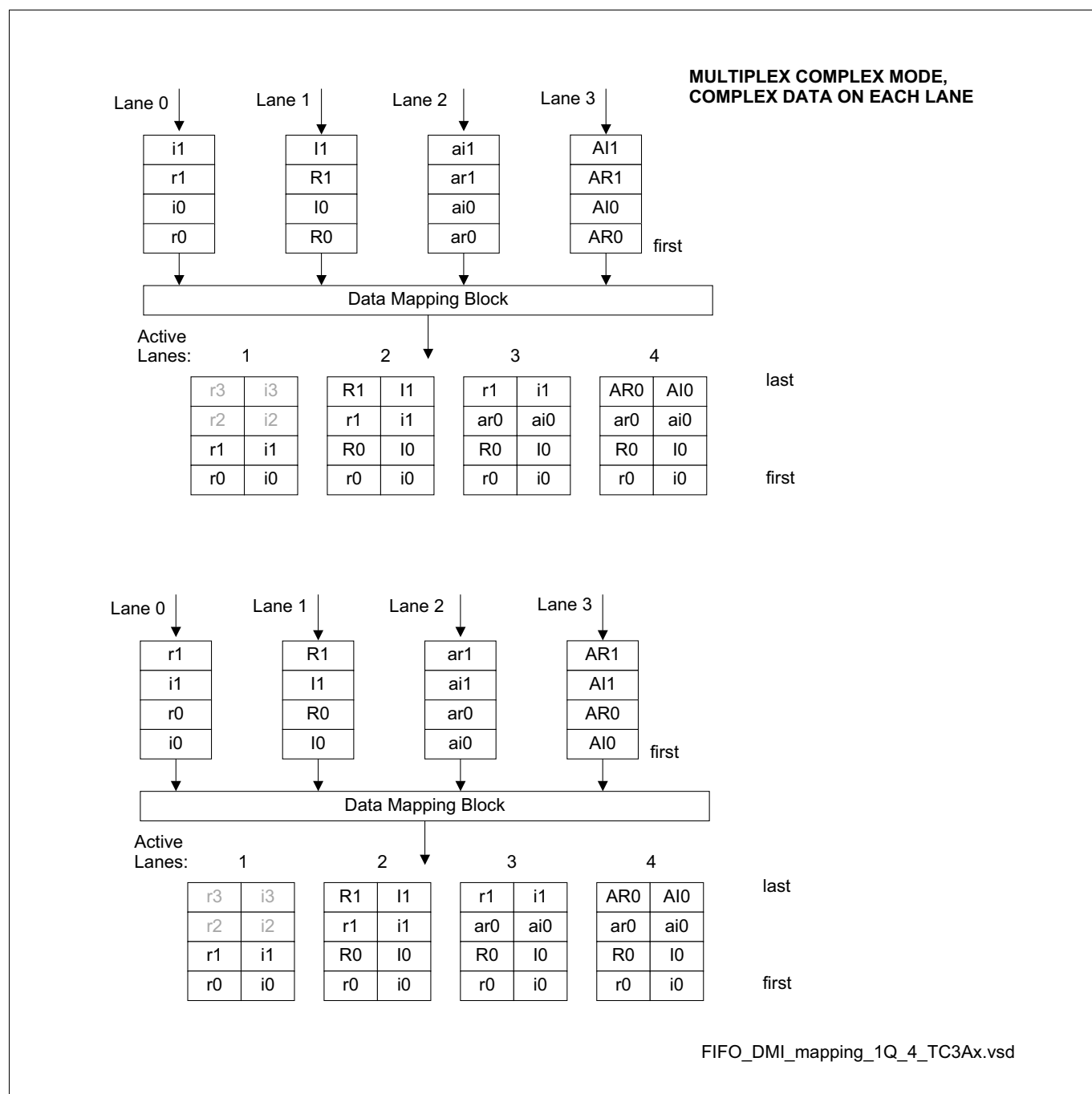
Figure 282 Multiplex Complex Sampling for Tc3Ax
