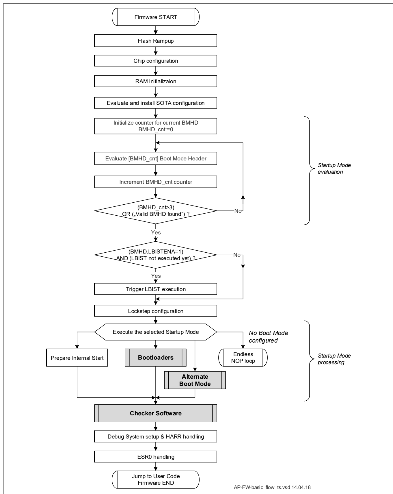
Figure 21 AURIX™ TC3xx Platform Firmware: main flow
