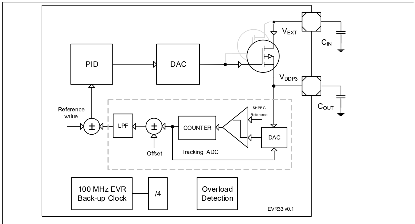
Figure 128 EVR33 LDO regulator
