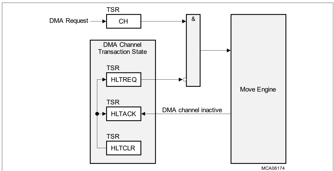
Figure 194 DMA Channel Halt Logic
