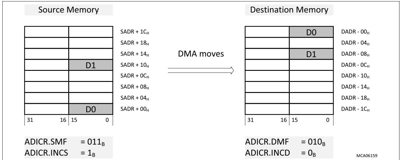
Figure 198 Programmable Address Generation - Example 1
