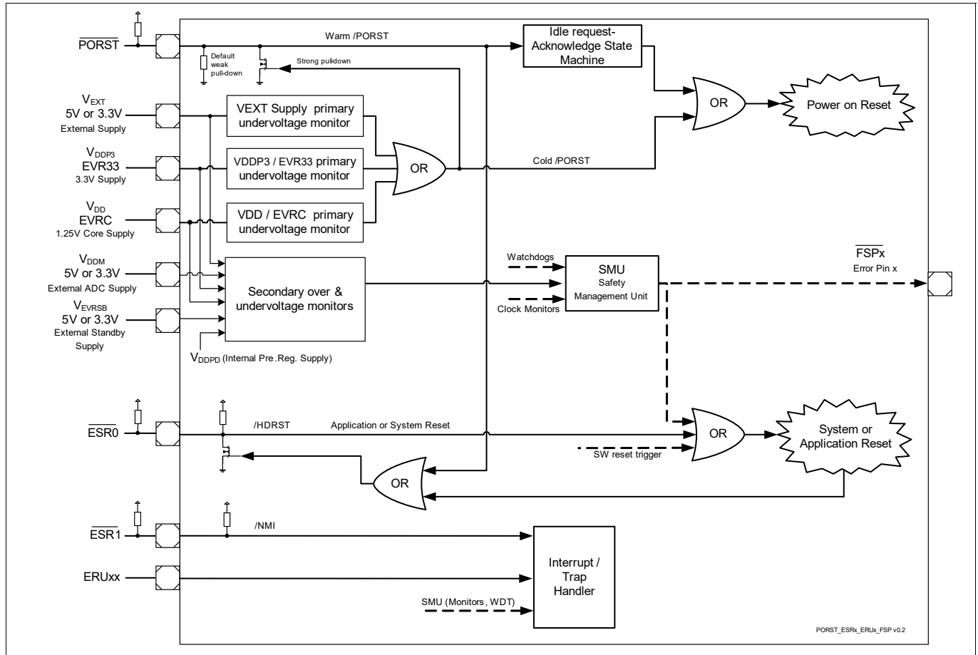
Figure 141 Monitoring and Reset Pins
