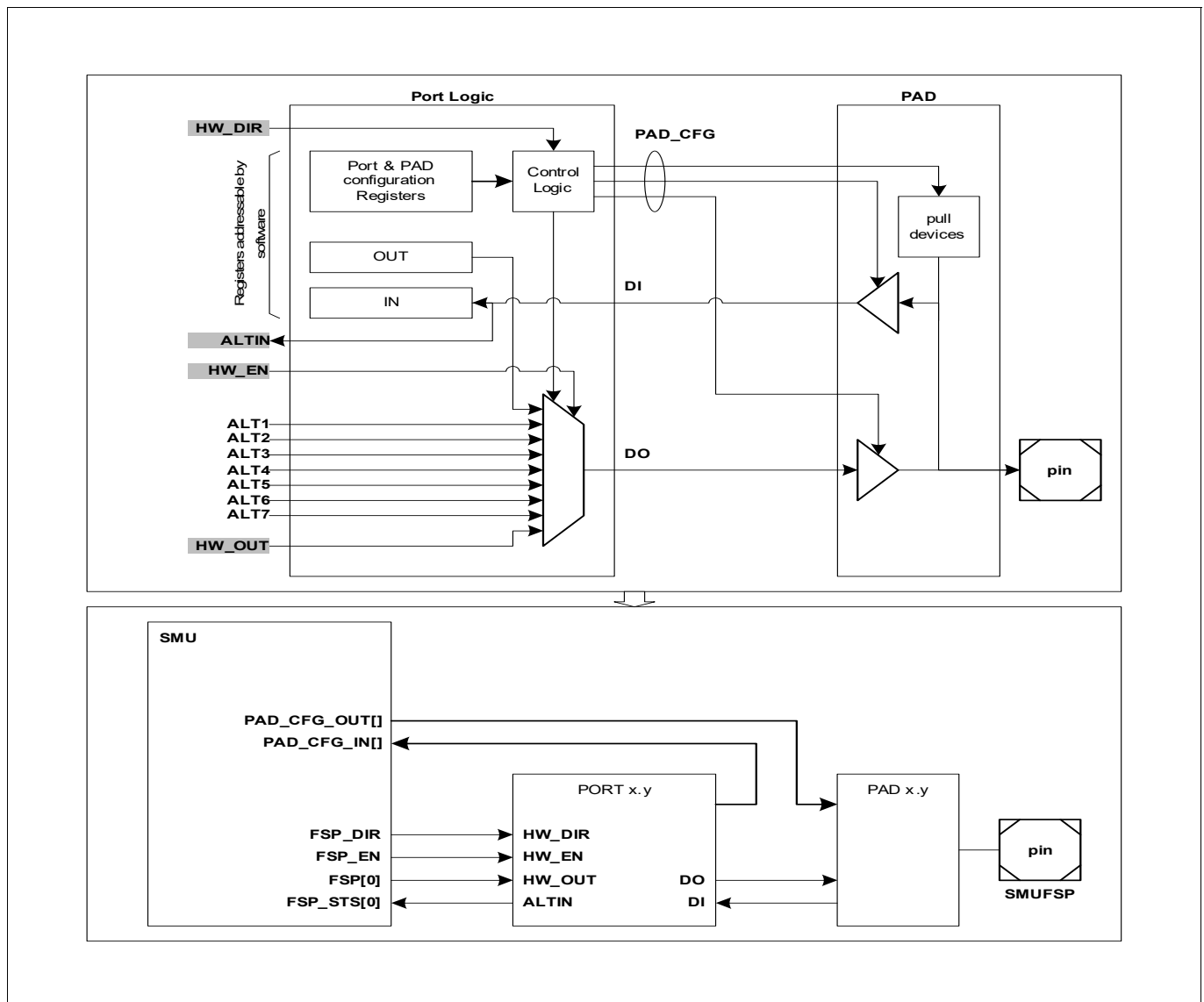
Figure 159 SMU/PAD Control Interface to the PADs
