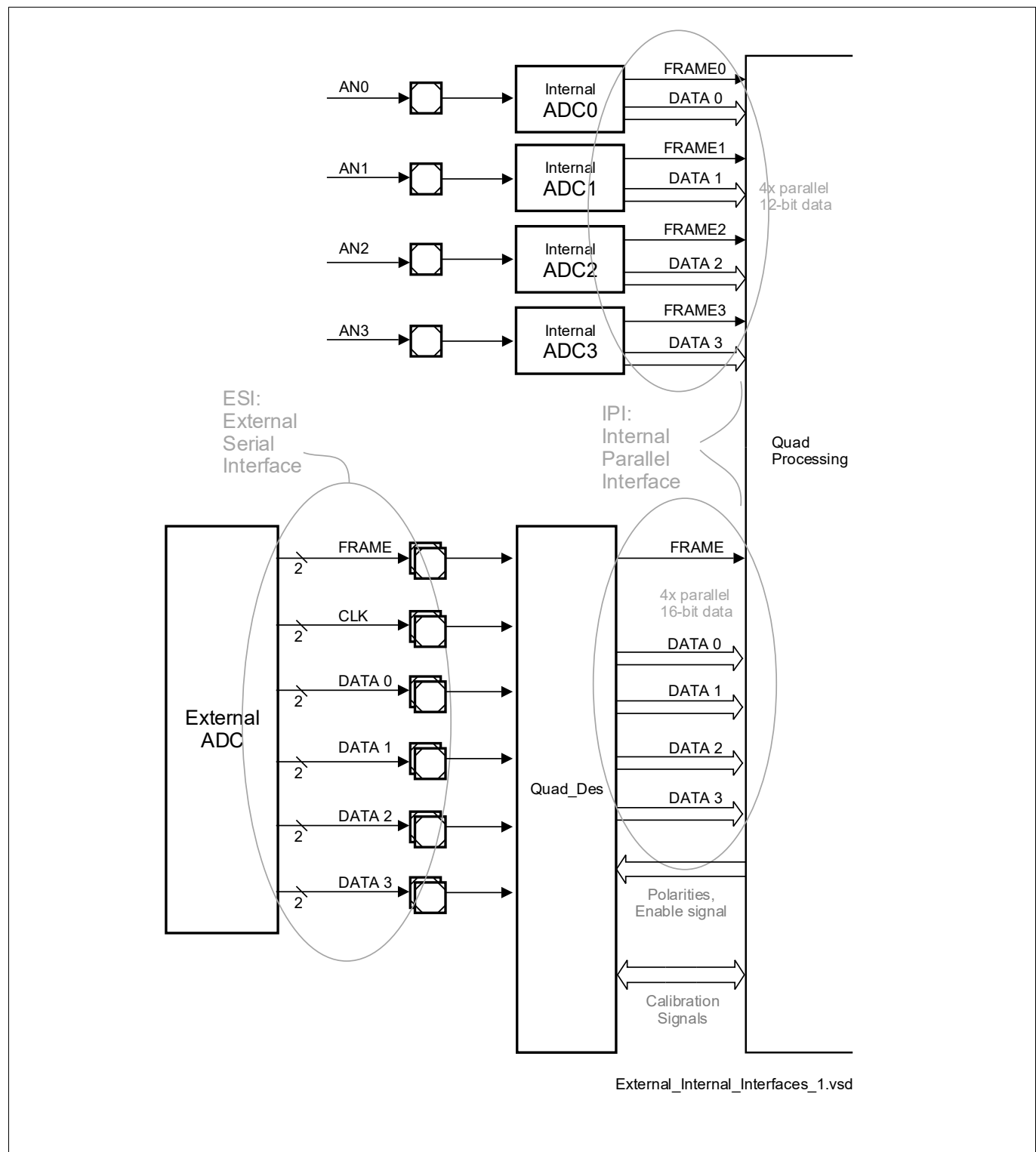
Figure 266 Input Interfaces of the RIF Module
