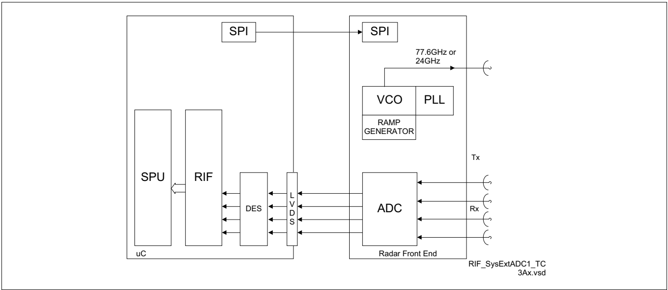
Figure 286 System View, TC3Ax External ADCs Use-Case
