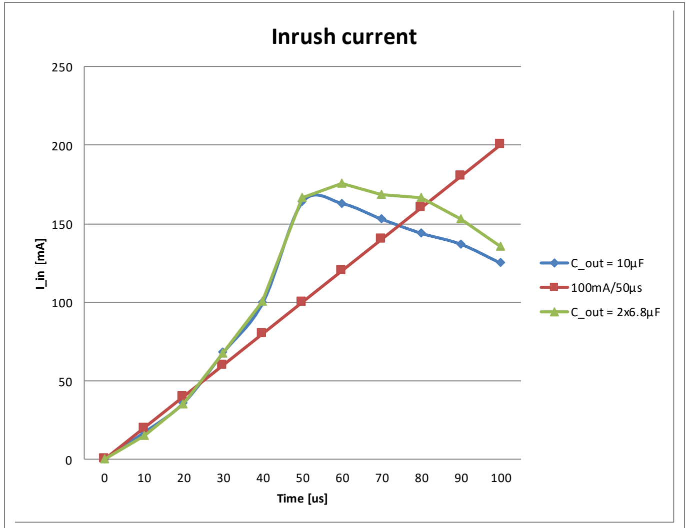
Figure 130 EVRC Inrush Current with different C_{out} values
