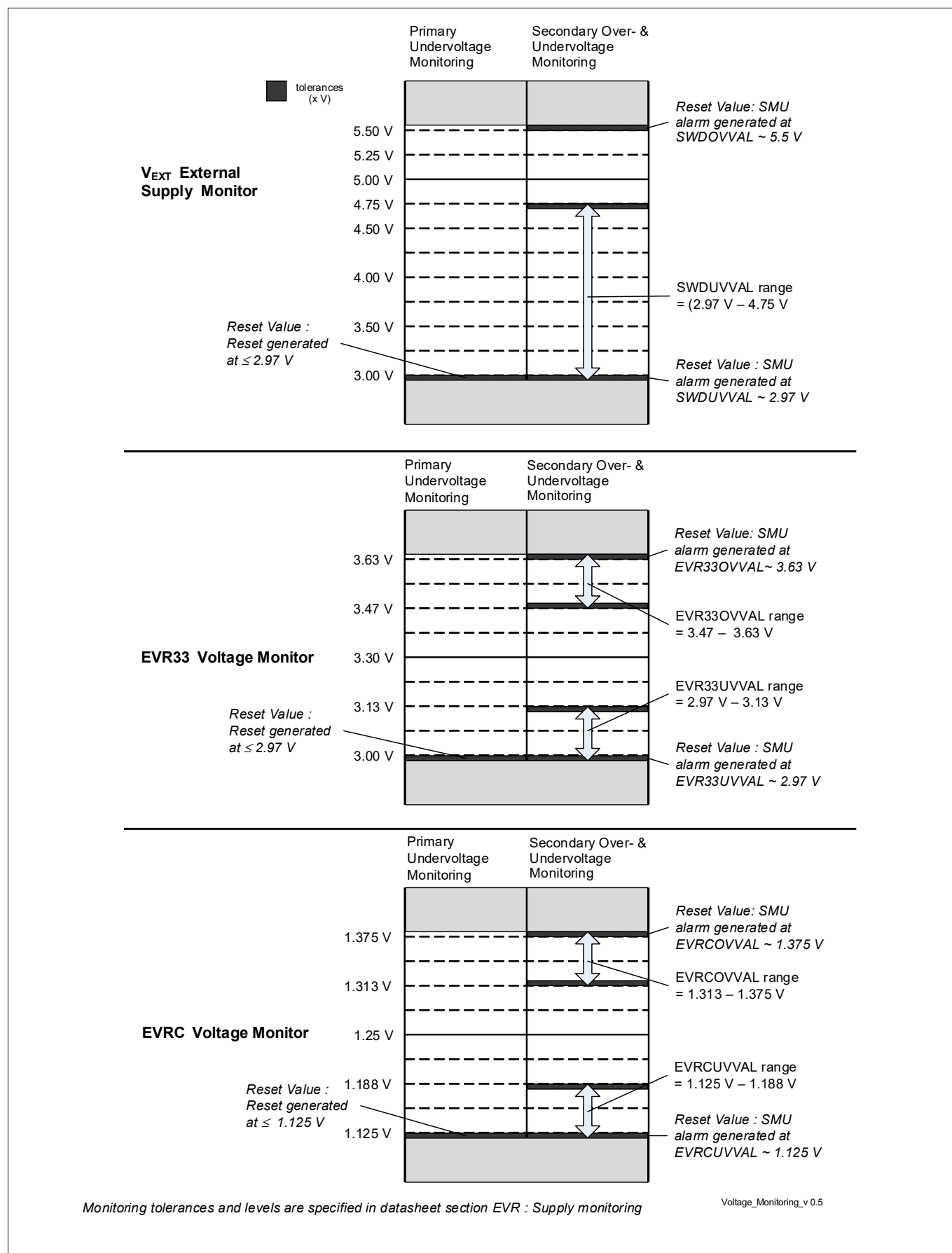
Figure 142 Voltage Monitoring - VEXT, VDDP3 &amp; VDD
