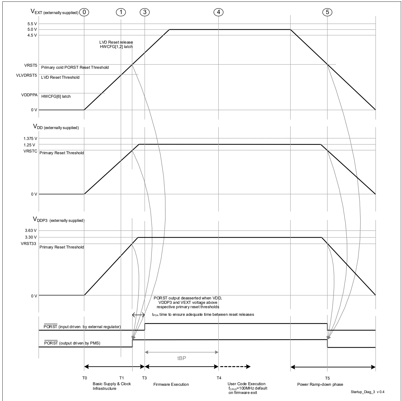
Figure 126 External Supply mode (h) - V_{EXT} , V_{DDP3} & V_{DD} externally supplied
