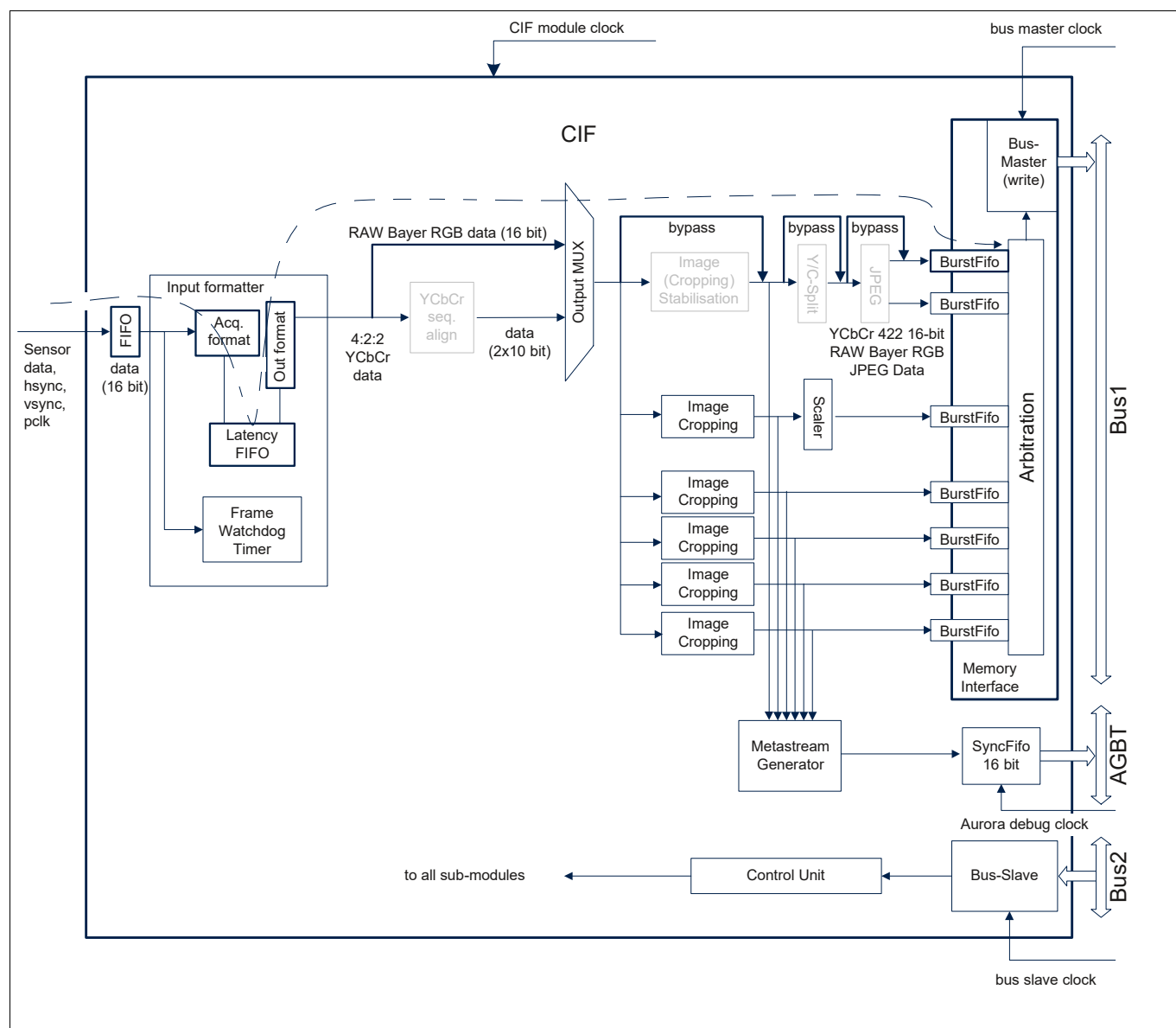
Figure 350 Active Blocks for Use Case Data Transfer
