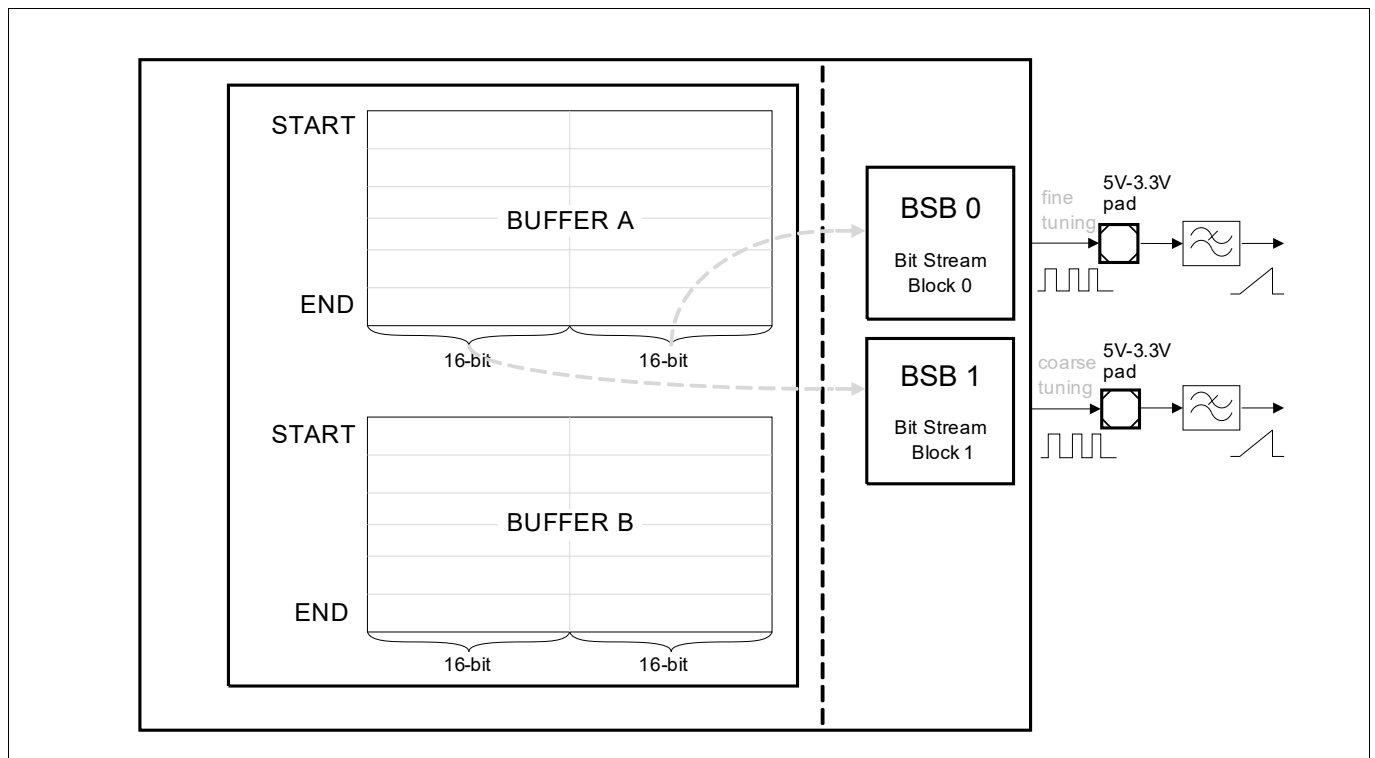
Figure 315 RAM storage of waveforms
