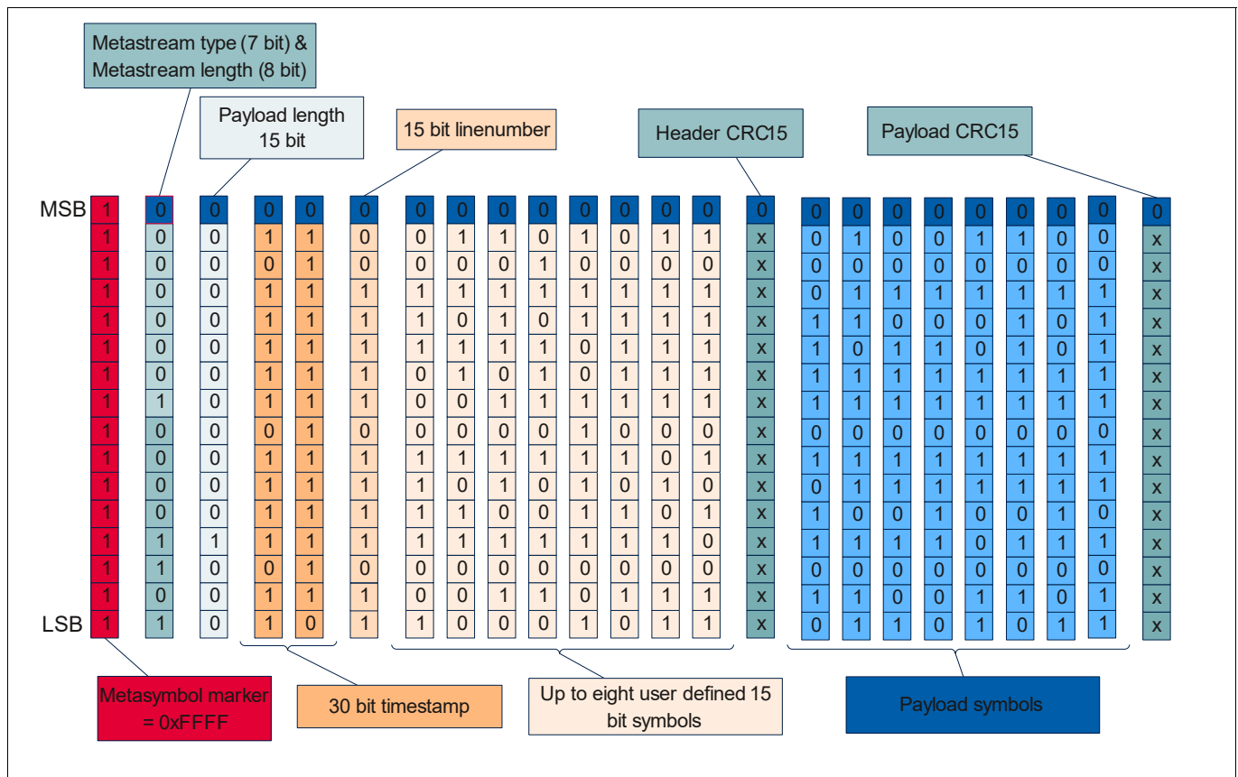
Figure 331 Line debug packet
