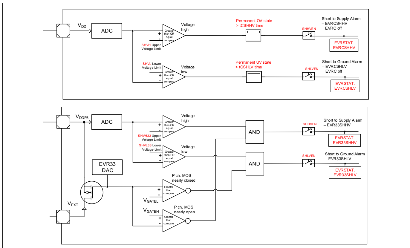
Figure 140 Short to Supply and Ground Detection
