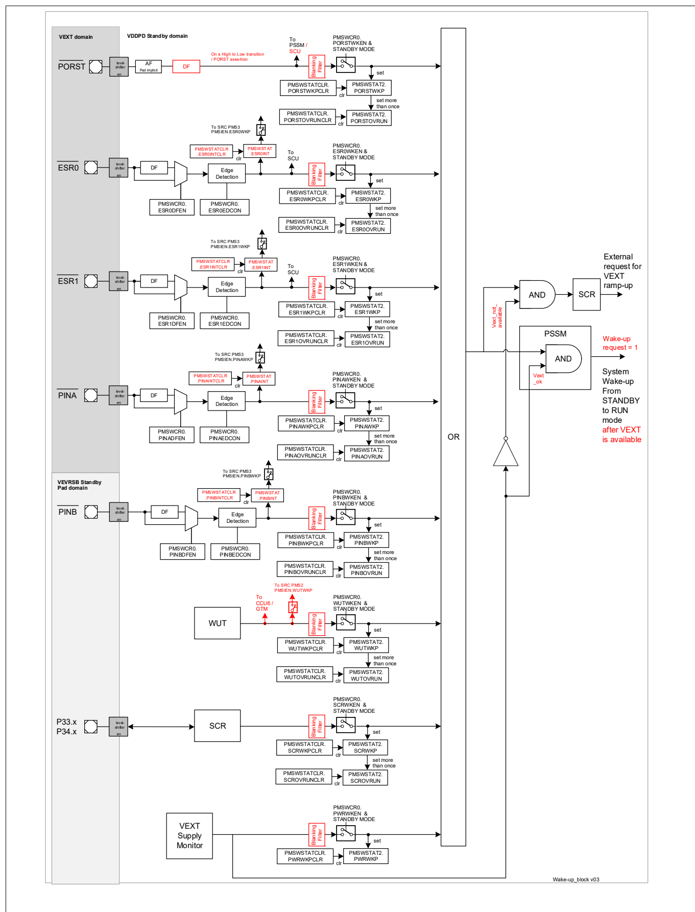
Figure 150 Wake-up Overview
