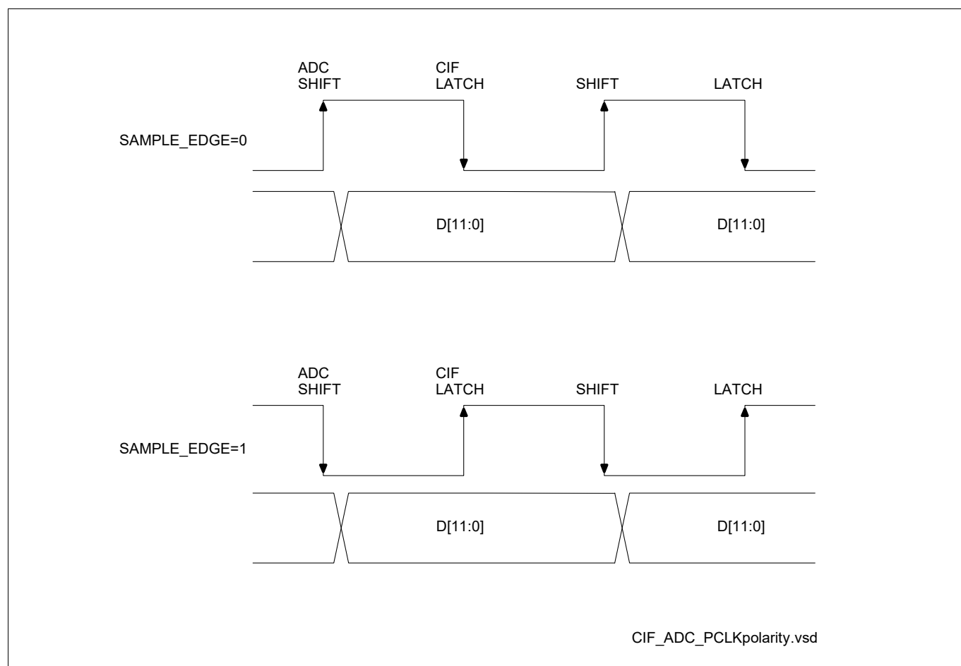
Figure 322 PCLK Clock Polarity and Data Transfer (12-bit ADC)
