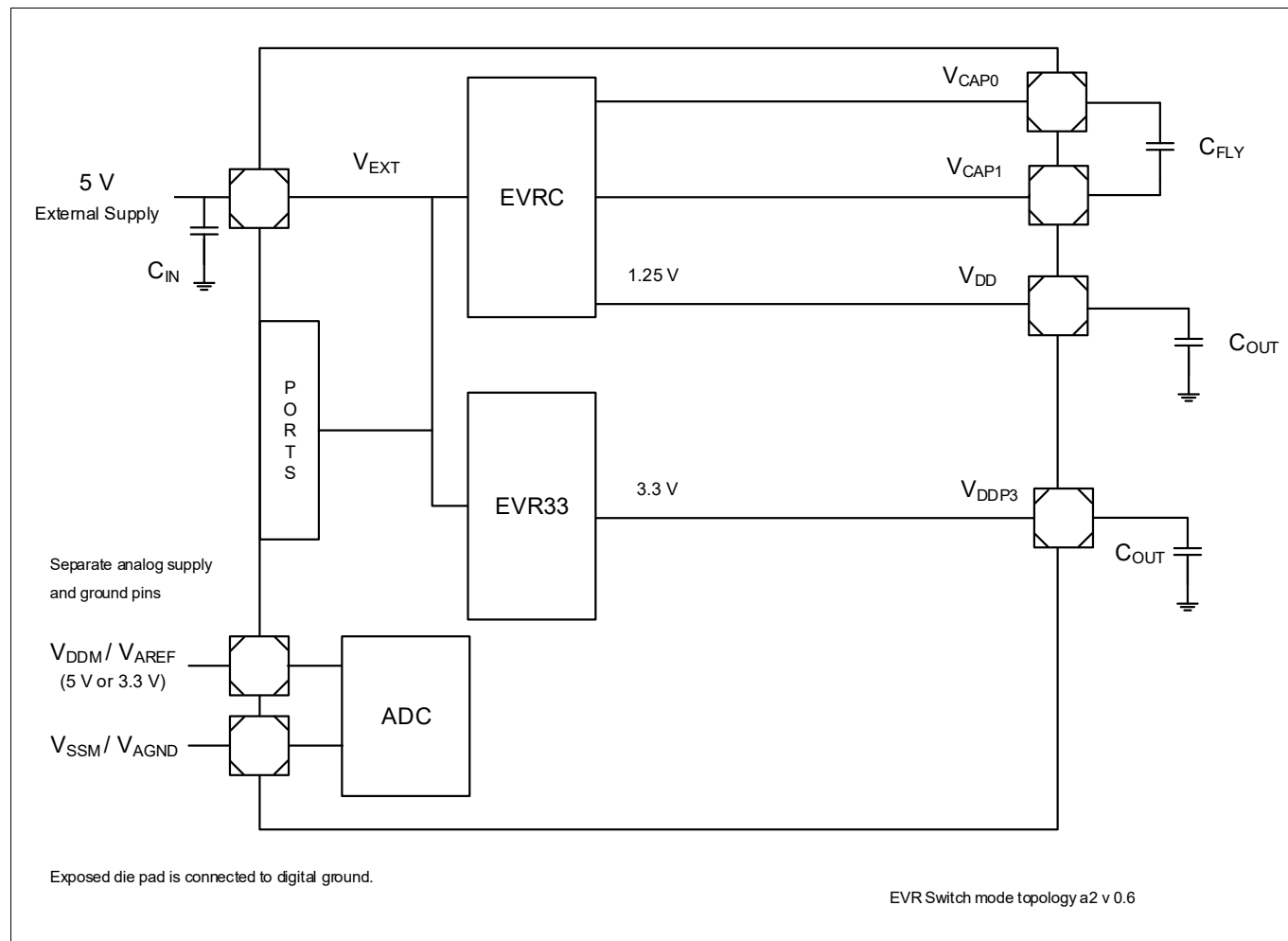
Figure 131 EVR Switch mode topology (a) - 5 V single supply
