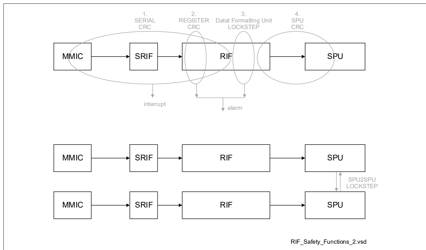
Figure 279 Safety Functions Overview
