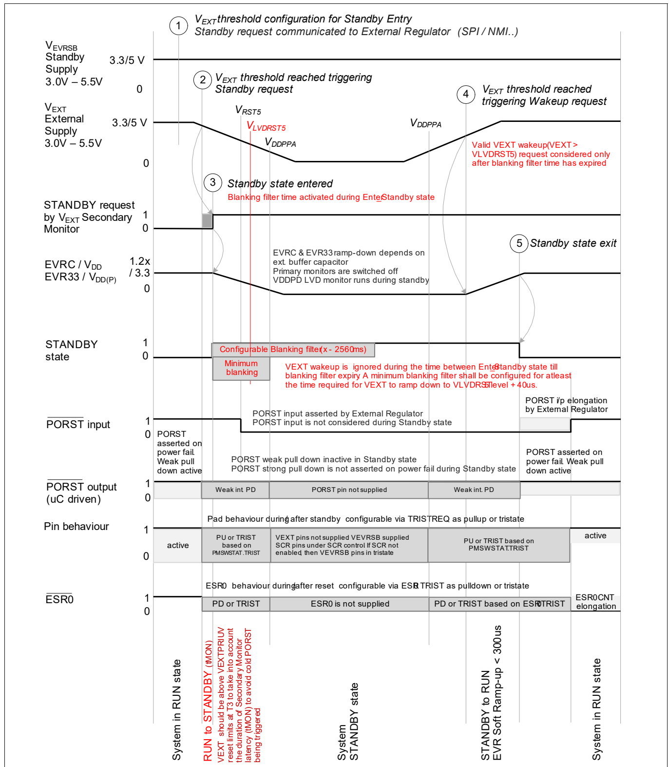
Figure 149 Standby entry on VEXT ramp-down and wake-up on VEXT ramp-up
