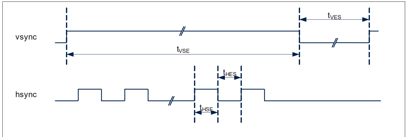
Figure 325 Programmable time-outs for the Security Watchdog
