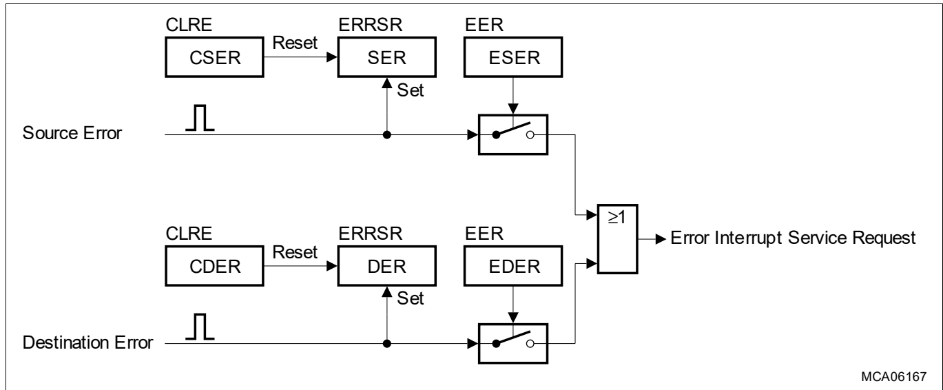
Figure 220 Source and Destination Error Interrupt Service Request
