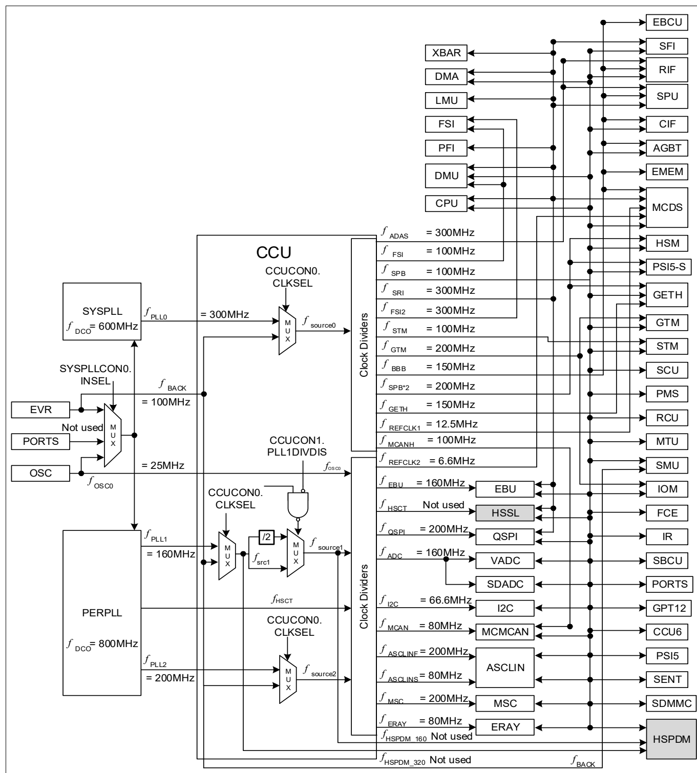
Figure 91 Clocking System example with external 25MHz crystal / clock input
