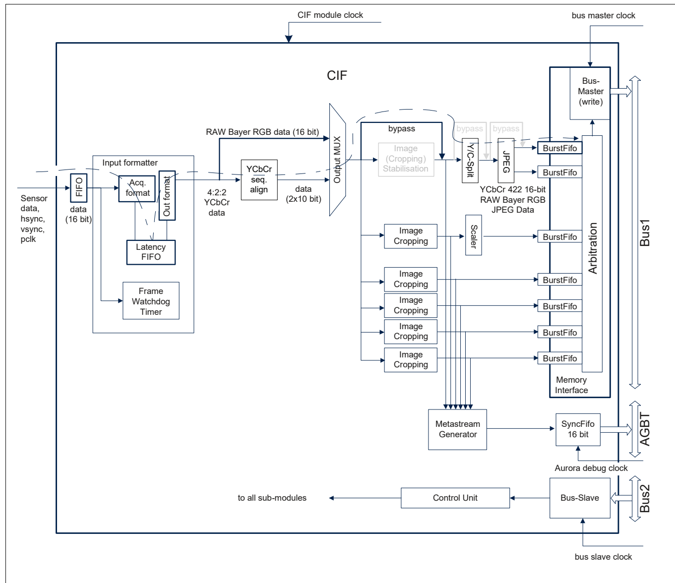
Figure 352 Active Blocks for Use Case Still Image Capture
