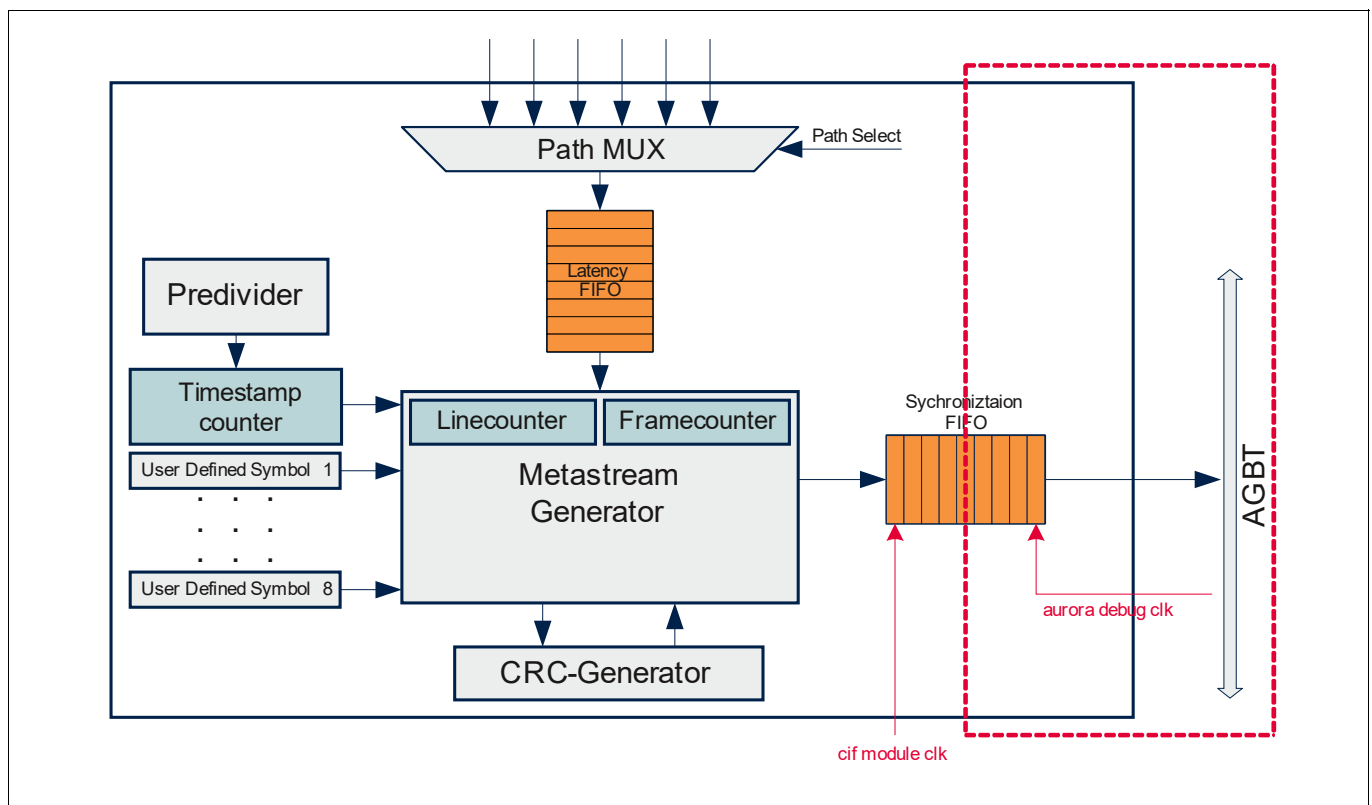
Figure 330 Debug Path block diagram
