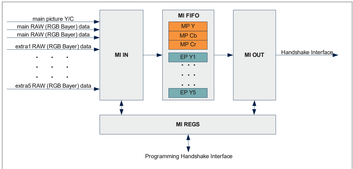
Figure 335 Block Diagram of the Memory Interface write path
