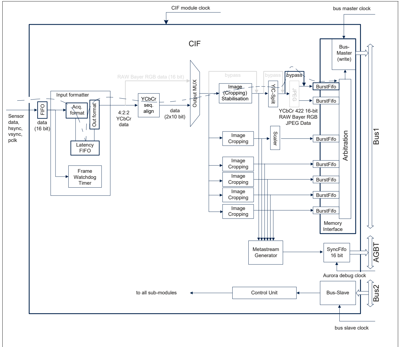
Figure 351 Active Blocks for Use Case Viewfinder
