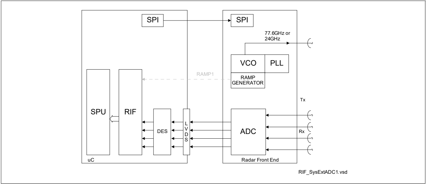
Figure 285 System View, External ADCs Use-Case
