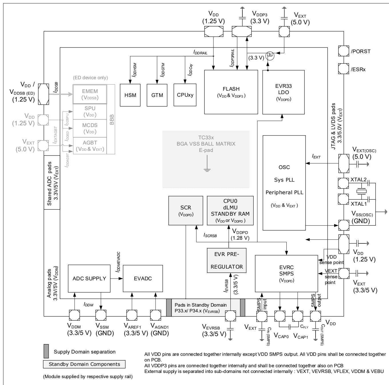
Figure 122 TC3xx Supply Pins and Module Connectivity
