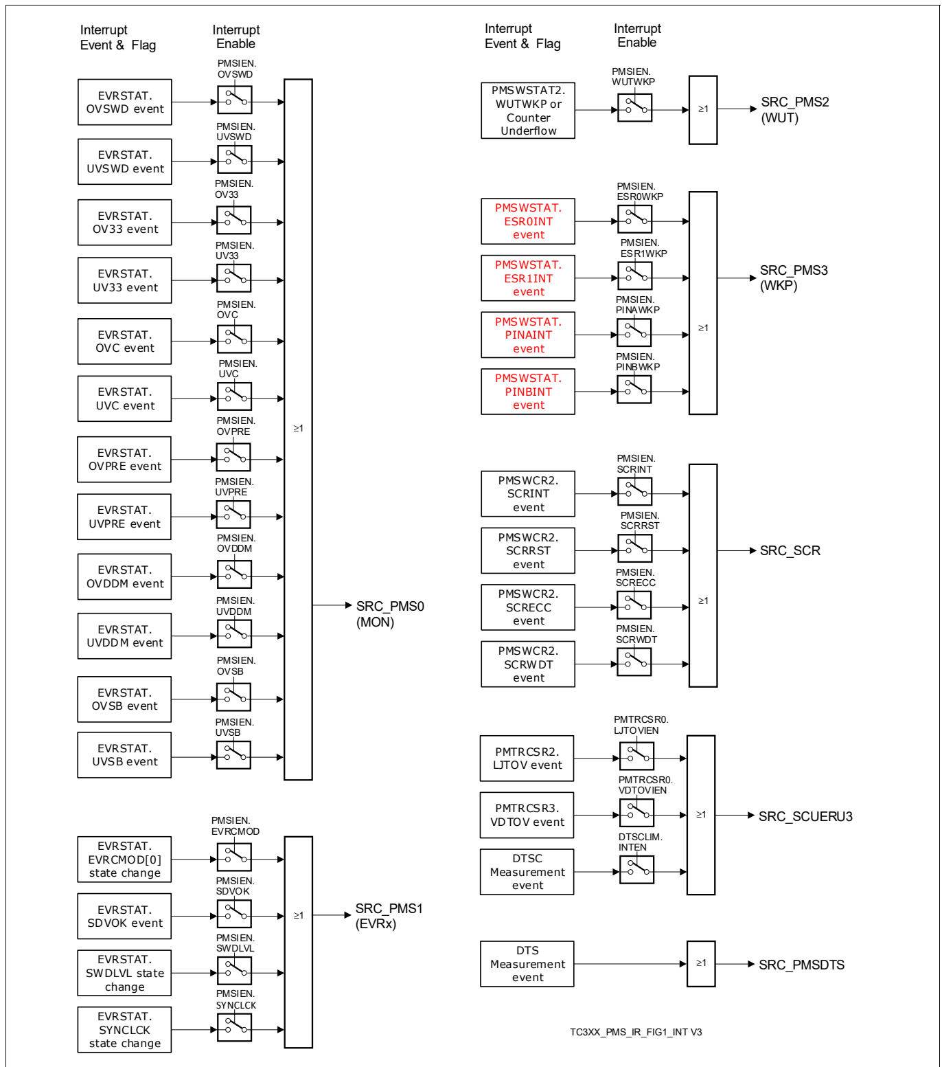
Figure 144 Interrupt Sources and Events
