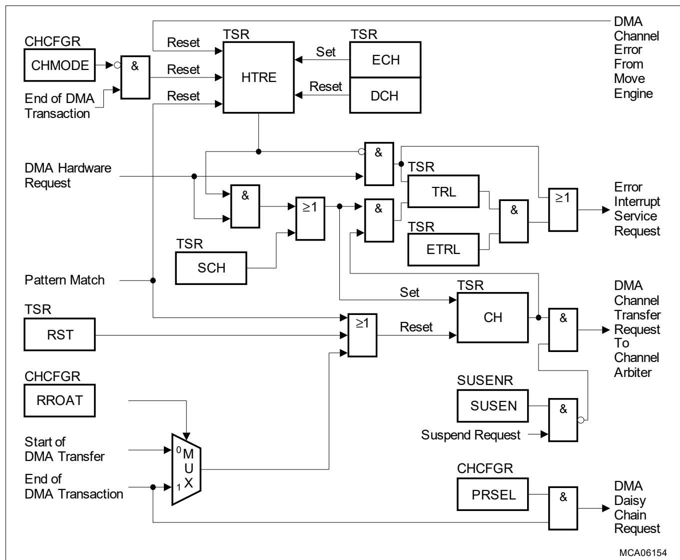
Figure 189 DMA Channel Request Control
