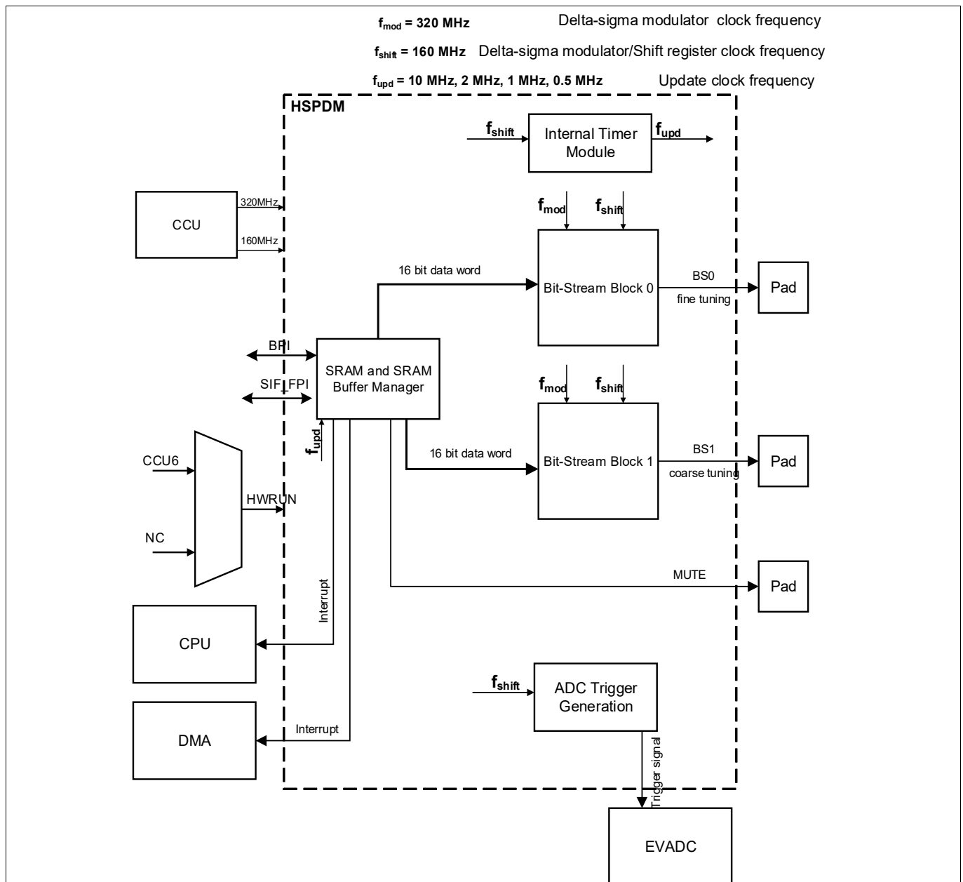
Figure 304 High speed pulse density modulation block level diagram
