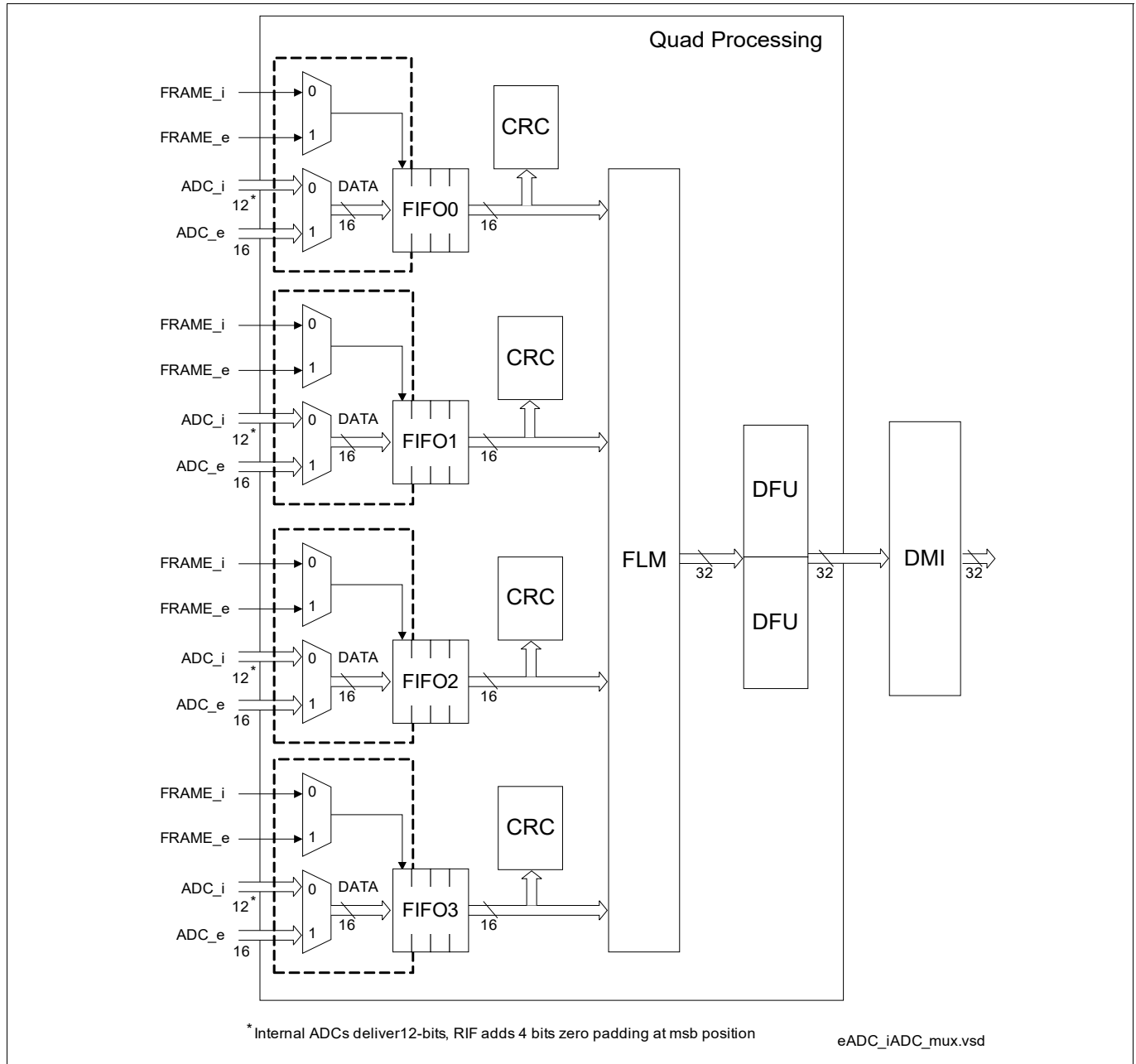
Figure 271 Quad Processing Unit
