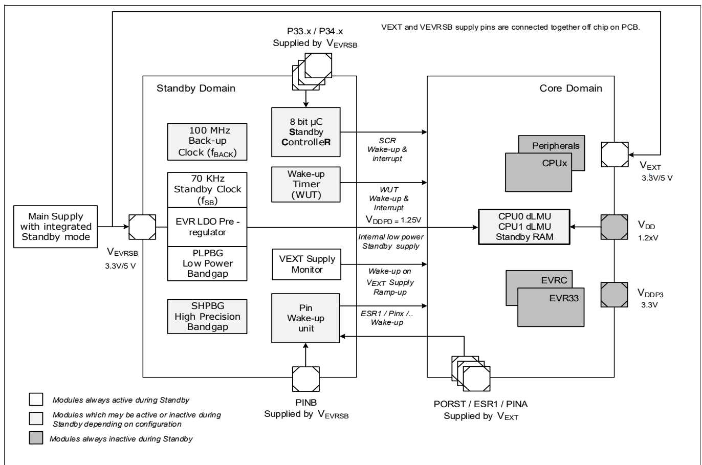
Figure 147 Standby domain supplied via a common supply rail connected to both VEXT and VEVRSB
