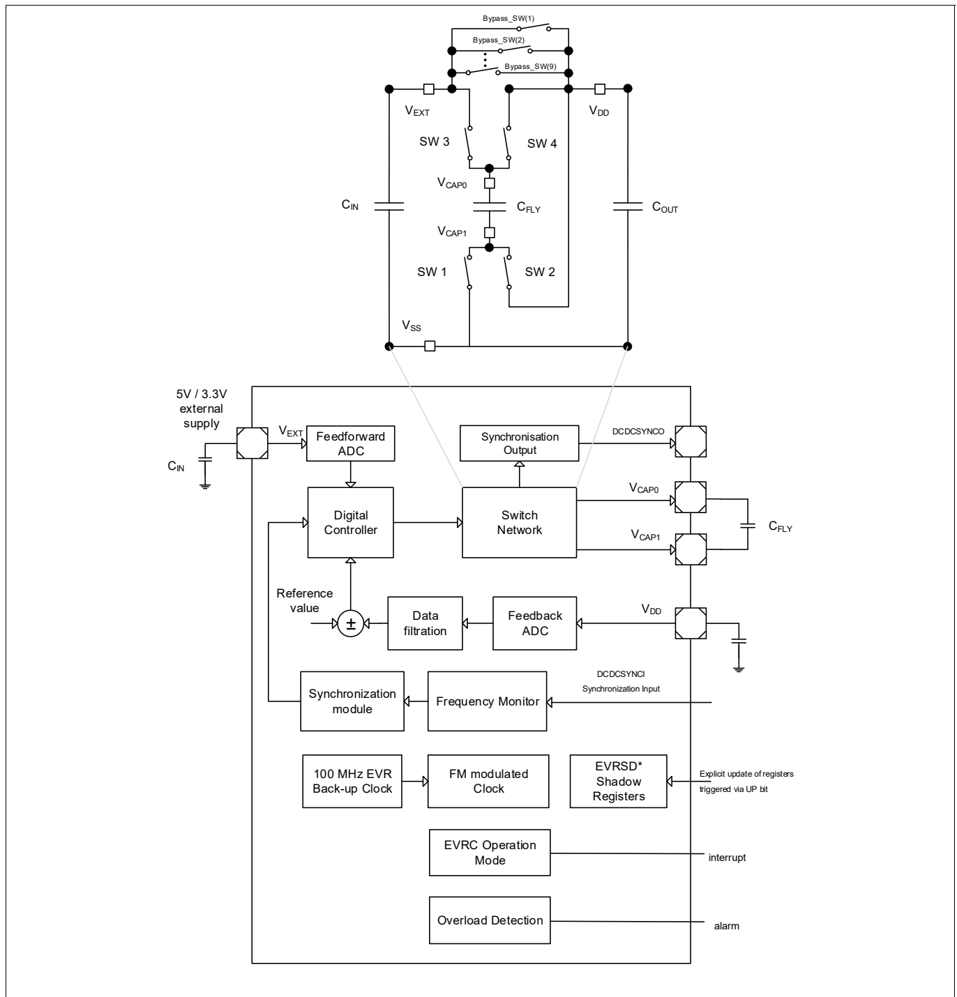
Figure 129 EVRC Step down regulator
