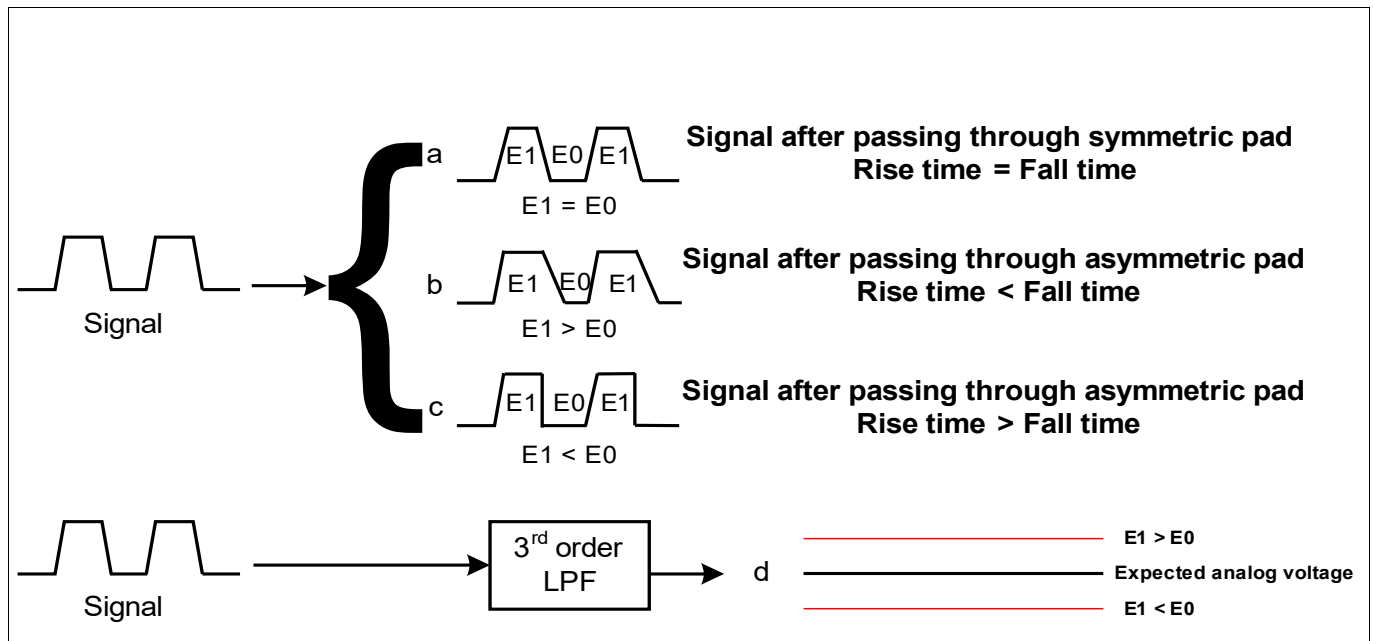
Figure 311 (a) Symmetric pad (b) Asymmetric pad with the rise time < fall time (c) Asymmetric pad with the rise time > fall time (d) DC voltage offset after passing of the PDM through the LPF
