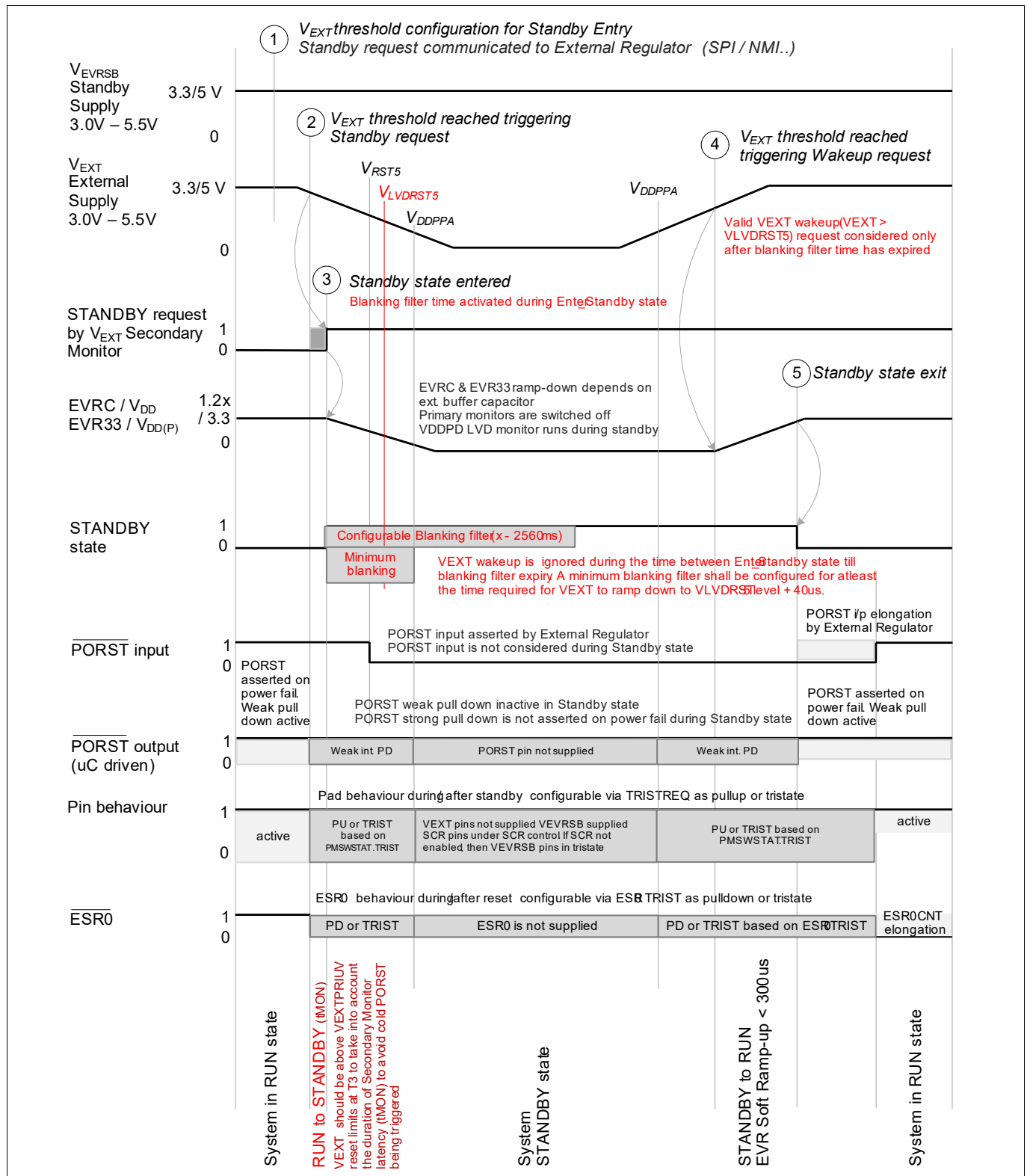
Figure 118 Standby entry on VEXT ramp-down and wake-up on VEXT ramp-up
