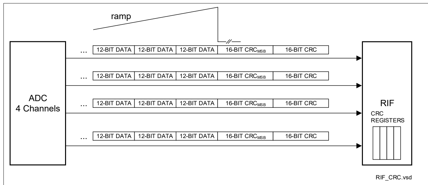
Figure 272 CRC Overview
