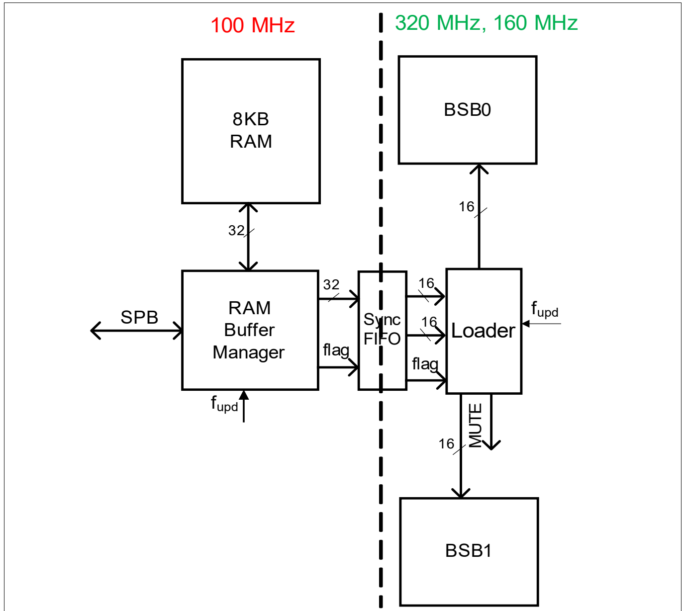
Figure 313 SRAM and data management
