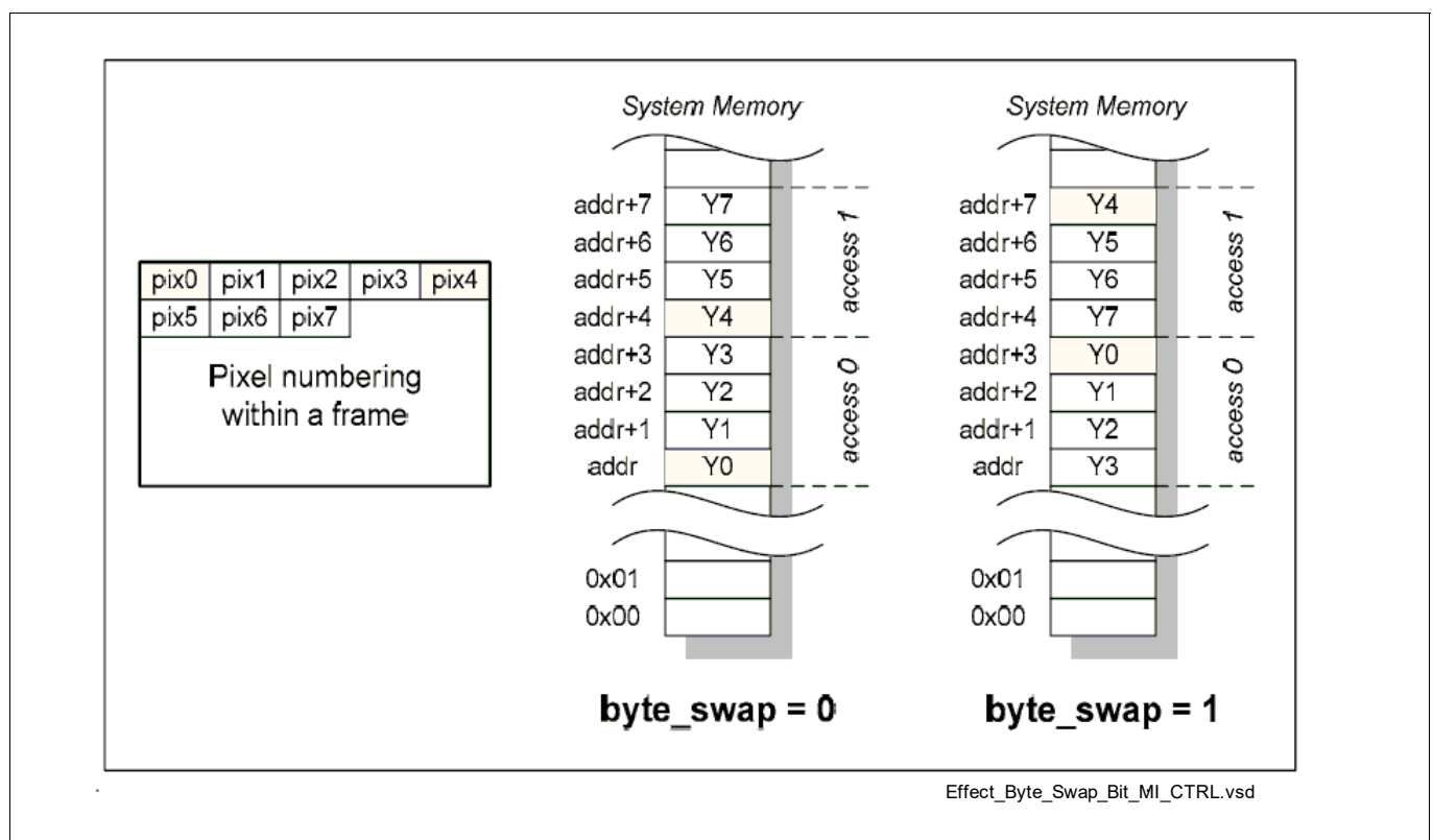
Figure 347 Effect of the byte_swap bit in MI_CTRL
