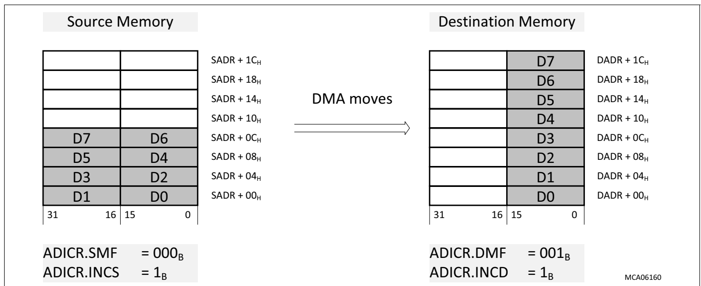
Figure 199 Programmable Address Generation - Example 2
