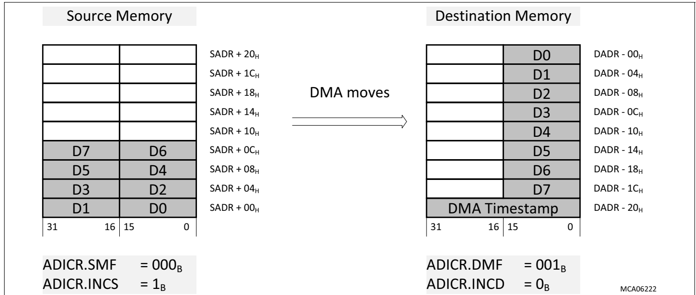
Figure 206 Decrementing Destination Address: DMA Timestamp appended below DMA Write Move Data
