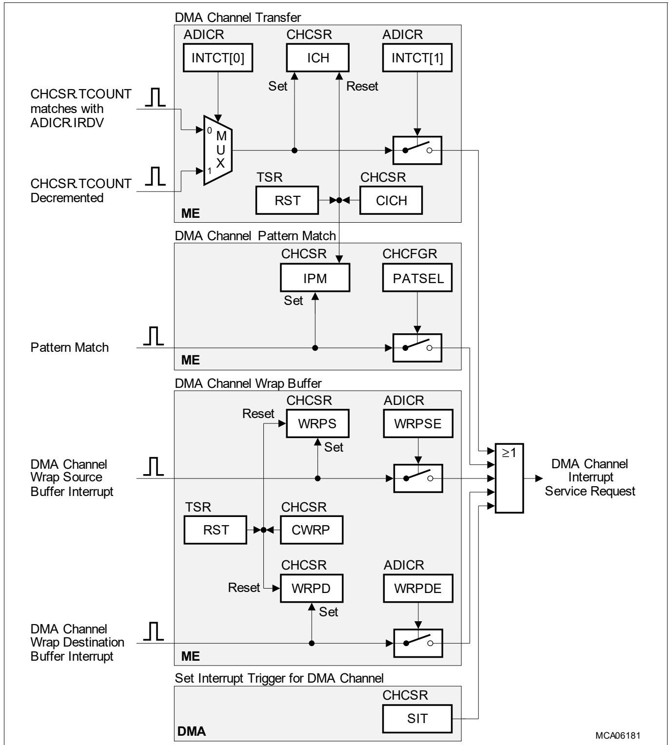
Figure 202 DMA Channel Interrupt Service Request
