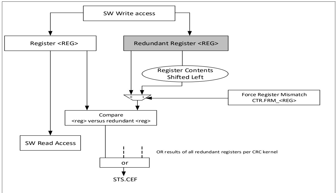
Figure 184 Register monitoring scheme
