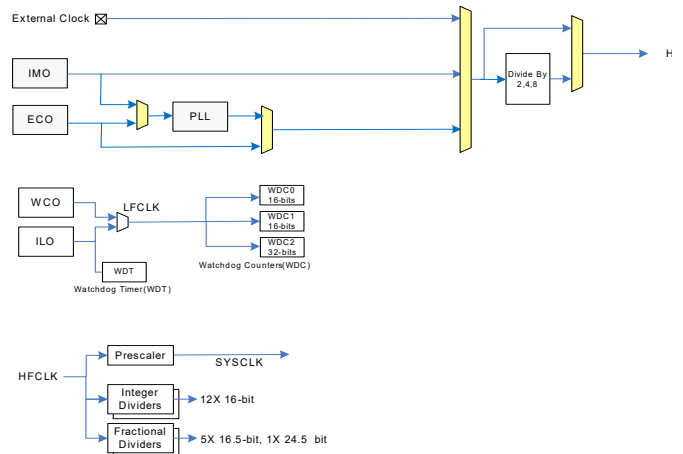
Figure 3. PSoC 4100S Plus MCU Clocking Architecture
