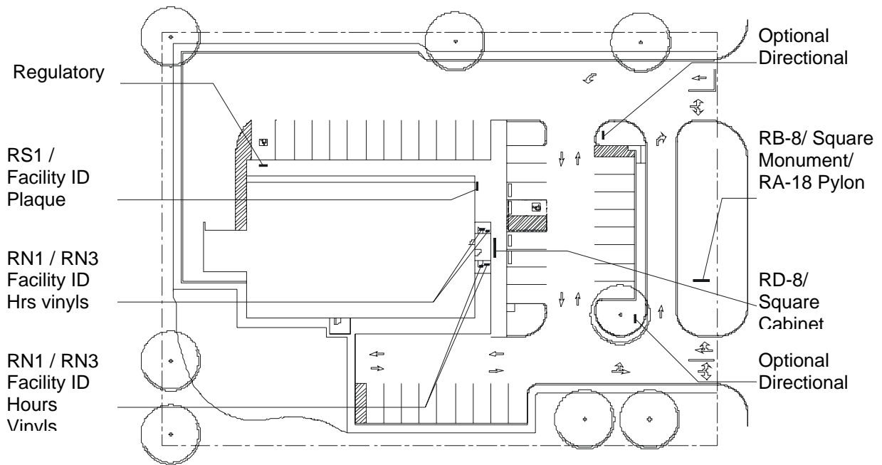
Exhibit 3-5k Typical site plan showing sign placement for SSBSD plans 40, 50, 65A, 80A, and 100A
