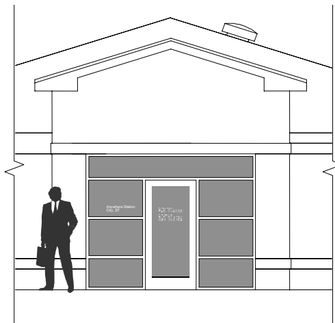
Exhibit 3-5h Typical elevation of entrance with vinyl placement for SSBD plans 20, 25 & 30
