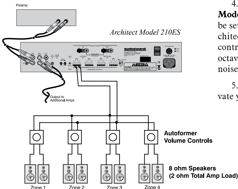
Four Zone System with Volume Controls
