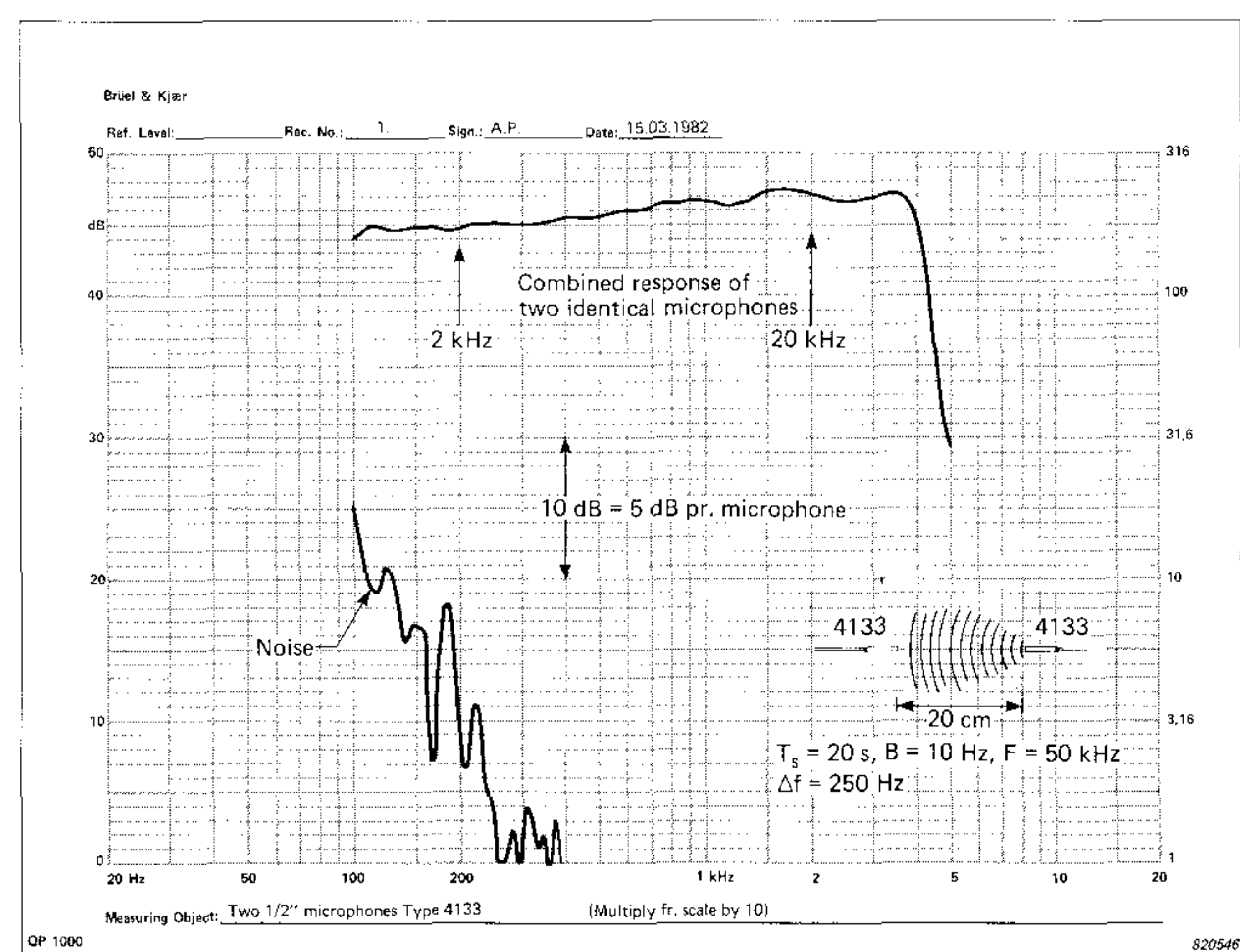
Fig. 10. Total, compensated frequency response of two 1/2" Microphones Type 4133 using one as a sound source and the other as a receiver. Deviations from the ideal flat response can be equally attributed to the emitter and the receiver thus making the 10dB division on the vertical axis equivalent to 5dB per microphone. For signal to noise evaluation the 10dB division is valid
