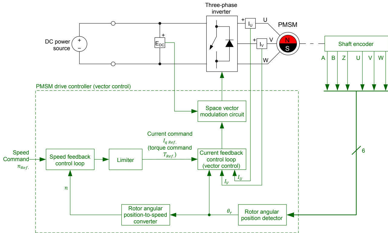
Figure 38. Block diagram of a vector control PMSM drive.
