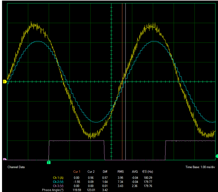
Figure 43. Phase angle difference \Delta\theta between the vertical cursors of the Oscilloscope (i.e., phase angle difference between the waveform of current I_U and the waveform of the signal indicating the angular position of the PMSM rotor) when the amount of torque T produced by the PMSM is equal to 0.00 N·m (0.00 lbf·in).
