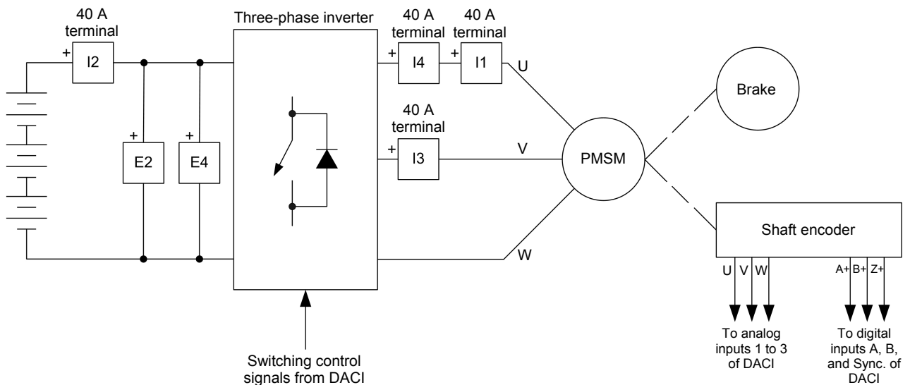
Figure 44. Vector control PMSM drive connected to a brake.
