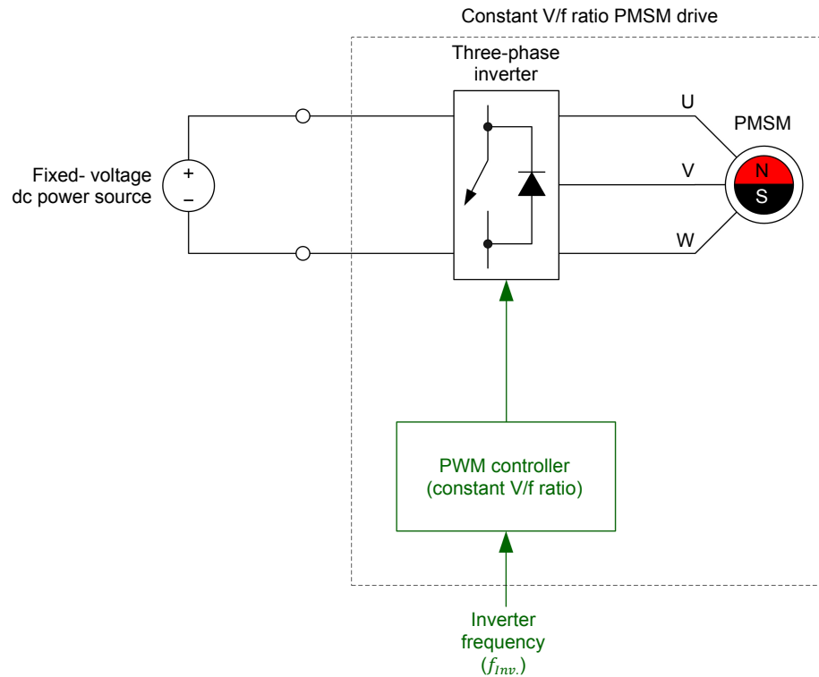
Figure 35. Block diagram of a typical constant V/f ratio PMSM drive.
