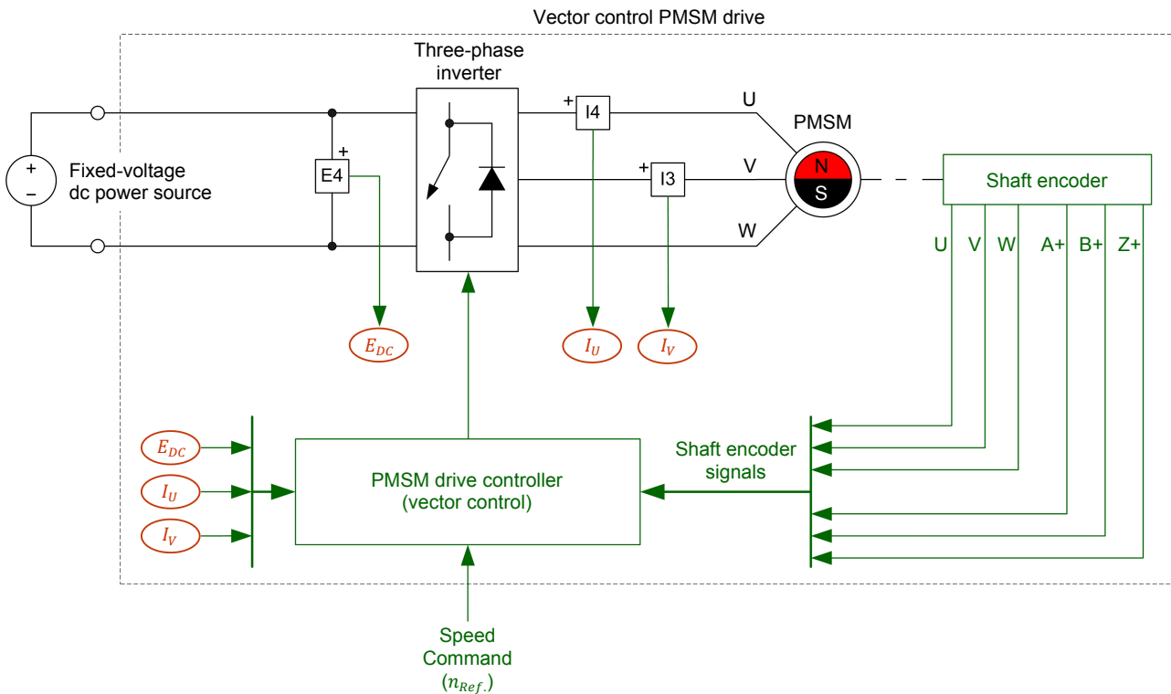
Figure 36. Block diagram of a typical vector control PMSM drive.
