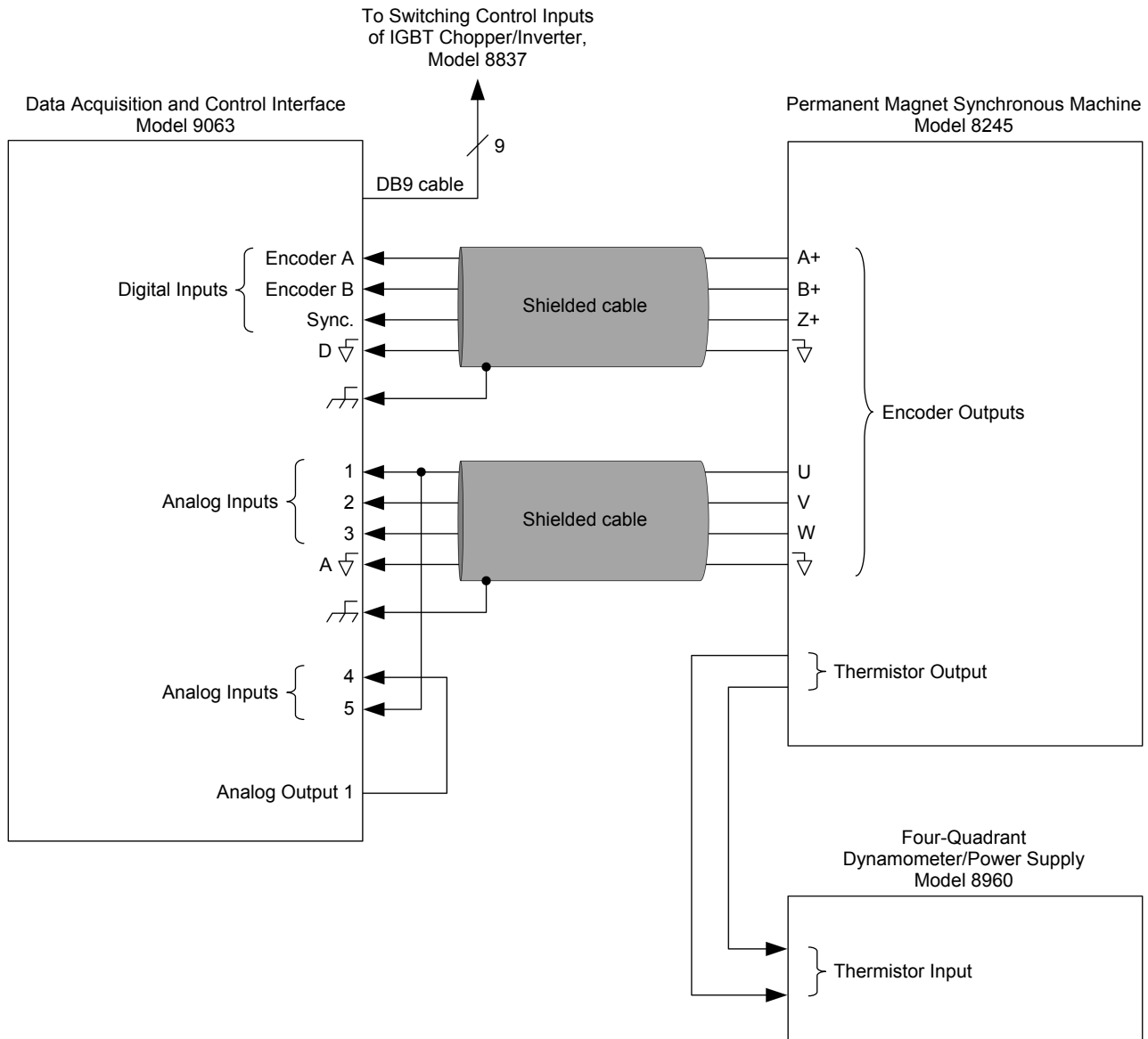
Figure 42. Low-power connections required to study the operation of the constant V/f ratio PMSM drive shown in Figure 41.
