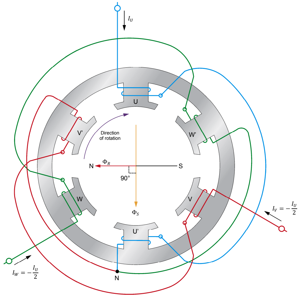
Figure 40. In a vector control PMSM drive, the stator magnetic flux lags behind the rotor magnetic flux by 90^\circ at all times when the PMSM operates as a generator (e.g., during braking).
