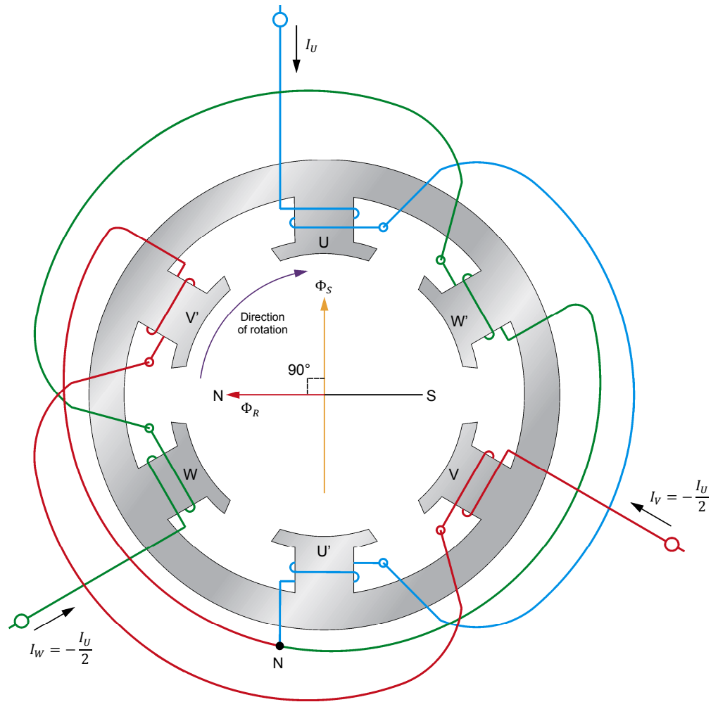
Figure 39. In a vector control PMSM drive, the stator magnetic flux leads the rotor magnetic flux by 90^\circ at all times when the PMSM operates as a motor.
