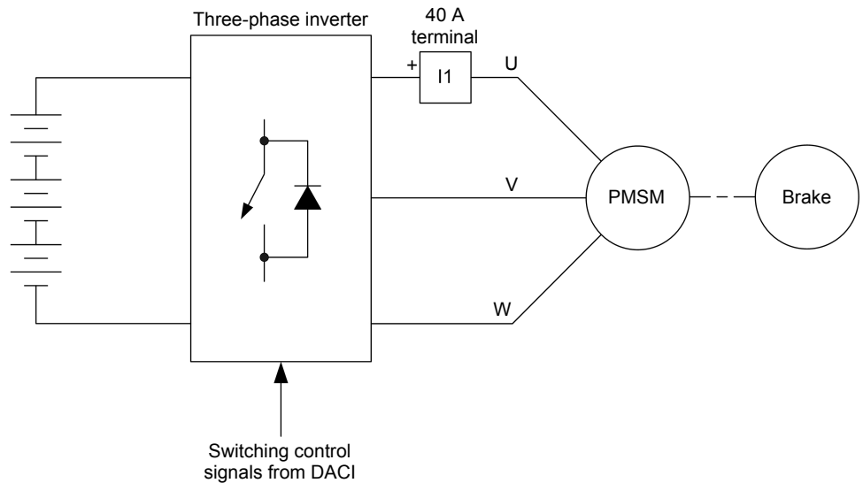
Figure 41. Constant V/f ratio PMSM drive connected to a brake.
