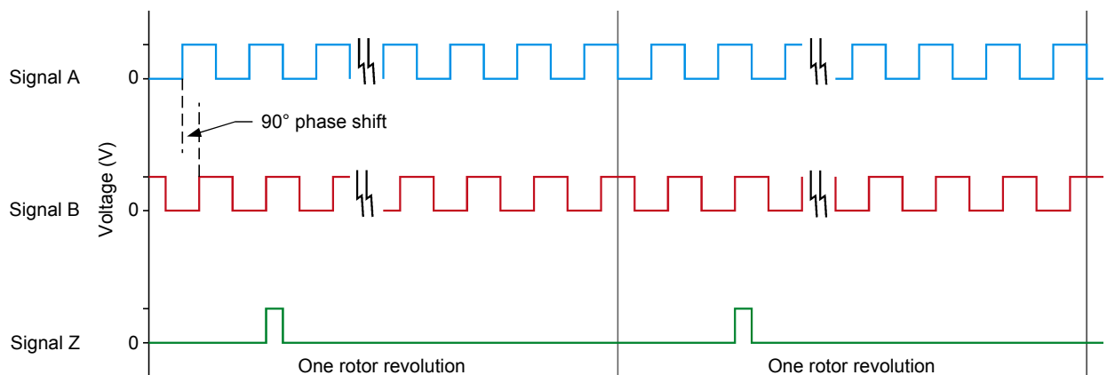
Figure 37. Typical A, B, and Z signals produced by the shaft encoder in a vector control PMSM drive.
