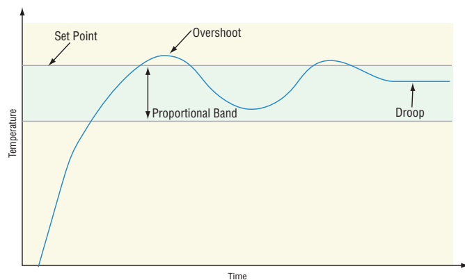
Proportional Control
