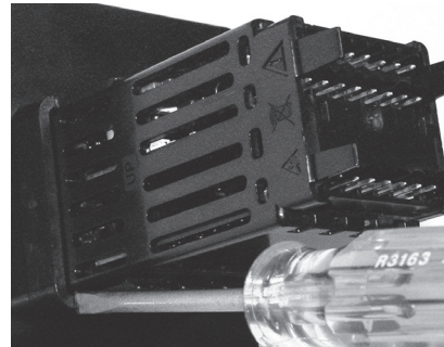
Place the blade of a screwdriver in any of the corner of the mounting collar assembly.
