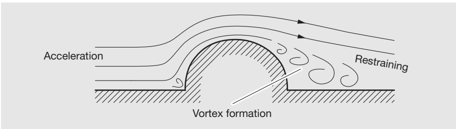
Fig. 1-3: Dead Zone with Vortex Formation
