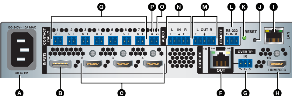
Figure 7. IN1804 DO Rear Panel
