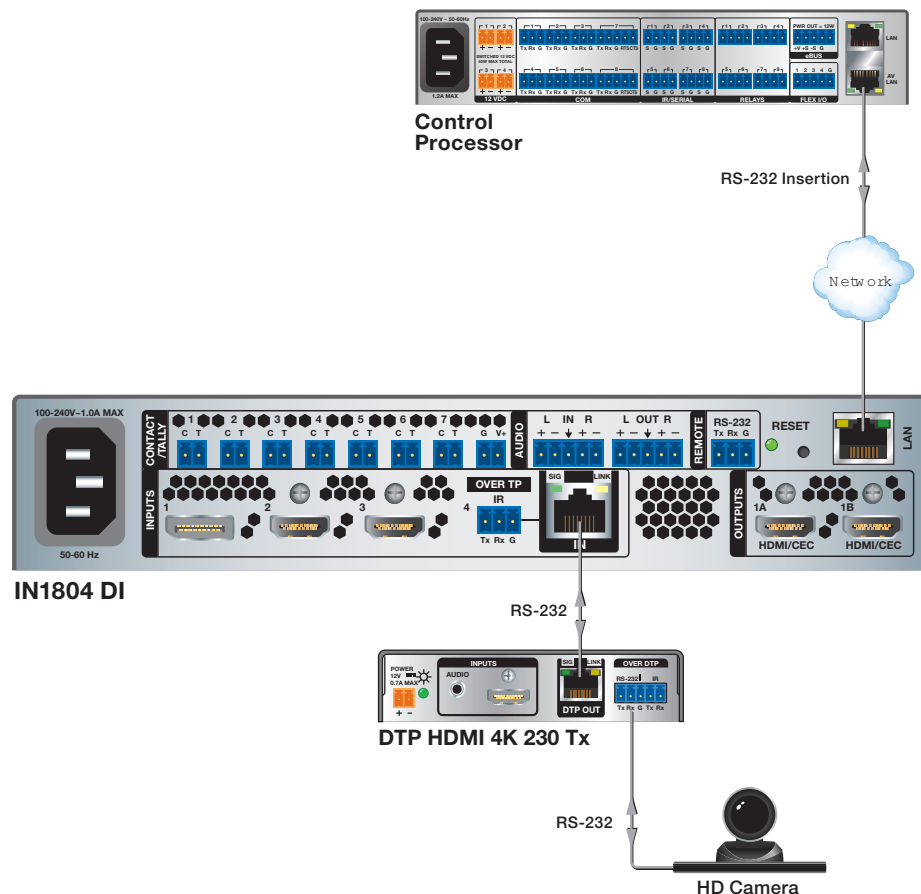
Figure 31. Typical Ethernet to RS-232 Insertion to an Input Endpoint
