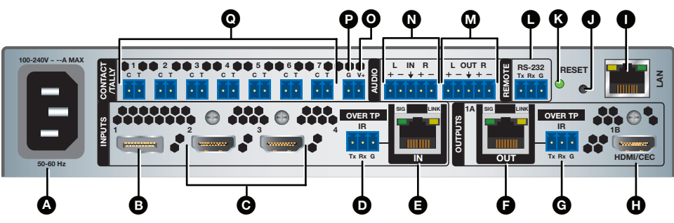
Figure 8. IN1804 DI/DO Rear Panel
