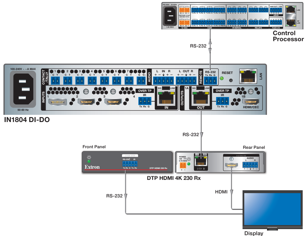
Figure 33. Typical Connection for Unidirectional RS-232 Insertion
