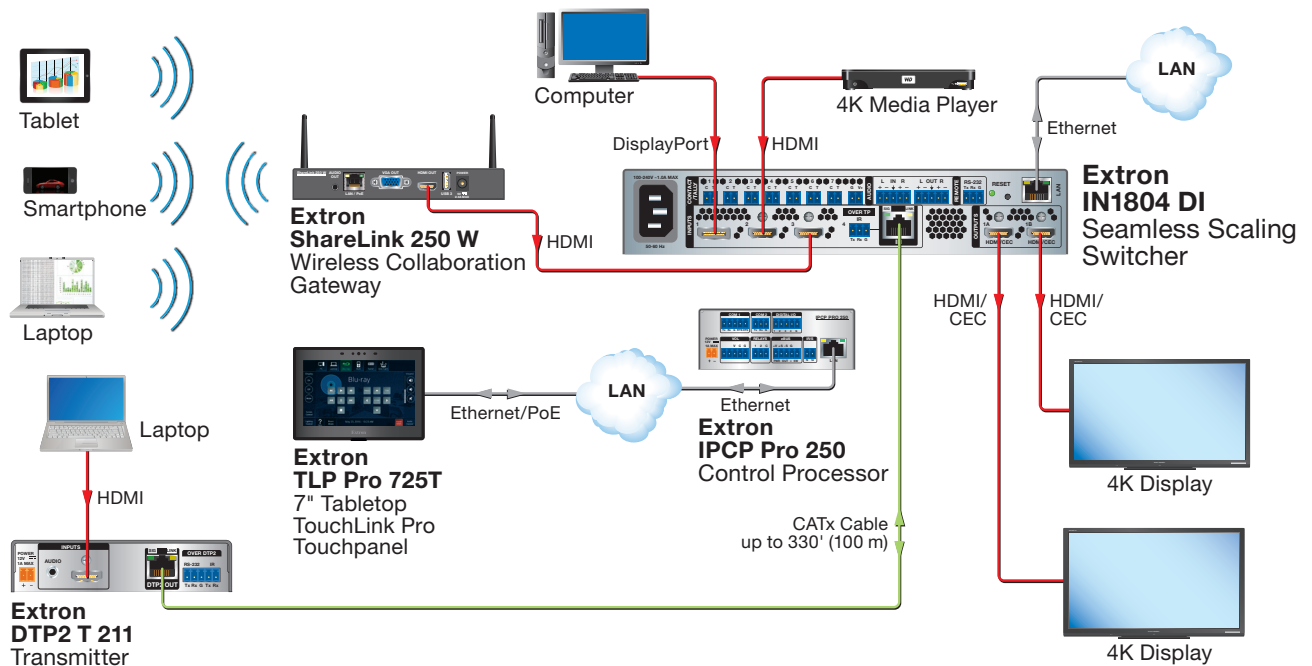
Figure 2. IN1804 DI Meeting Room Application Example
