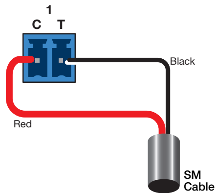
Figure 15. SM Cable Connecting Contact and Tally Ports
