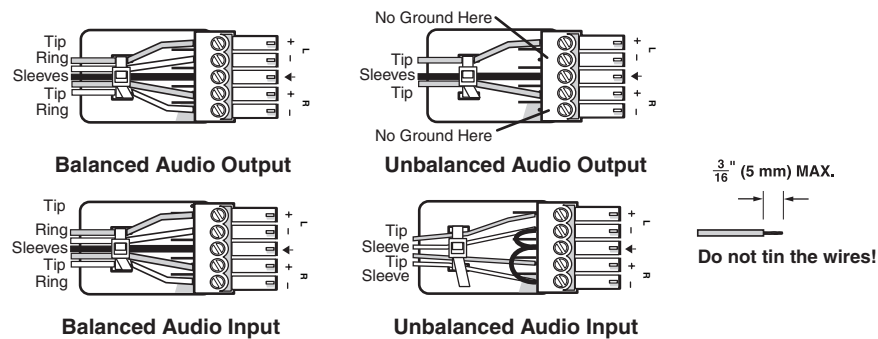
Figure 11. Analog Audio Wiring Configuration
