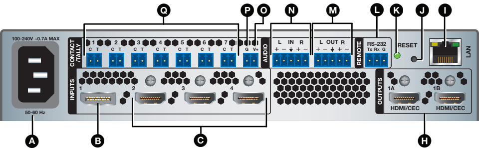
Figure 5. IN1804 Standard Rear Panel
