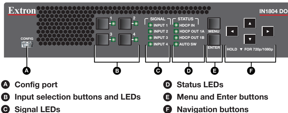
Figure 16. Front Panel Features (IN1804 DO Example)
