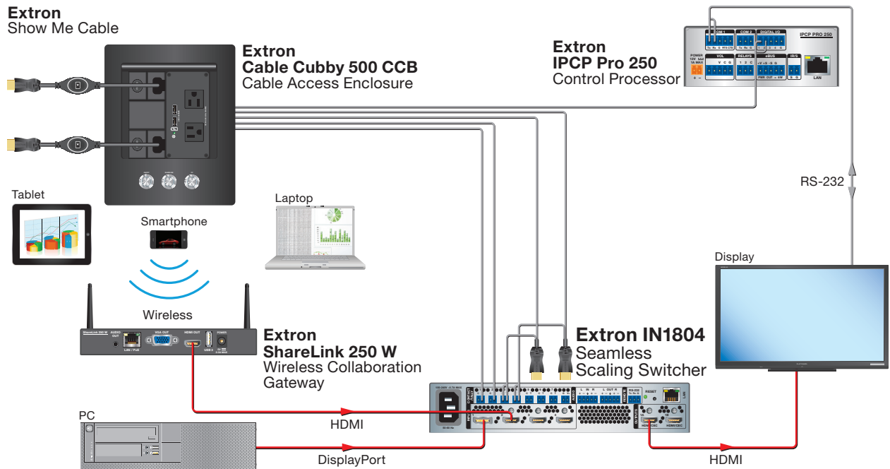
Figure 1. IN1804 Standard Model Application Example — Teamwork System
