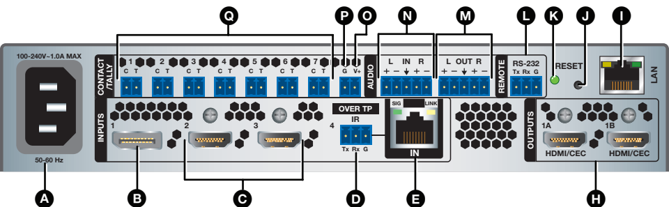
Figure 6. IN1804 DI Rear Panel
