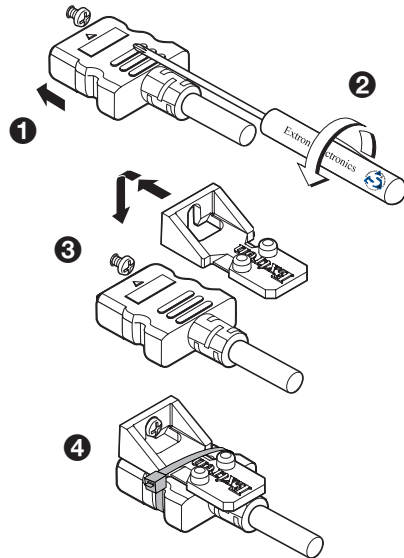
Figure 12. Mounting a LockIt Cable Lacing Bracket
