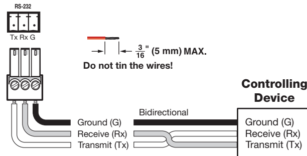
Figure 10. RS-232 Wiring
