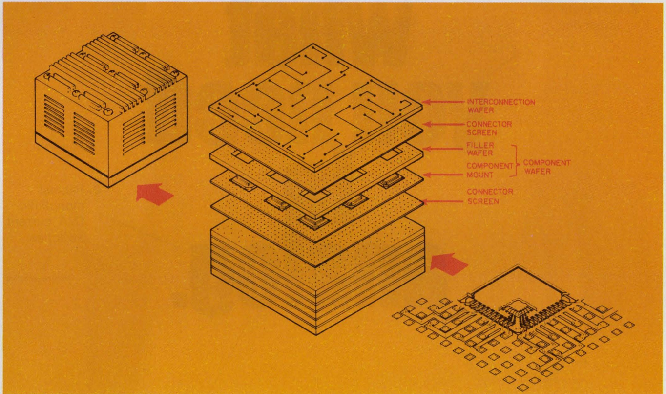
Bunker-Ramo's Planar Coax package has component wafers for holding devices like the 42-lead IC, lower
